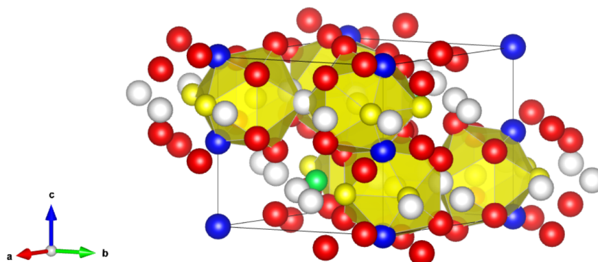
Figure 2: Coordination polyhedra of site 6h_2 of the \tau_{11} - \text{Al}_4\text{Fe}_{1.7}\text{Si} structure. Atoms and coordination polyhedron are represented in blue for site 2a , white for site 6h_1 , red for site 12k , green for site 2d and yellow for site 6h_2 .
