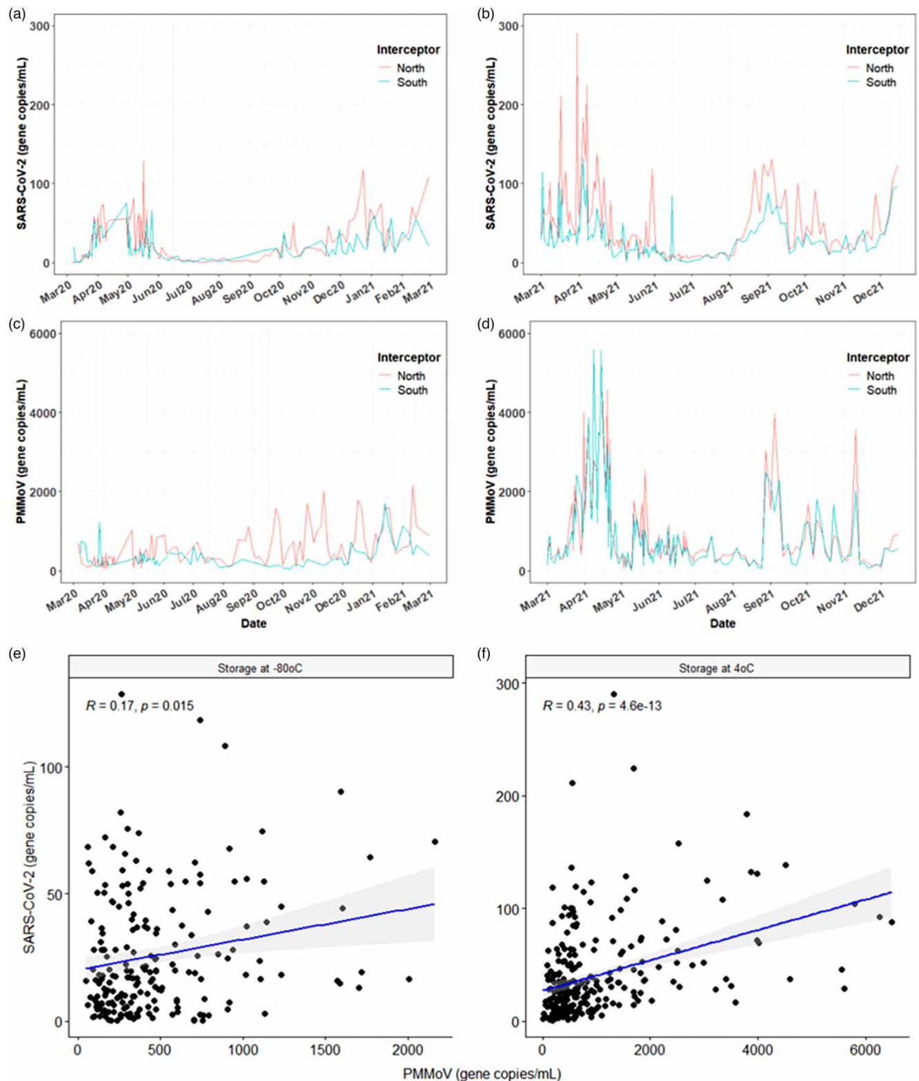
Figure 1 | Temporal series of SARS-CoV-2 (a and b) and PMMoV (c and d) concentrations in North and South interceptors from March 2020 to December 2021. Panels (a) and (c) show time series for samples stored at -80^{\circ}\text{C} before analysis. Panels (b) and (d) show samples stored at 4^{\circ}\text{C} . Panels (e) and (f) show the correlation of SARS-CoV-2 and PMMoV for samples stored at -80 and 4^{\circ}\text{C} .
