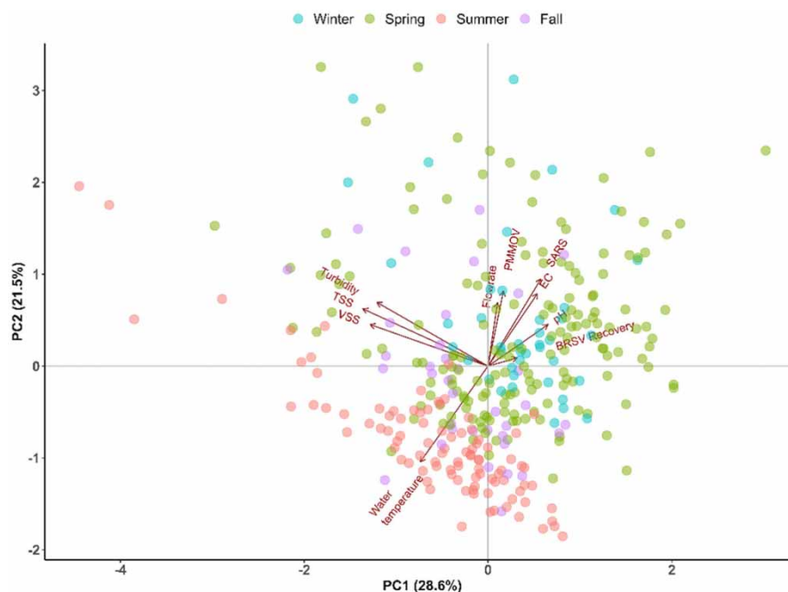
Figure 3 | PCA biplot of SARS-CoV-2, PMMoV, and wastewater parameters with a two-dimensional PCA biplot illustrating both the PC scores of samples (dots) and the loadings of variables (vectors). The dispersion of data points indicates the degree of correlation between the wastewater quality parameters and the virus's gene copies.
