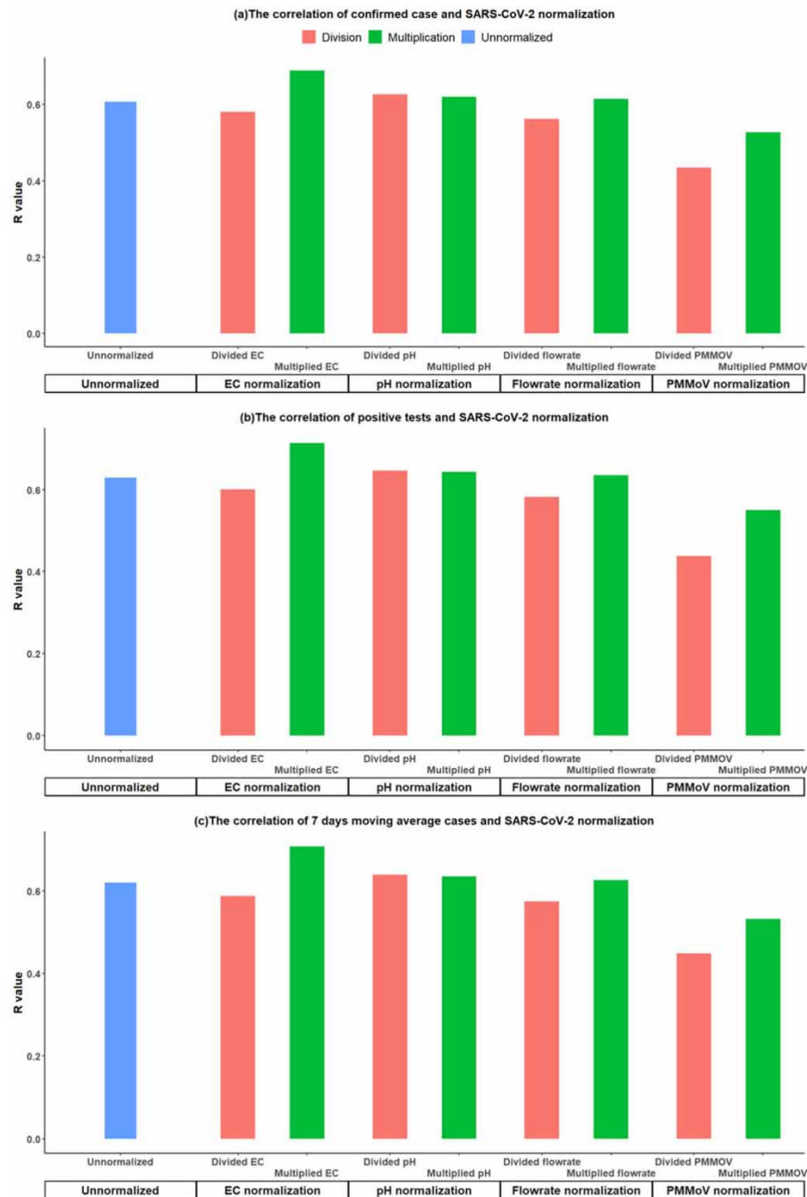
Figure 4 | The strength of association of unnormalized and normalized SARS-CoV-2 with different clinical data (the number of confirmed cases, positive tests, and moving average 7 days).
