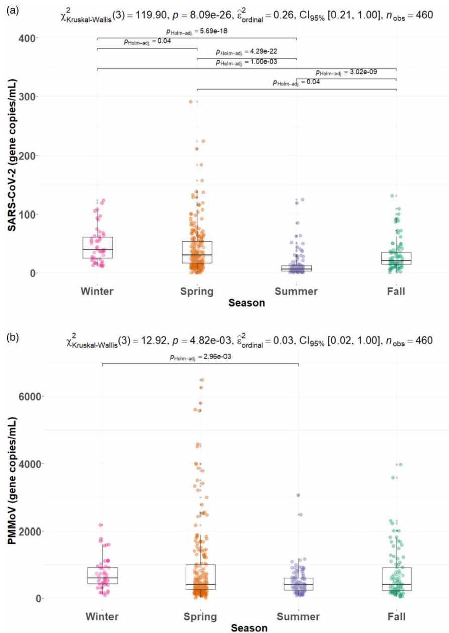
Figure 2 | The seasonal variation of SARS-CoV-2 and PMMoV in both sewer interceptors over a period of more than 1.5 years of monitoring.
