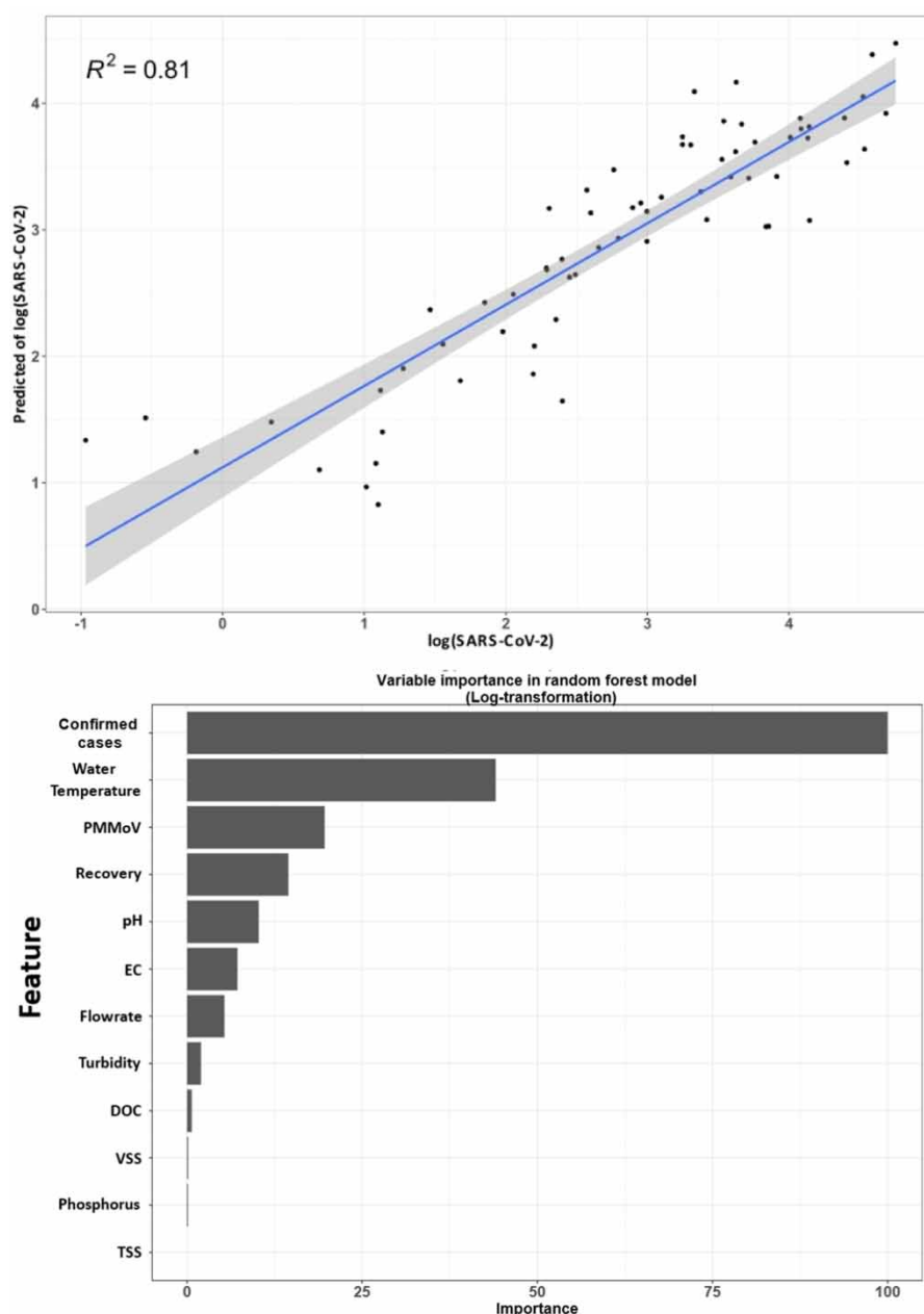
Figure 5 | Correlation of SARS-CoV-2 in wastewater and predicted SARS-CoV-2 using random forest with natural log-transformed SARS-CoV-2 data (top panel) and variable importance plot (bottom) for the random forest model. Training data = 272 observations and testing data = 67 from both storage conditions ( -80 and 4 °C).
