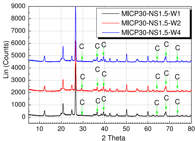
Fig. 18. X-Ray Diffraction of the sample modified by 30 % bacterial and cementation solutions and 1.5 % nano-SiO 2 after W1, W2 and W4 of curing time.
