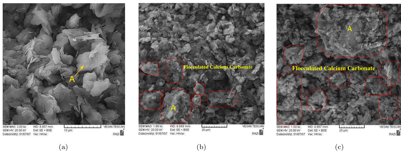
Fig. 19. SEM images of a) untreated sample, b) sample treated by MICP, c) sample treated by MICP+1.5 % nano-SiO 2 .
