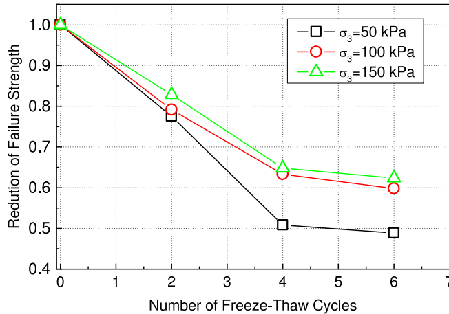
Fig. 12. Effect of FTCs on the degradation of failure strength at 50, 100 and 150 kPa confining pressure.
