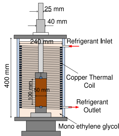
(b) Cross section of the cell and the thermal copper coil
