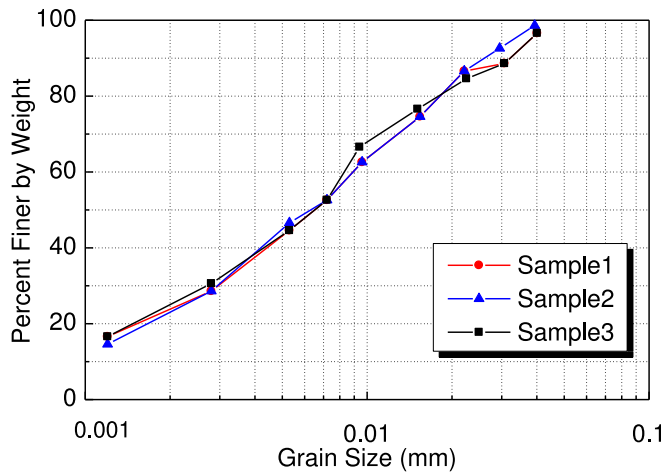
Fig. 1. Grain size distribution curves of the kaolinite samples.
