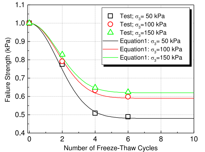
Fig. 14. Comparison of the experimental data and the curves obtained by Eq. 1.
