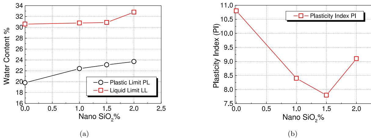
Fig. 10. Effect of nano-SiO 2 on the Atterberg limits and plasticity index of the kaolinite soil samples.
