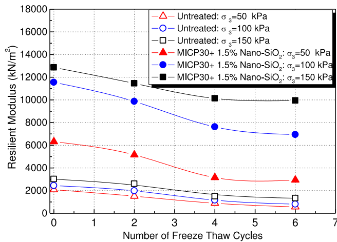
Fig. 15. Effect of FTCs on resilient modulus of non-modified and modified soil at different confining stresses.
