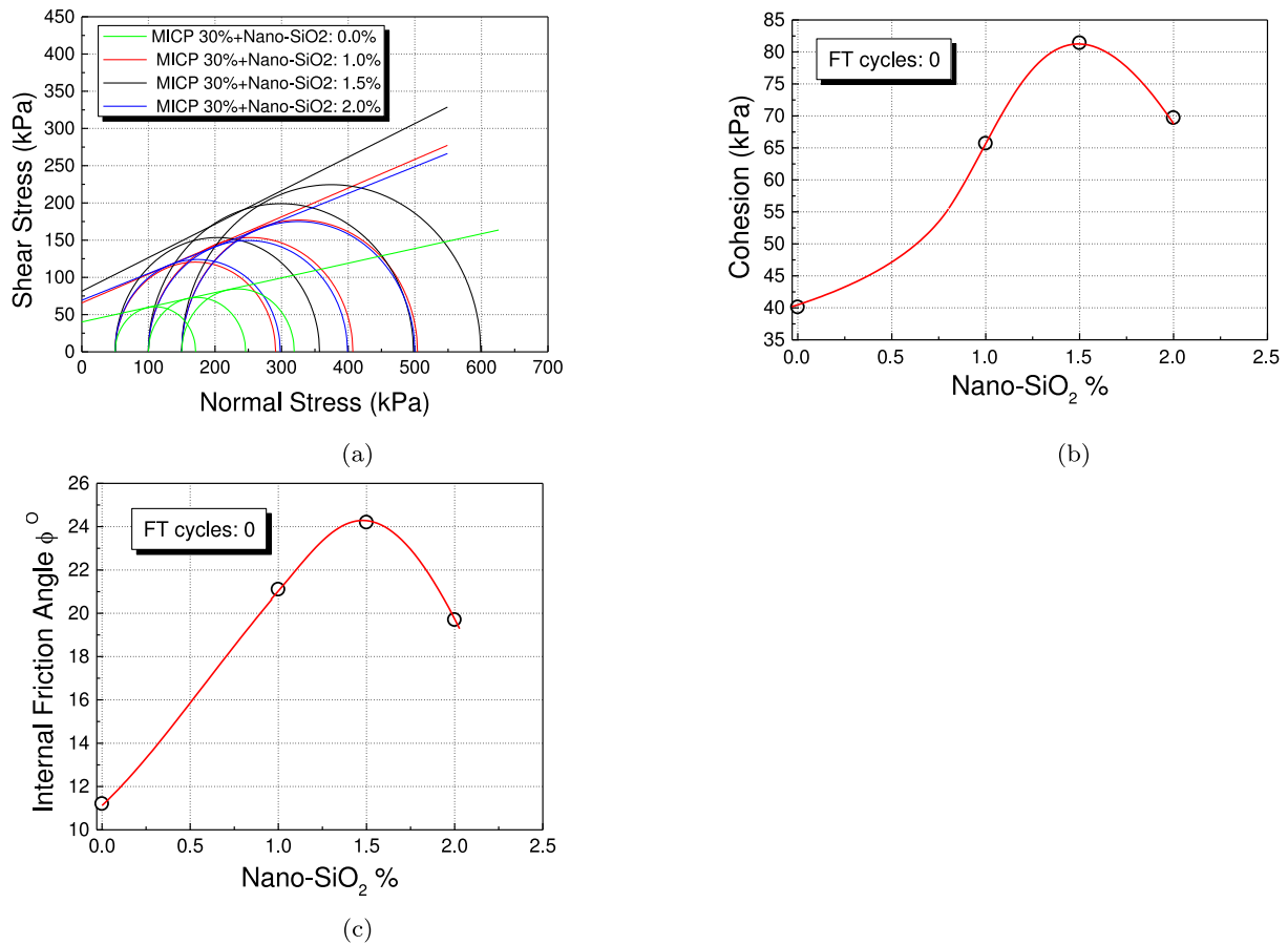
Fig. 9. Comparison of Mohr-Coulomb failure envelopes, and cohesion and friction angle of non-modified and 30 % MICP modified samples with 1, 1.5 and 2 % nano-SiO 2 .
