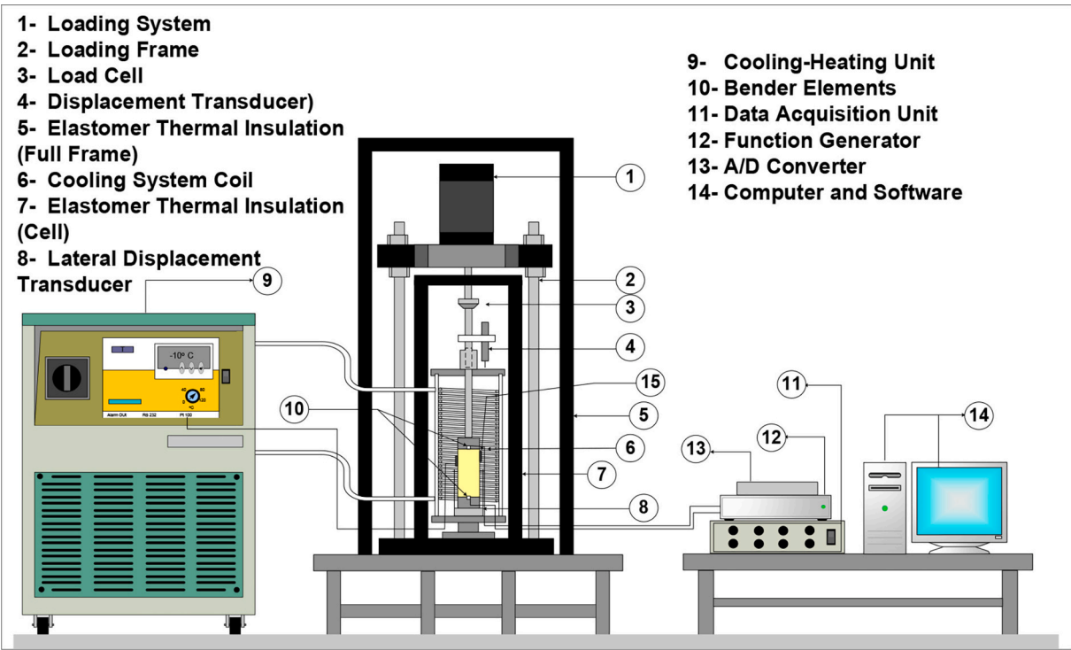
Fig. 4. General layout of F-T triaxial apparatus used in this study.
