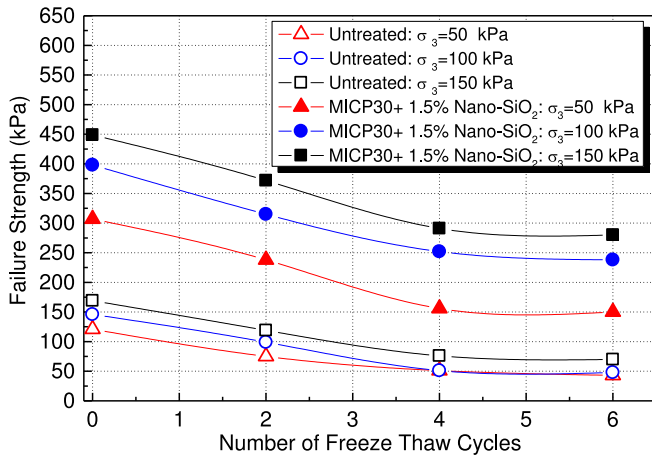
Fig. 11. Effect of FTCs on failure strength of untreated kaolinite treated by 30 % MICP and 1.5 % nano-SiO 2 under different confining stresses.
