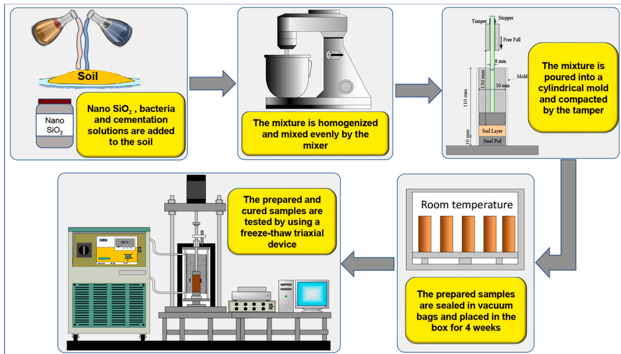
Fig. 3. Sample preparation process.
