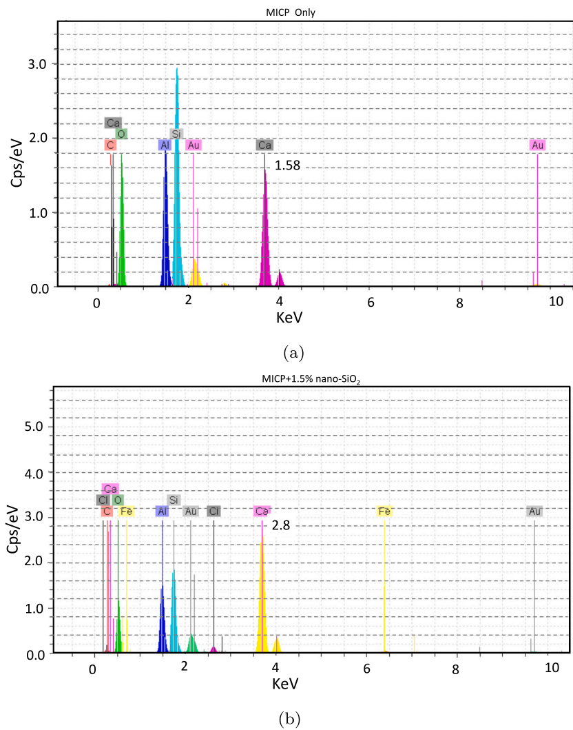
Fig. 20. a) Energy dispersive spectra (EDS) for agglomerated area A of the sample treated by MICP b) for agglomerated area A of the sample treated by MICP+1.5 % nano-SiO 2 .
