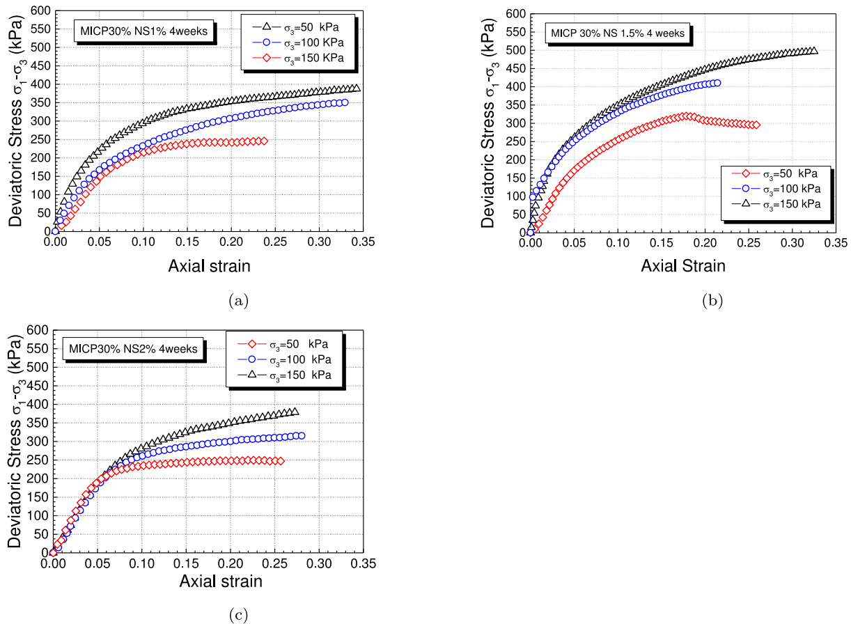
Fig. 8. Results of triaxial test on kaolinite samples treated with 30 % MICP mixed with 1.0 %, 1.5 % and 2 % nano-SiO 2 after 4 weeks curing time before applying FTCs.
