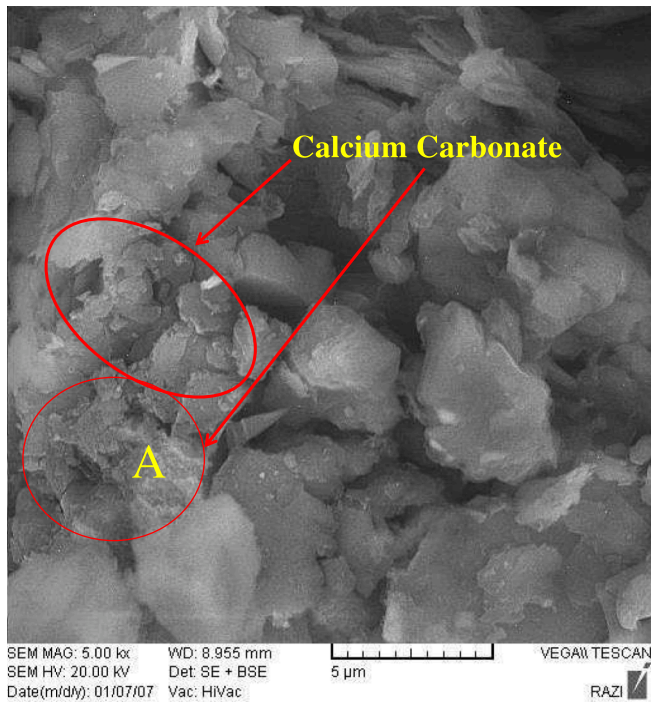
Fig. 17. Scanning Electron Microscope images of sample treated with 30 % MICP solutions and 1.5 % nano-SiO 2 ; clear difference between clay minerals and agglomerated part.
