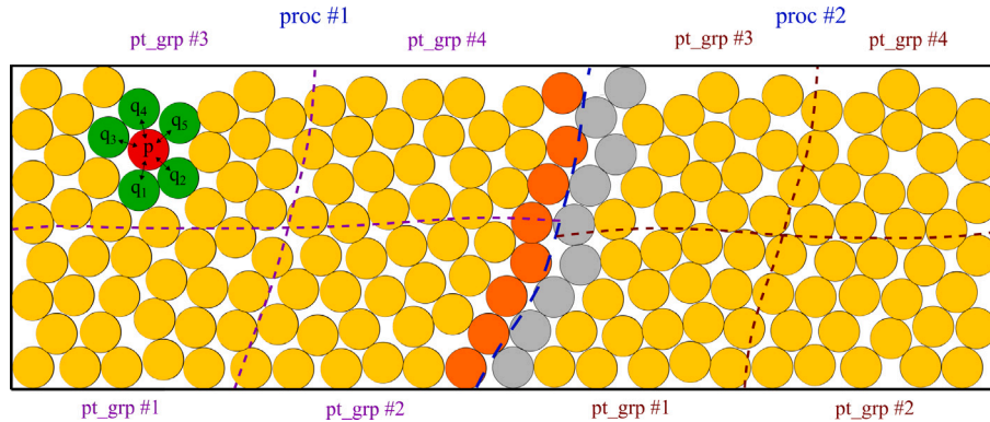
Fig. 2. Particle distribution in a computational domain. \text{—} \text{—} \text{—} : limit between processor domains. \text{-- --} : limit between particle groups (pt_grp). \bullet : ghost particles of processor #2. \odot : ghost particles of processor #1. A particle of interest, p , is in contact with 5 particles.
