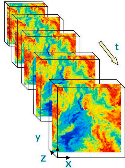
Fig. 4. Schematics of the problem domain [49–51] from https://turbulence.pha.jhu.edu .
