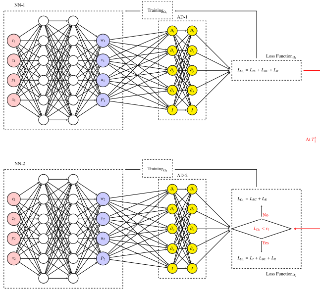
Fig. 3. Schematics of the DG-PINN. (For interpretation of the references to color in this figure legend, the reader is referred to the web version of this article.)
