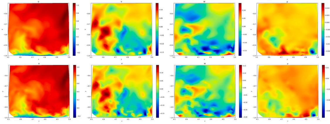
Fig. 11. Velocity and pressure fields at t_{13} = 13 \times 0.0065 . Top: DNS solutions; bottom: DG-PINN approximations.
