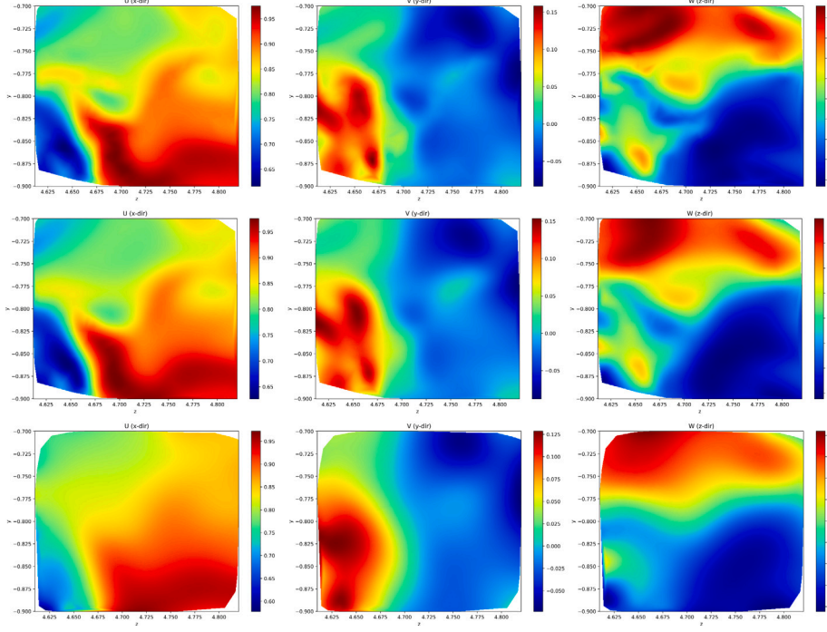
Fig. 6. Instantaneous velocity fields at t_{65} = 65 \times 0.0065 : From top to bottom: DNS solution, DG-PINN, and Baseline PINNs.
