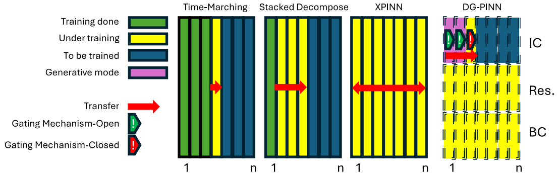
Fig. 1. Illustration of existing decomposition methods compared with the DG-PINN.
