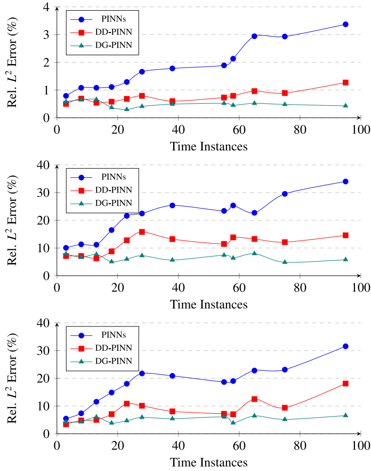
Fig. 8. Comparison of the error: Top: x direction, middle: y direction, and bottom: z direction.
