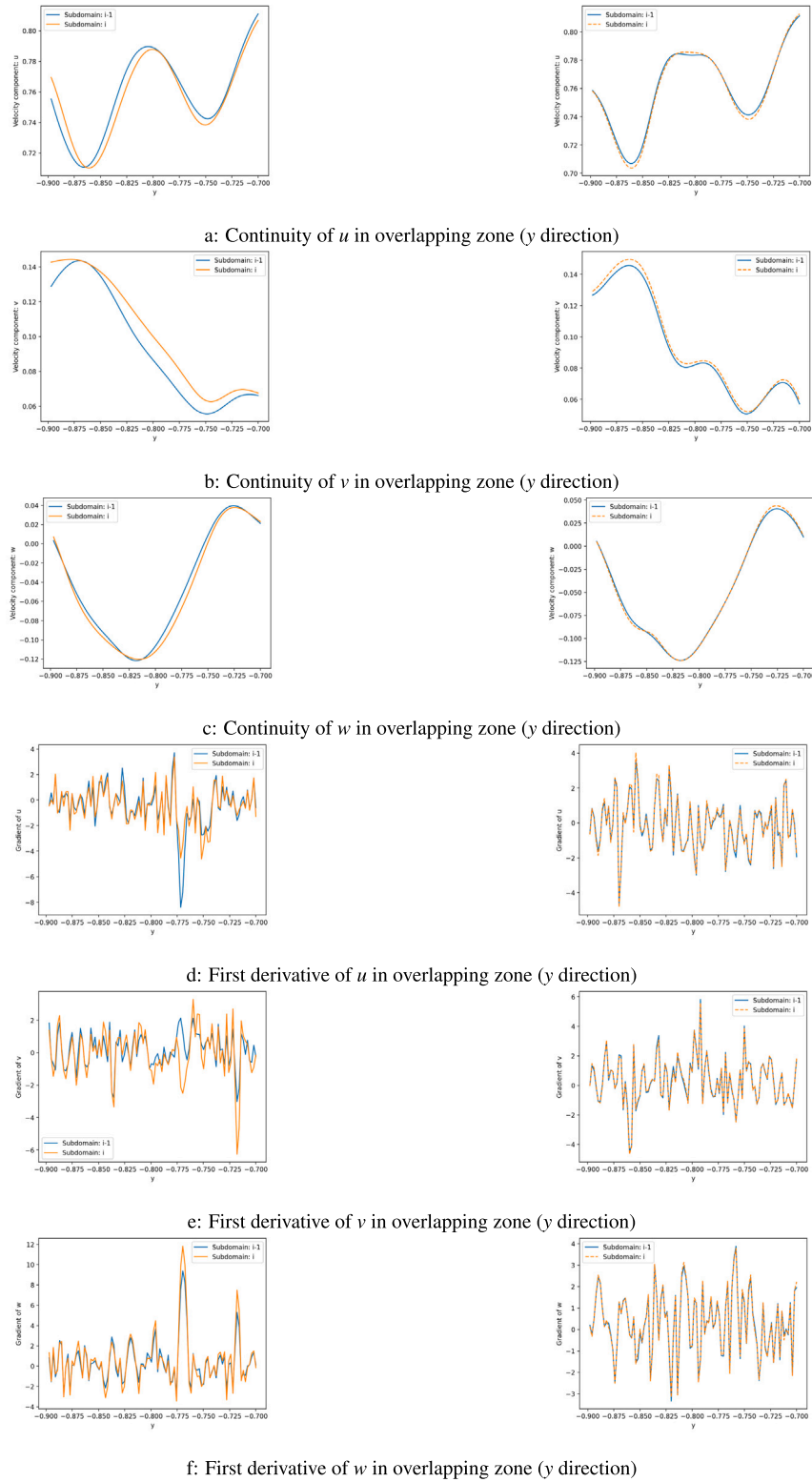
Fig. 12. Solution regularity analysis at 10th time step: DG-PINN using H^1 norm (right) vs. a counterpart model using L^2 norm resembling traditional decomposition methods (left).
