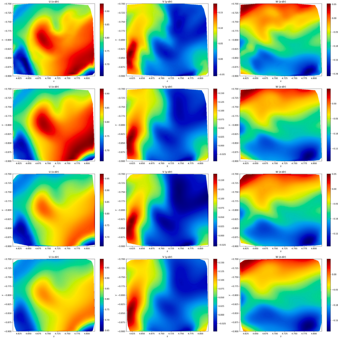
Fig. 5. Instantaneous velocity fields at t_8 = 8 \times 0.0065 : From top to bottom: DNS solution, DG-PINN, DD-PINN, and Baseline PINNs.
