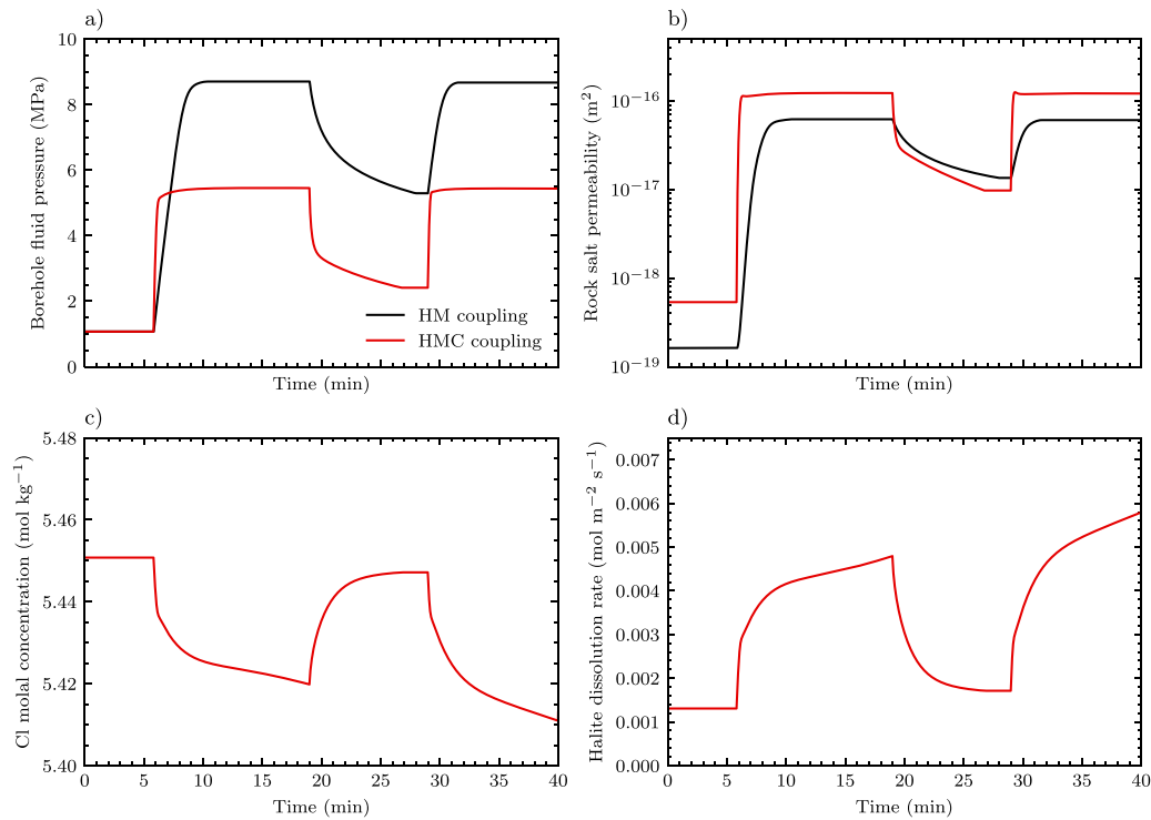
Fig. 9. Comparison of fluid pressure (a) and permeability (b) between the HM and HMC models, and the corresponding \text{Cl}^- concentration (c) and halite dissolution rate (d).
