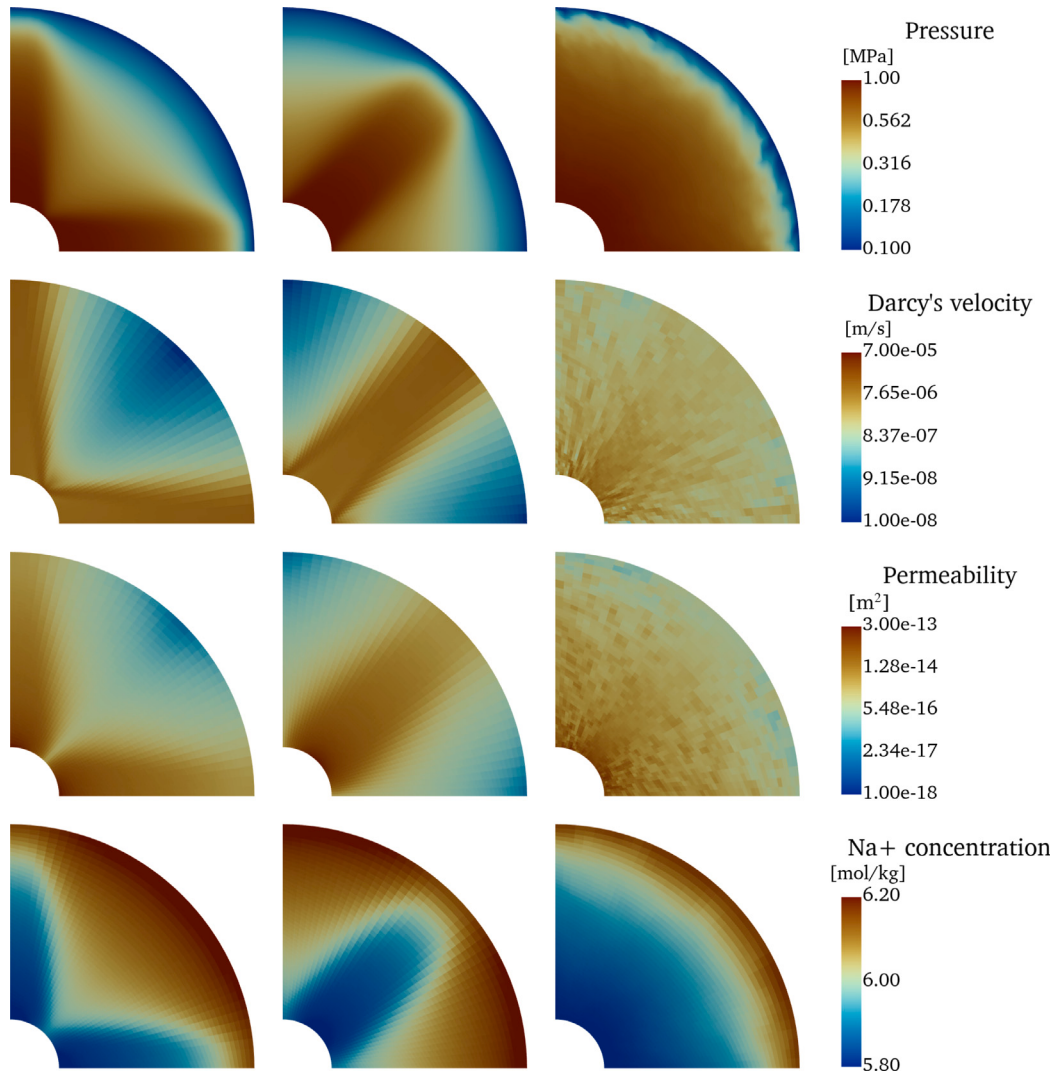
Fig. 5. Fluid pressure, Darcy's velocity, permeability, and \text{Na}^+ concentration fields for HMC coupling (with halite dissolution) shown from left to right for (left) the embedded orthotropic fracture model aligned in both vertical and horizontal directions, (center) the embedded orthotropic fracture model rotated by 45^\circ , and (right) the embedded orthotropic fracture model of randomly-distributed fracture normal.
