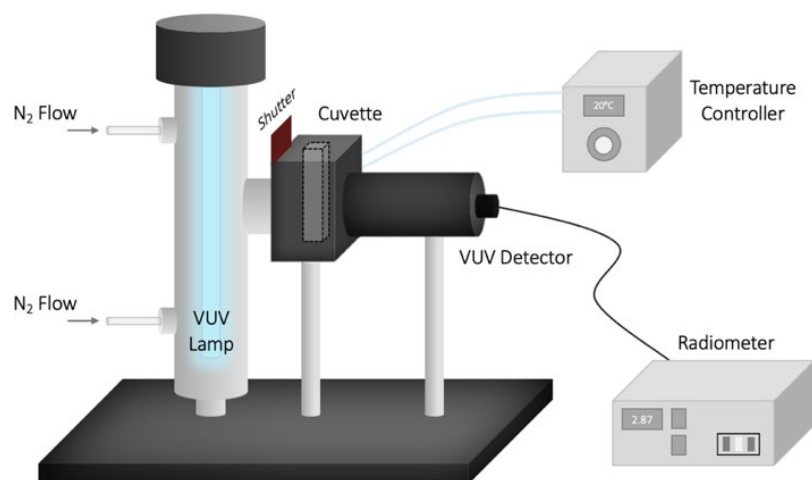
Figure S2. VUV 185 nm radiometry setup.
