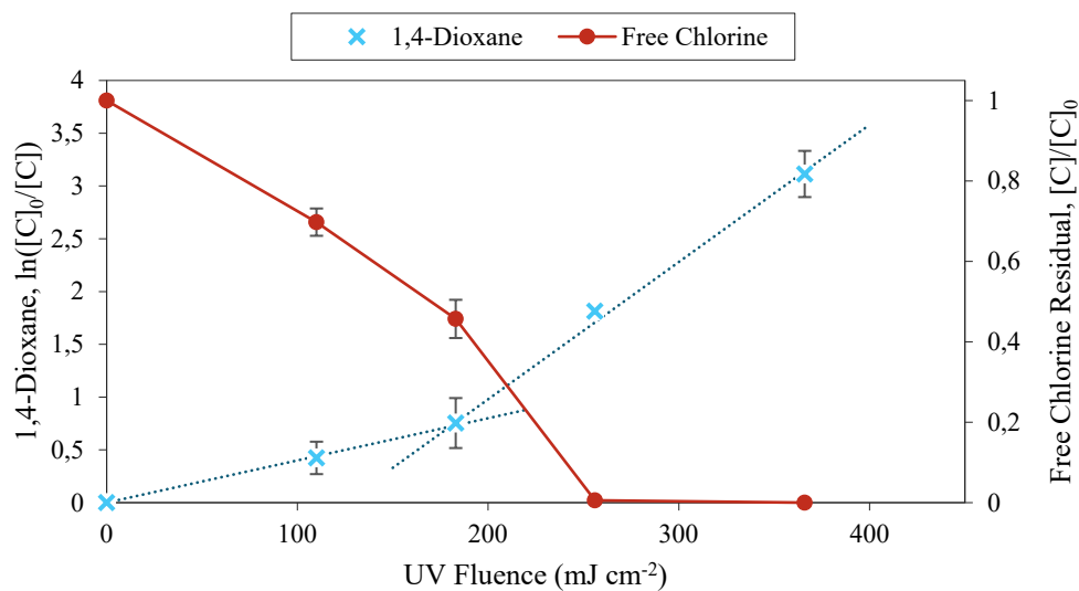
Figure S3. Enhancement of 1,4-D removal with consumption of free chlorine in the VUV/UV/Cl AOP in DI water ( [C]_{1,4-D,0} = 6 \mu\text{M} , [C]_{\text{free chlorine},0} = 70 \mu\text{M} , Average pH = 6.5 (unadjusted)). Dotted lines indicate the trend lines for 1,4-D removal before and after chlorine depletion in the solution.
