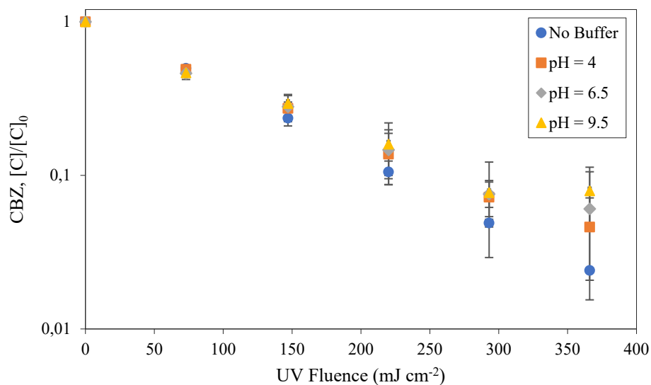
Figure S4. Degradation of CBZ in the VUV/UV AOP at different pH levels ( [C]_{\text{CBZ},0} = 1 \text{ ppm} , [C]_{\text{phosphate buffer}} = 2 \text{ mM} ).
