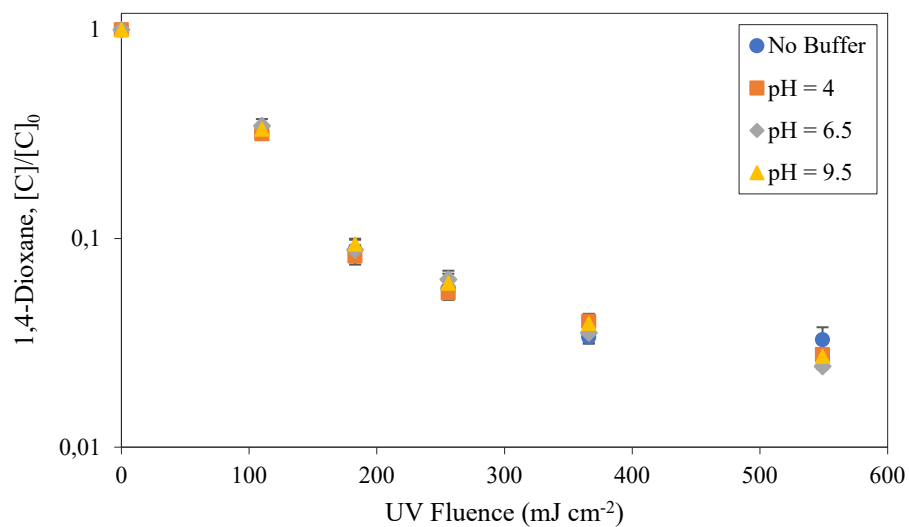
Figure S5. Degradation of 1,4-D in the VUV/UV AOP at different pH levels ( [C]_{1,4-D,0} = 0.5 ppm, [C]_{\text{phosphate buffer}} = 2 mM).
