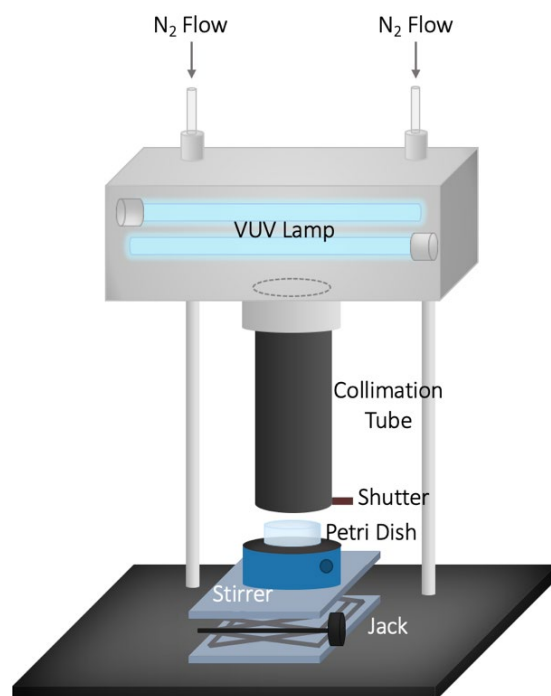
Figure S1. VUV/UV collimated beam setup.
