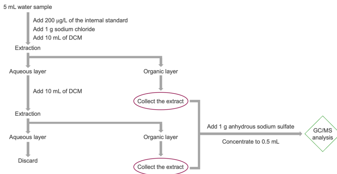
Figure S7. The flowchart of 1,4-dioxane sample preparation overview.
