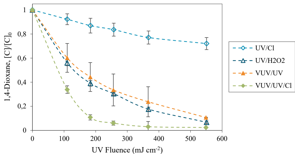
Figure S6. Degradation kinetics of 1,4-D in the VUV/UV and VUV/UV/Cl AOPs compared to the commonly used UV/Cl and UV/H 2 O 2 treatments in RO permeate water matrix ( [C]_{1,4-D,0} = 6 \mu M, [C]_{\text{free chlorine},0} = 70 \mu M, [C]_{\text{H}_2\text{O}_2,0} = 88 \mu M).
