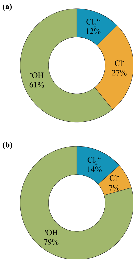
Fig. 5. Contribution of ^{\bullet}\text{OH} , \text{Cl}^{\bullet} , and \text{Cl}_2^{\bullet-} to the degradation of (a) CBZ and (b) 1,4-D in the VUV/UV/ \text{Cl}_2 AOP in DI water ( [\text{C}]_{\text{CBZ},0} = 4 \text{ }\mu\text{M} , [\text{C}]_{1,4\text{-D},0} = 6 \text{ }\mu\text{M} , [\text{C}]_{\text{free chlorine},0} = 70 \text{ }\mu\text{M} , [\text{C}]_{\text{t-BuOH}} = 0.4 \text{ mM} , [\text{C}]_{\text{NB}} = 40 \text{ }\mu\text{M} , Average pH = 6.5 (unadjusted)).
