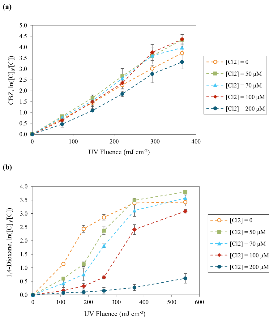
Fig. 3. Effect of free chlorine dose on the VUV/UV AOP for degradation of (a) CBZ, and (b) 1,4-D in DI water ( [\text{C}]_{\text{CBZ},0} = 4 \mu\text{M} , [\text{C}]_{1,4\text{-D},0} = 6 \mu\text{M} , Average pH = 6.5 (unadjusted)). Error bars represent the standard deviations of three experimental replicates.
