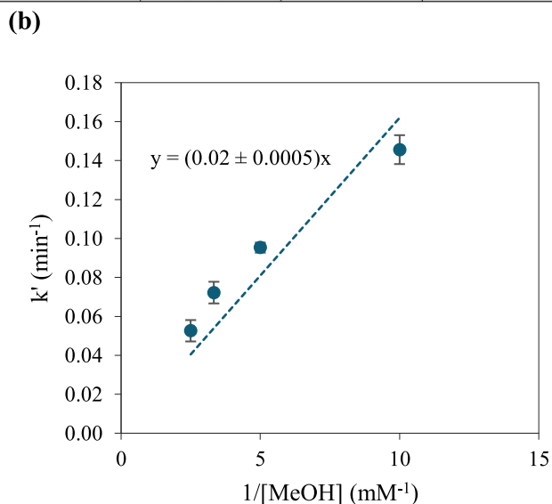
Fig. 1. (a) Experimental measurement of the pseudo-first order photo-degradation rate constant of CBZ at different concentrations of MeOH ( [C]_{CBZ,0} = 0.85 \mu\text{M} ); (b) Estimation of the incident fluence rate at 185 nm based on the experimental results of CBZ degradation in presence of MeOH. Error bars represent the standard deviations of three experimental replicates.
