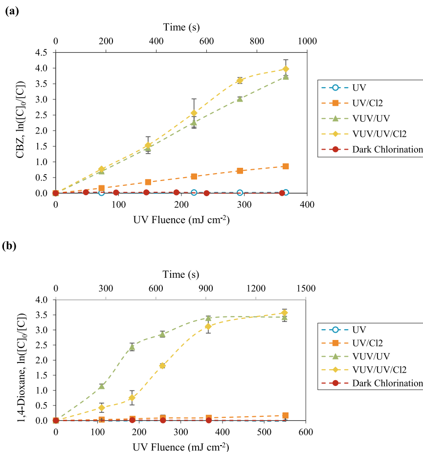
Fig. 2. Degradation of (a) CBZ and (b) 1,4-D under different AOP conditions in DI water ( [C]_{\text{CBZ},0} = 4 \mu\text{M} , [C]_{1,4\text{-D},0} = 6 \mu\text{M} , [C]_{\text{free chlorine},0} = 70 \mu\text{M} , Average pH = 6.5 (unadjusted)). Error bars represent the standard deviations of three experimental replicates.
