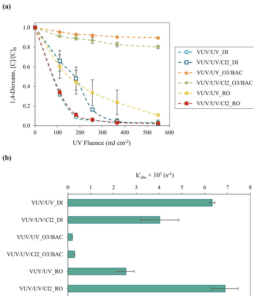
Fig. 6. (a) Degradation kinetics of 1,4-D in the VUV/UV and VUV/UV/Cl 2 AOPs obtained in water samples from potable reuse trains as compared to DI water and (b) Comparison of the pseudo-first order rate constants for 1,4-D degradation in the VUV/UV and VUV/UV/Cl 2 AOPs in different water matrices ( [C]_{1,4-D,0} = 6 \mu\text{M} , [C]_{\text{free chlorine},0} = 70 \mu\text{M} ). Error bars represent the standard deviations of three and two experimental replicates for DI water and the investigated water samples, respectively.
