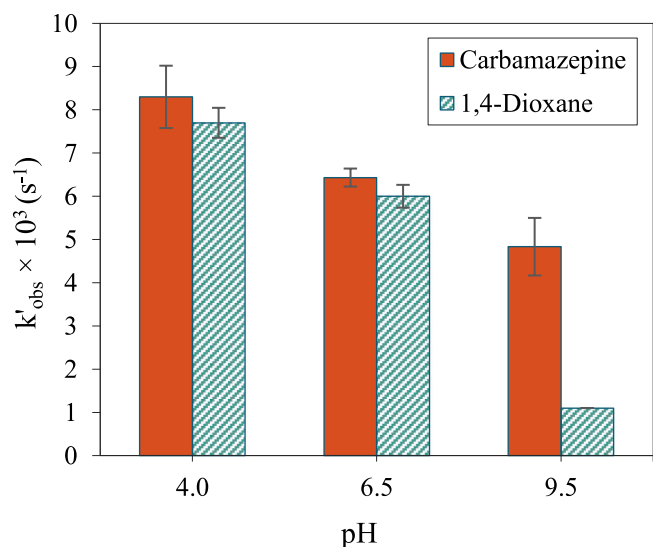
Fig. 4. Observed pseudo-first order rate constants for the degradation of CBZ and 1,4-D in the VUV/UV/ \text{Cl}_2 AOP in DI water as a function of pH ( [\text{C}]_{\text{CBZ},0} = 4 \mu\text{M} , [\text{C}]_{1,4\text{-D},0} = 6 \mu\text{M} , [\text{C}]_{\text{free chlorine},0} = 70 \mu\text{M} , [\text{C}]_{\text{phosphate buffer}} = 2 \text{ mM} ). Error bars represent the standard deviations of three experimental replicates.
