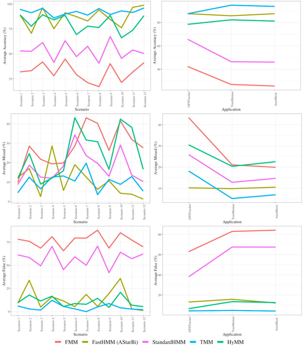
Fig. 4. Plots of average accuracy, average missed links, and average false links for each algorithm by scenario and application
