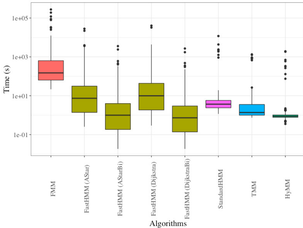
Fig. 6. Box plot of matching run time per 1000 observations by algorithm (on a logarithm scale)
