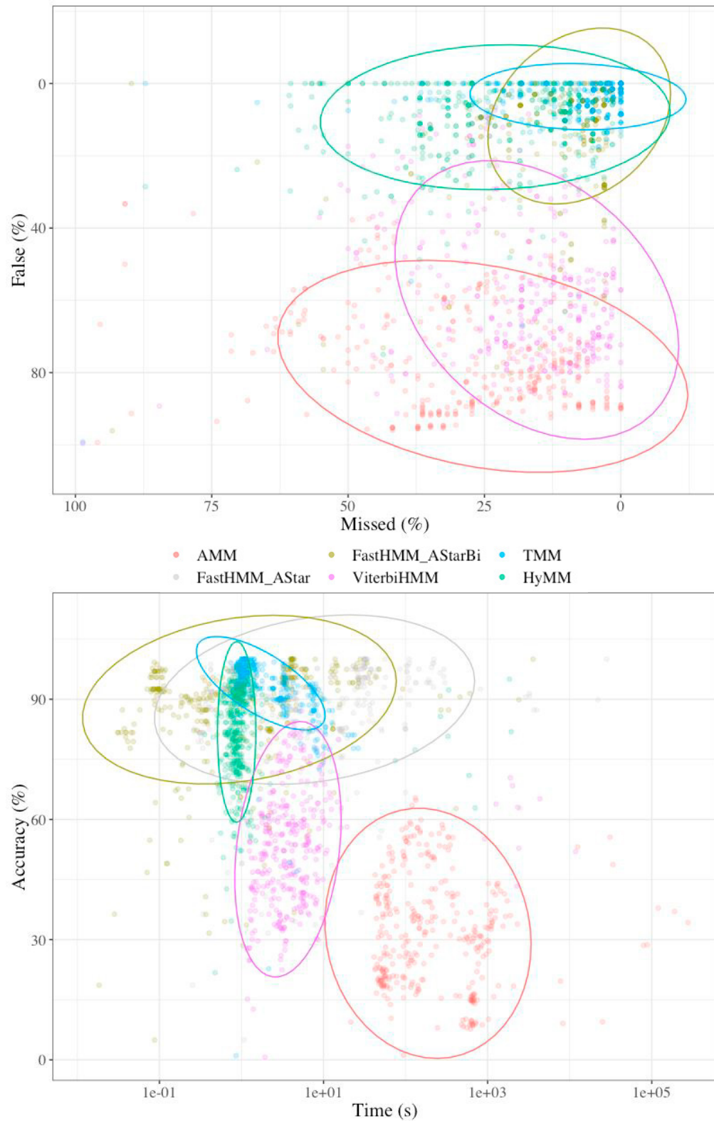
Fig. 7. % missed vs. % false (top) and accuracy vs. run time (bottom) with dispersion ellipses for all considered algorithms
