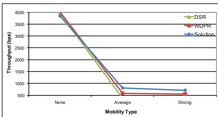
Figure 3.6 Overall throughput as a function of the nodes mobility (60 mobile nodes and no attackers)
