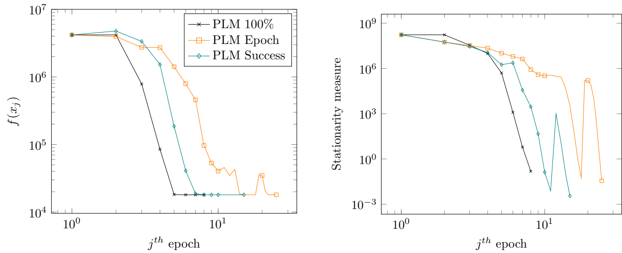
Figure 3.8 PLM methods on Bundle Adjustment Dubrovnik problem.
