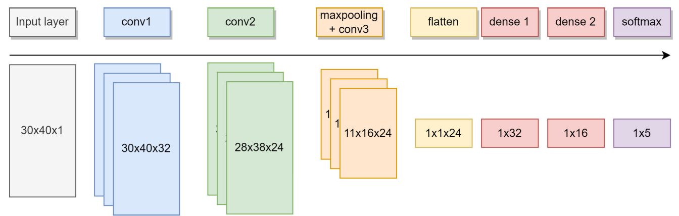
FIGURE 7. Face recognition model used for testing [65].
