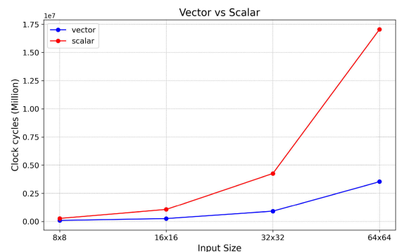
FIGURE 6. Comparison of vector and scalar computational in millions of clock cycles for different input sizes.
