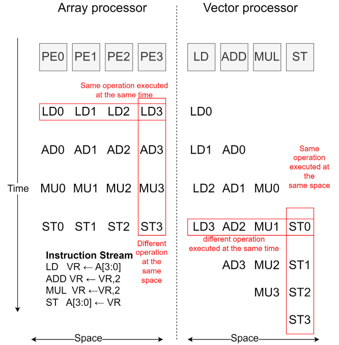
FIGURE 3. Comparison of scalar or array processor with vector processor: the former necessitates full data loading before execution initiation, whereas the latter facilitates execution on the vector in parallel with data loading, reducing execution delays.
