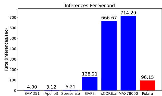
FIGURE 8. Number of inferences per second.
