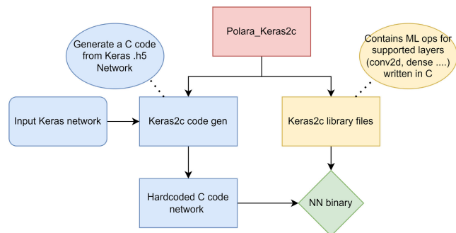
FIGURE 4. Polara-Keras2c system diagram: The code has two parts: a Python code that generates the C code with the layers used, tensor sizes, and library files in C that contain the executable code for supported layers.
