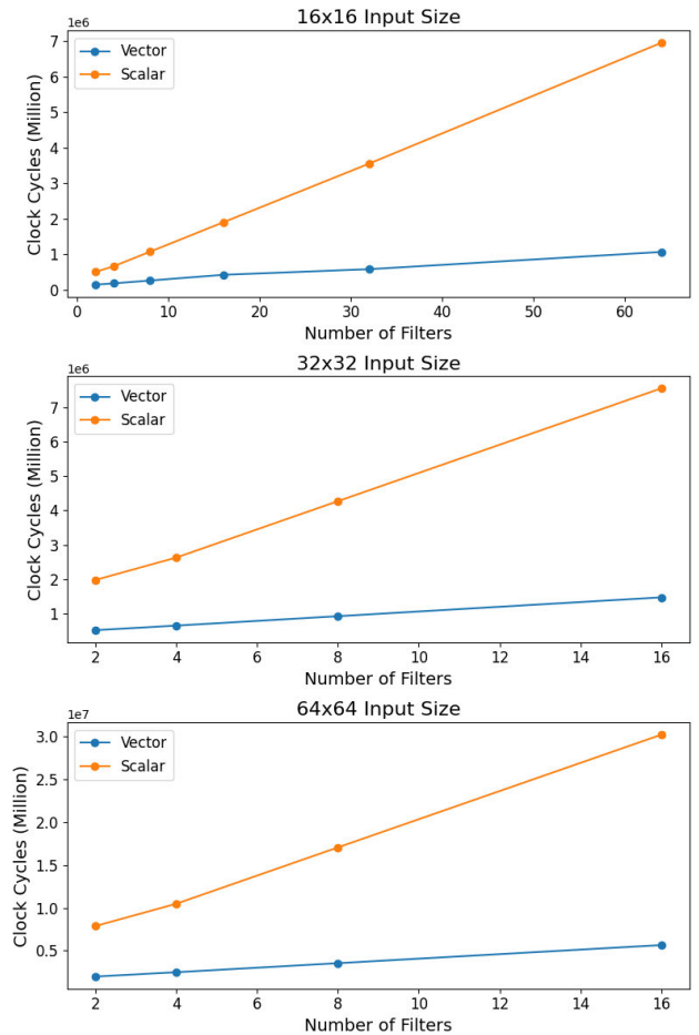
FIGURE 5. Clock cycles in millions versus the number of filters for different input sizes.
