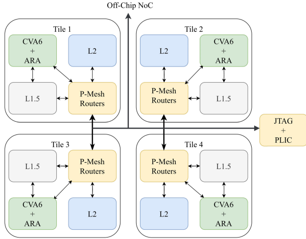
FIGURE 2. System Architecture Overview. The architecture comprises four interconnected tiles, each containing a CVA6 + ARA processing core, L1.5 cache, L2 cache, and P-Mesh routers for inter-tile communication. Tiles are linked to an off-chip Network-on-Chip (NoC) and JTAG + PLIC for debugging and interrupt handling, respectively. The P-Mesh routers manage data traffic within and between tiles, providing scalable, low-latency communication.
