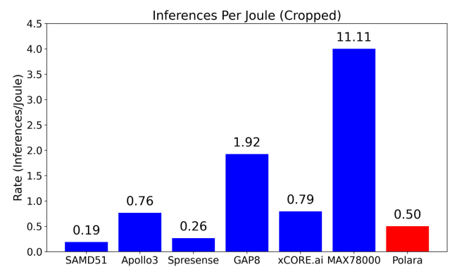
FIGURE 9. Number of inferences per Joule.
