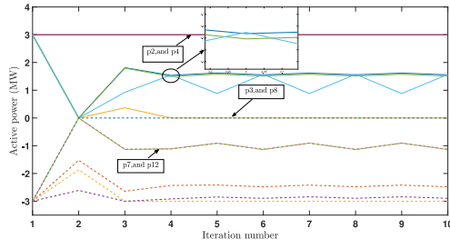
(a) Equilibrium of P2P trade in Scenario 6.
