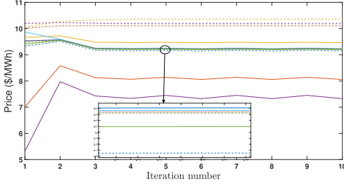
(c) DSO's pricing strategy in Scenario 6.
