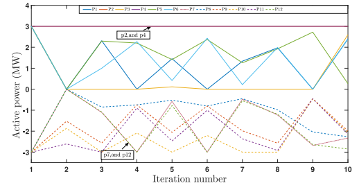
(b) Equilibrium of P2P trade in Scenario 7.
