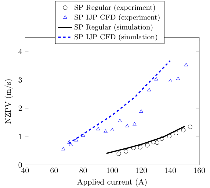
Figure 10. Measured NZPV values vs. the applied current for a SP regular sample (black circles) and a SP IJP CFD sample (blue triangles). The solid black line corresponds to the simulated NZPV for a SP regular sample, while the dashed blue line is the simulated NZPV for a SP IJP CFD sample for R_i^* = 35 \mu\Omega.cm^2 .
