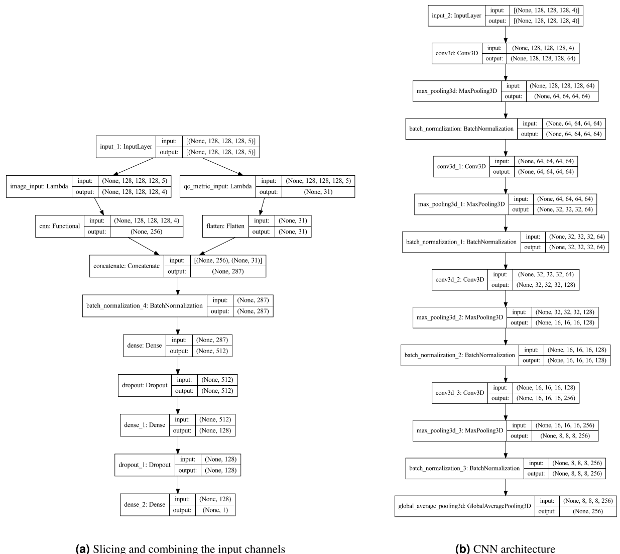
Fig. 5 Deep learning model architecture: (a) The CNN-i + q model accepts multichannel input that combined four imaging channels with a fifth channel containing 31 QSIprep automated data quality metrics. The imaging channels are separated from the data quality channel using Lambda layers. The imaging channels are passed through a CNN (b) , the output of which is concatenated with the data quality metrics, batch normalized and passed through two fully-connected (FC) layers, with rectified linear unit (ReLU) activation functions and with 512 and 128 units respectively. Each FC layer is followed by a dropout layer which drops 40% of the input units. The final layer contains a single unit with a sigmoid activation function and outputs the probability of passing QC. (b) The CNN portion of the model passes the imaging input through four convolutional blocks. Each block consists of a 3D convolutional layer with a kernel size of 3 and a ReLU activation, a 3D max pooling layer with a pool size of 2, and a batch normalization layer with Tensorflow's default parameters. The number of filters in the convolutional layers in each block are 64, 64, 128, and 256 respectively. The output of the final block is passed through a 3D global average pooling layer with Tensorflow's default parameters.
