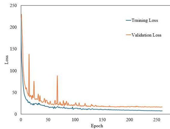
Figure A3. Representative CD training and validation loss curves.
