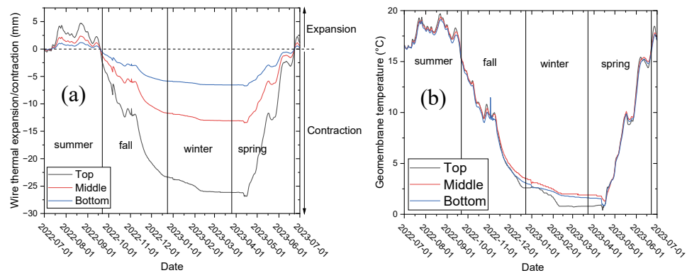
Fig. 8. Wire thermal expansion/contraction (a) and the temperature at the geomembrane level (b) from July 2022 to July 2023.
