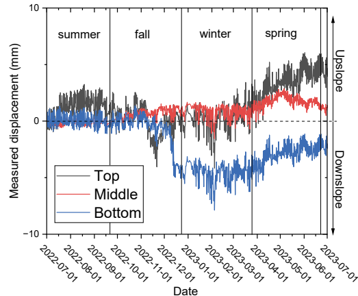
Fig. 7. Measured displacement from July 2022 to July 2023.
