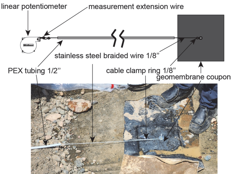
Fig. 3. Components of the geomembrane displacement measurement system.
