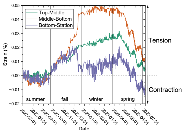
Fig. 10. Calculated strains between paired coupons, and the bottom coupon/measurement box.
