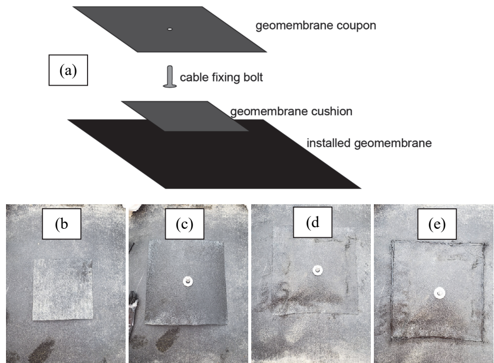
Fig. 4. Components of the geomembrane coupon (a) followed by the different steps of the installation: (b) GMB cushion installation, (c) GMB coupon installation, (d) thermal fusion, and (e) extrusion fillet.
