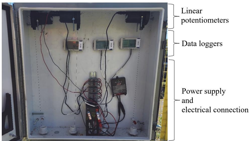
Fig. 5. Photograph of the components inside the monitoring station.
