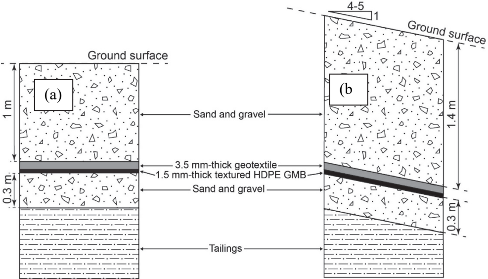
Fig. 1. Cross sections of the multilayered cover system built at the Aldermac mine site on the flat top section (a) and on the slopes (b).
