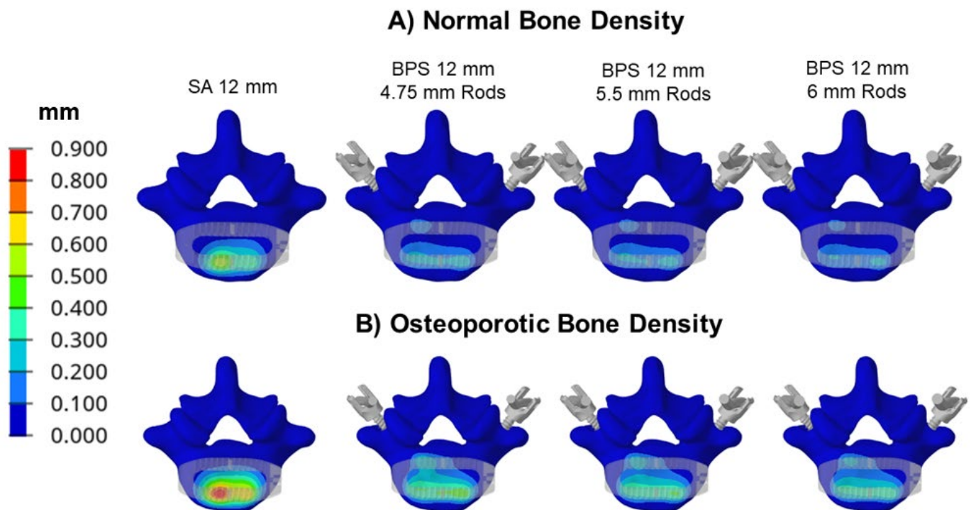
Figure S3 Maximum compression displacements (in mm) on L5 Cortical Endplate for A) normal and B) osteoporotic bone densities under functional load (400 N compression and 10 Nm flexion) with 12-mm cages.
