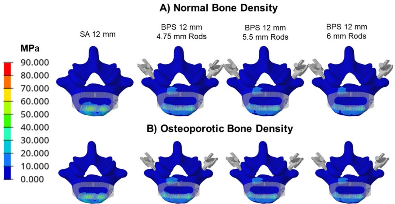
Figure S2 Maximum Von-Mises Stress (in MPa) on L5 Cortical Endplate for A) normal and B) osteoporotic bone densities under functional load (400 N compression and 10 Nm flexion) with 12-mm cages.
