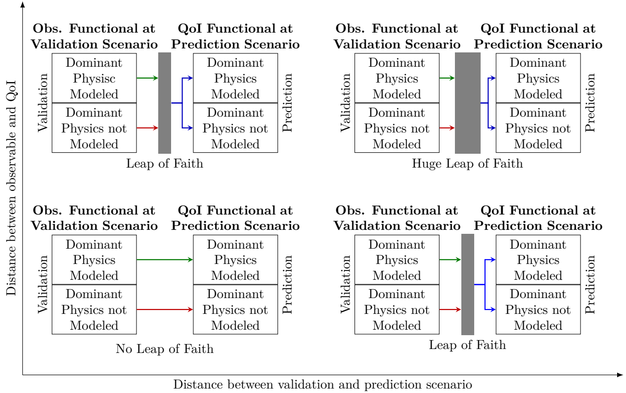
Figure 1.1 Extrapolation of the validation process from the observable to the QoI. The x-axis represent a "distance" between the validation and prediction scenario. The y-axis represent a "distance" between the observable functional and the QoI functional.
