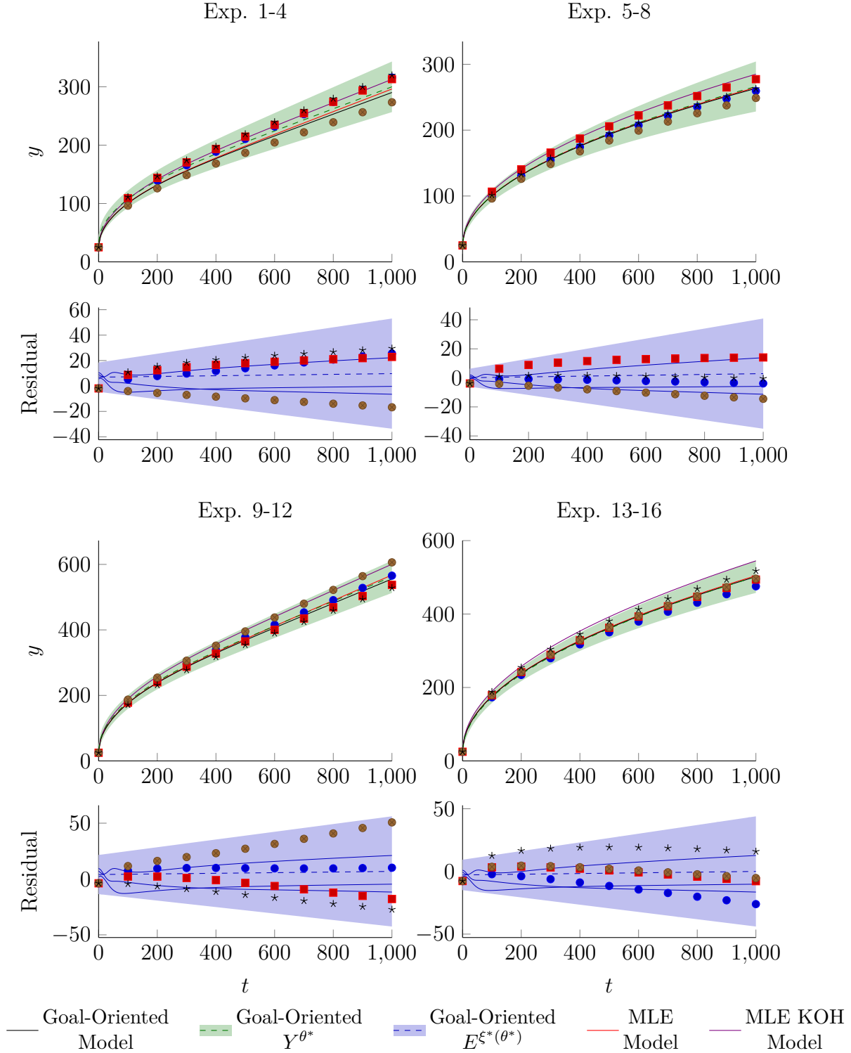
Figure 4.11 Optimal model predictions and associated modeling discrepancy at the four calibration scenarios. The first and third rows show the predictions obtained with the various calibration methods. The second and fourth rows depict the modeling discrepancies and residuals obtained with the second objective of the goal-oriented calibration. Some realizations of the modeling discrepancies E^{\xi^*(\theta^*)} are also demonstrated by thin curves.
