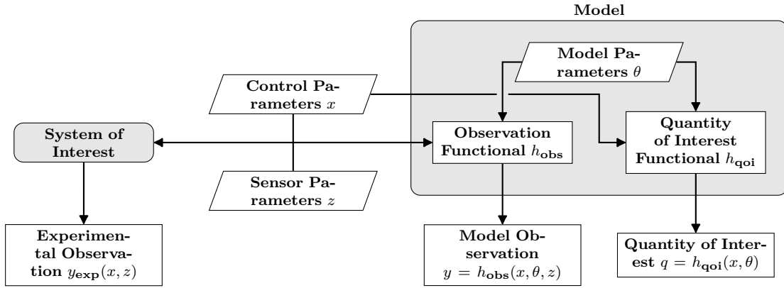
Figure 3.2 Diagram of the interactions between the various parameters and the system of interest as well as the model. It is important to observe that the model parameters \theta do not affect the system of interest, but only the observation and QoI functional h_{\text{obs}} and h_{\text{qoi}} . For the sake of simplicity, the QoI functional h_{\text{qoi}} does not depend explicitly on the sensor parameters z .
