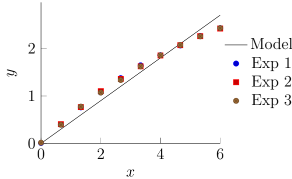
Figure 4.3 Experimental data and model prediction for \theta = 0.45 .
