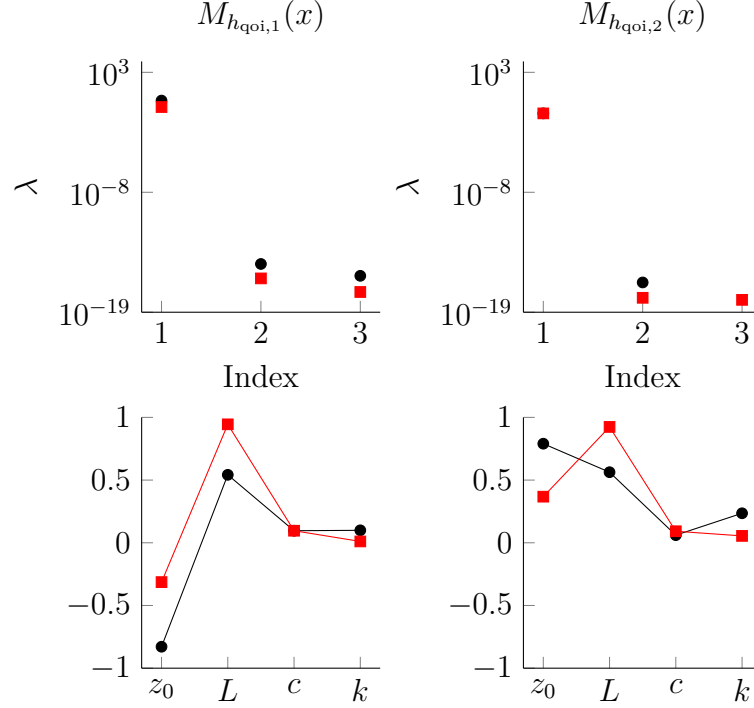
Figure 3.8 Eigenvalues (top row) and eigenvectors (bottom row) associated with the influence matrices for the prediction scenario (black circles) and for the validation scenario (red squares). The left and right columns display the sensitivity indices related to the first and second QoIs, respectively. For the sake of clarity, only the first (and only relevant) eigenvector is displayed for each influence matrix.
