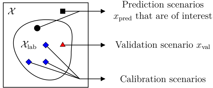
Figure 3.1 Illustration of the various scenarios. The prediction scenario may be producible (black circle) or may not be producible experimentally (black square). The validation and calibration scenarios are elements of the set \mathcal{X}_{\text{lab}} of controlled environments.
