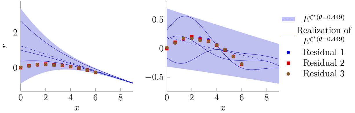
Figure 4.4 (Left) Optimal representation of the modeling discrepancy E obtained by solving Problem (4.30). (Right) Optimal representation of the modeling discrepancy E obtained by sequentially solving problems (4.32) and (4.34). Both representation of the modeling discrepancy are obtained for \theta = 0.449 . The dashed blue line is the mean of the Gaussian process while the blue-shaded area is the 95% prediction interval. Some realizations of the priors are displayed by thin lines.
