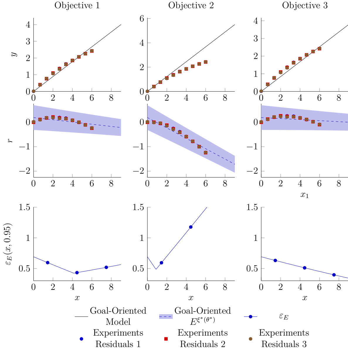
Figure 4.7 Goal-oriented calibration for the first objective (left), the second objective (middle), and the third objective (right). The top row illustrates the optimal model predictions. The middle row presents the associated residuals and modeling discrepancy E^{\xi^*}(\theta^*) . The bottom row displays the corresponding quantile error functions.
