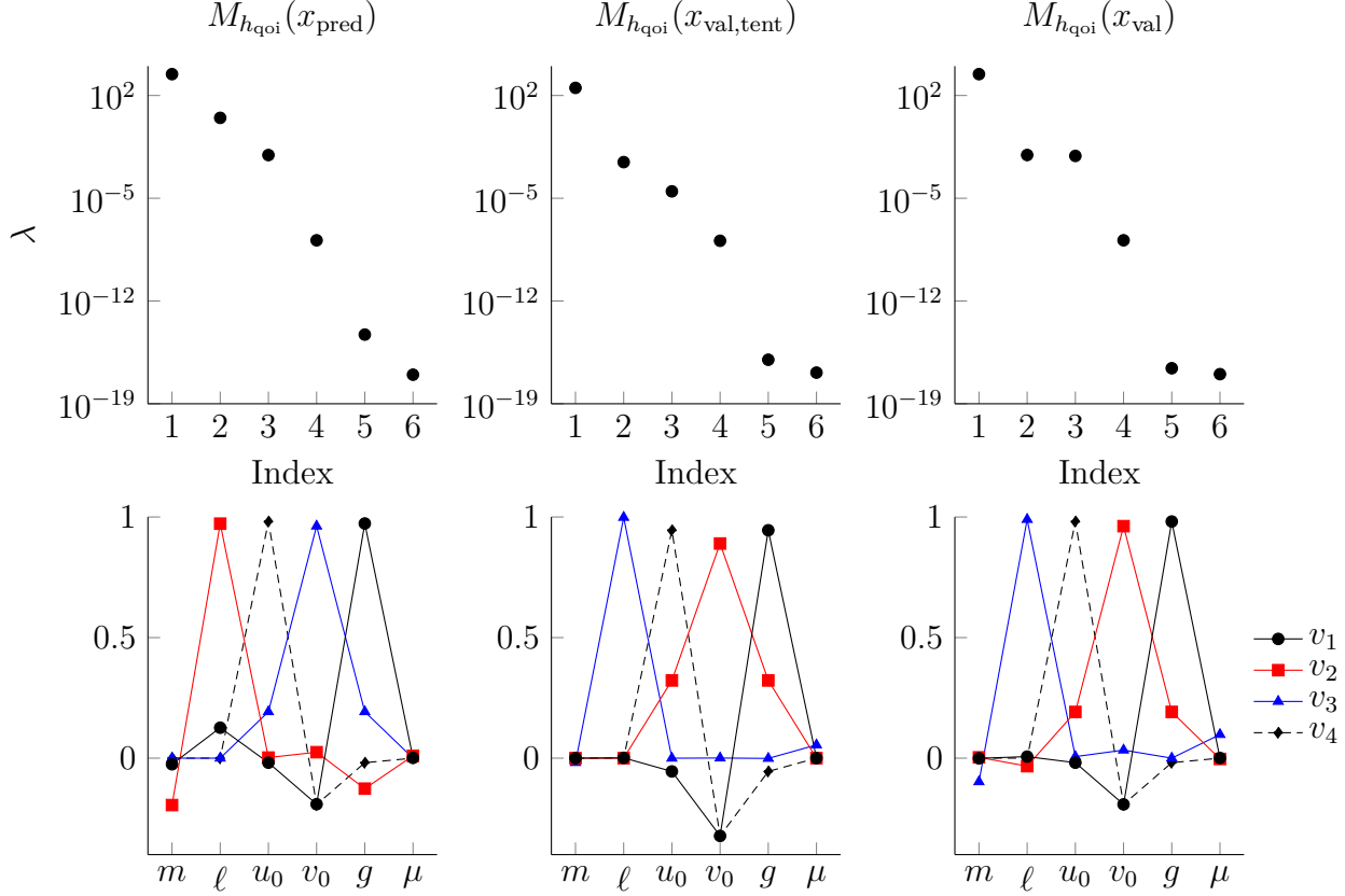
Figure 3.3 Eigenvalues (top row) and eigenvectors (bottom row) associated with the influence matrices of the QoI (3.15) for the prediction scenario x_{\text{pred}} (left), the tentative validation scenario x_{\text{val,tent}} (center), and the optimal validation scenario x_{\text{val}} (right). For the sake of clarity, only the first four eigenvectors associated with the largest four eigenvalues are displayed as the values of the other two eigenvalues are negligible.
