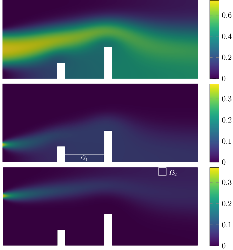
Figure 3.7 Concentration of the pollutant for the prediction and optimal validation scenarios: (top) prediction scenario, (center) optimal validation scenario associated with h_{\text{qoi},1} , (bottom) optimal validation scenario associated with h_{\text{qoi},2} .
