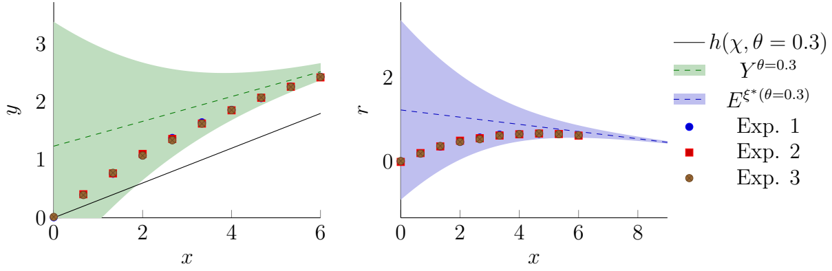
Figure 4.9 One possible optimal solution to the calibration Problem (4.25). The optimal model prediction and associated modeling discrepancy are displayed for the optimal model parameters \theta^* = 0.3 .
