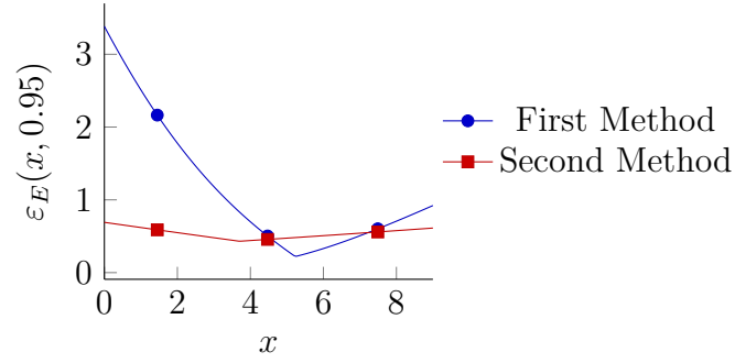
Figure 4.5 Quantile error function (4.38) for the modeling discrepancy obtained with the first and second calibration approaches. The value of \alpha is fixed at 95%.
