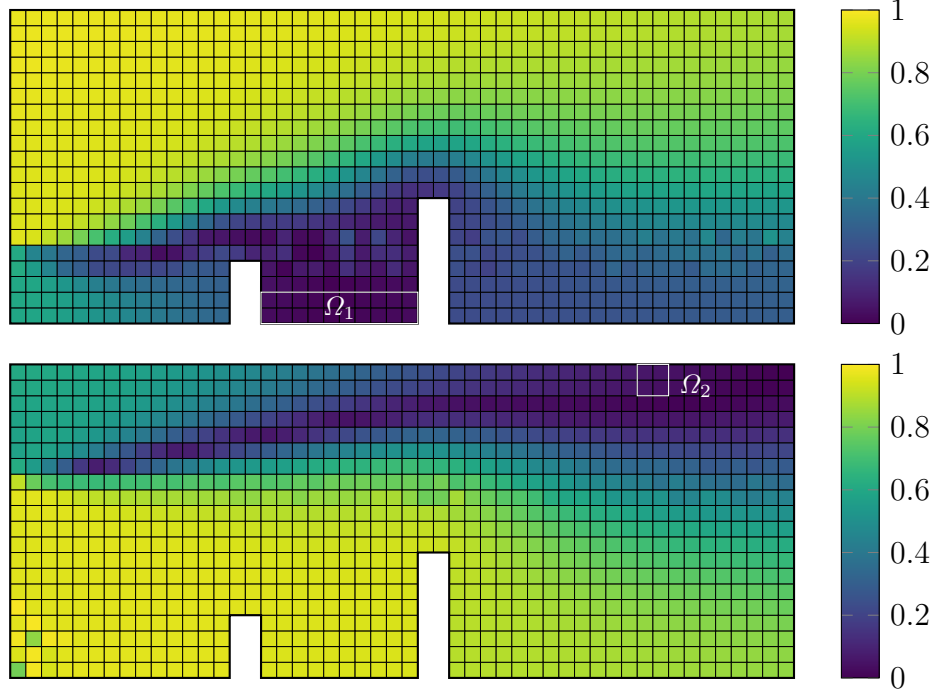
Figure 3.9 Value of the objective function in (3.14) for the first QoI (top) and second QoI (bottom).
