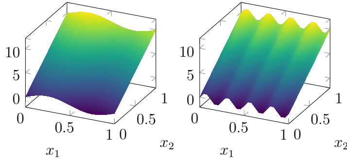
Figure 2.2 Function (2.23) for n = 1 (left) and for n = 4 (right).
