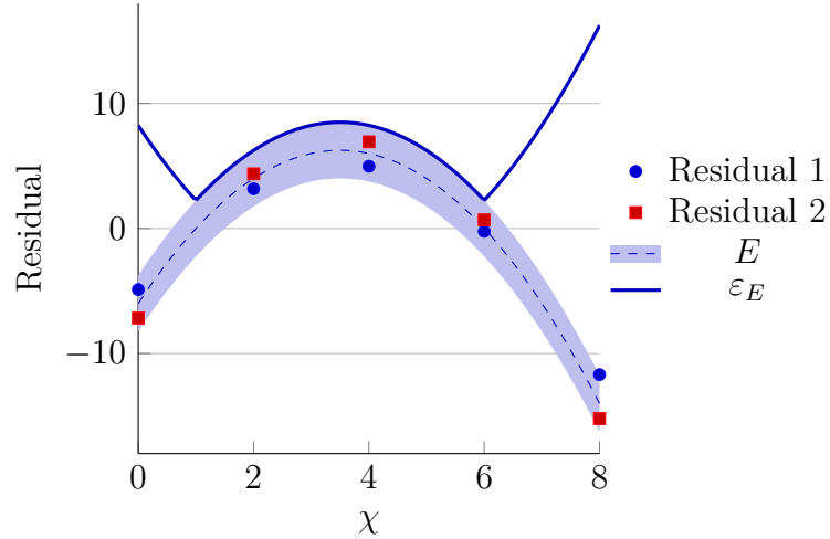
Figure 4.2 Illustration of the quantile error function \varepsilon_E from the modeling discrepancy E (illustrated in blue). The dashed curve indicates the mean function of the Gaussian process while the shaded area represent the 95% prediction interval. Two sets of residuals are displayed for illustrative purpose.
