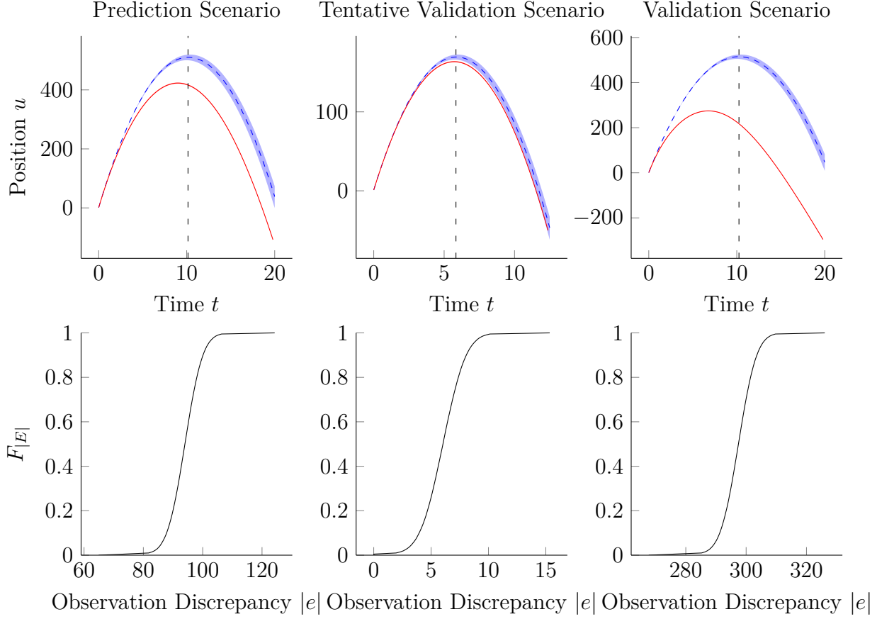
Figure 3.5 Position u (top row) and discrepancies (bottom row) for the prediction scenario (left column), tentative validation scenario (center column), and the optimal validation scenario (right column). The experimental observations are in red and the model observations are in blue. The shaded areas represent the 95% confidence interval for both the experimental and model observations. The absolute value of the discrepancies (3.5) are computed at the sensor location indicated by the black dashed lines.
