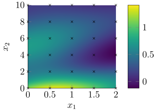
Figure 4.10 Surface of response of the manufactured solution and the design of experiments marked by black crosses.
