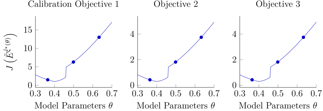
Figure 4.8 Profiles of the calibration functional for the first objective (left), the second objective (middle), and the third objective (right) with the representation (4.43) of the modeling discrepancy.
