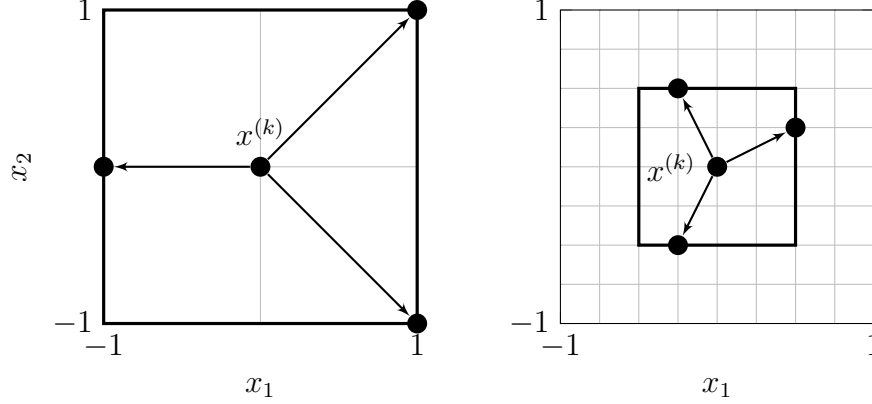
Figure 2.5 Illustration of two poll steps of the MADS algorithm. The two frames are depicted by thick squares and the candidate points are shown as points. If no candidate points decrease the objective function (left), the frame and mesh are reduced and new candidate points are considered (right).
