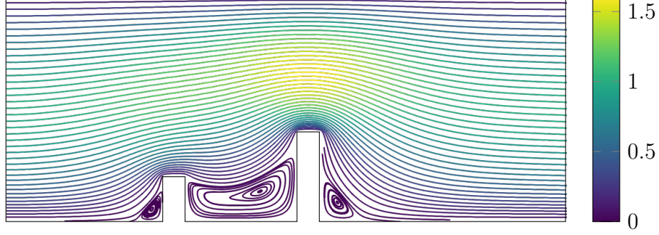
Figure 3.10 Streamline of the velocity field v
