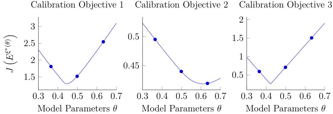
Figure 4.6 Profiles of the calibration functional for the first objective (left), the second objective (middle), and the third objective (right).
