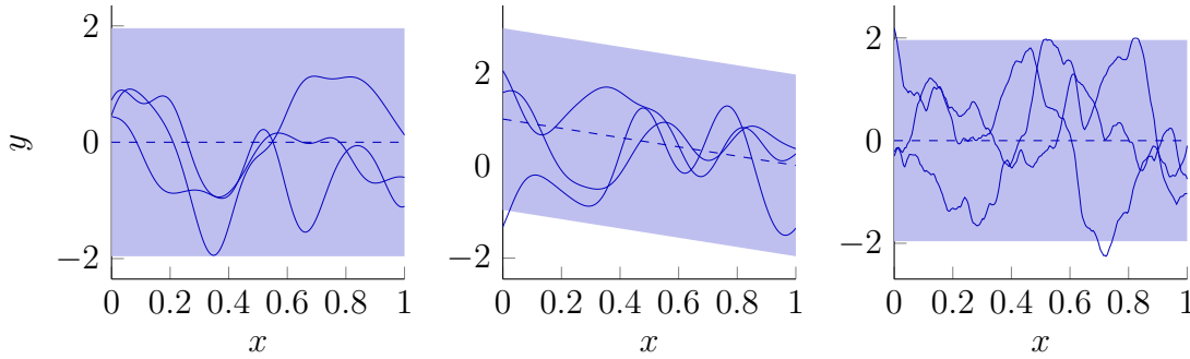
Figure 2.3 Illustration of Gaussian processes. The dashed blue lines indicate the mean function whereas the shaded areas represent the 95% prediction interval. Three realizations of the Gaussian processes are displayed by thin lines.
