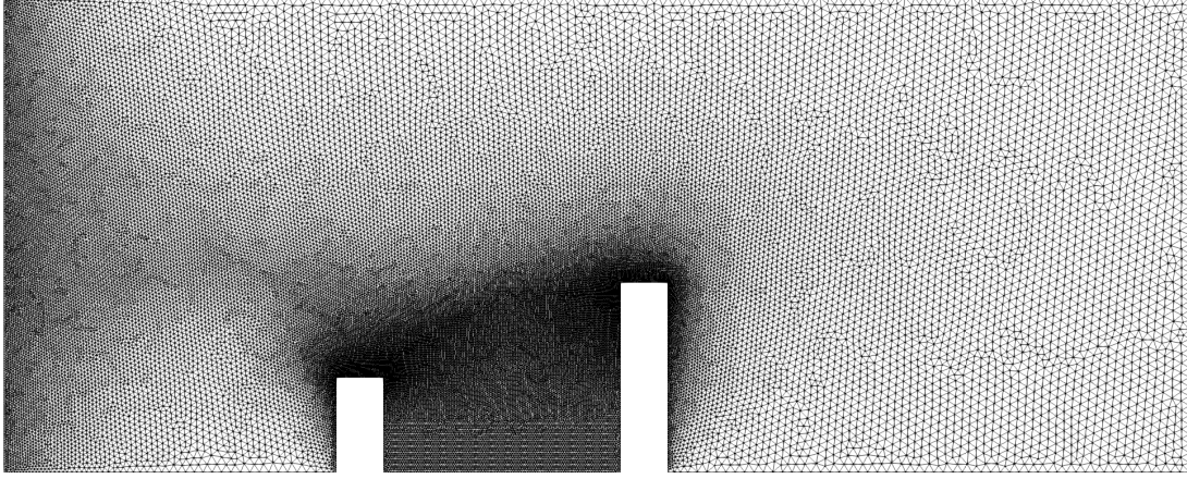
Figure 3.11 Mesh employed to compute the optimal validation scenario for the prediction of the mean concentration inside \Omega_1 .
