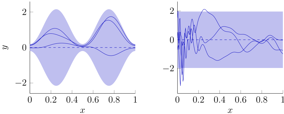
Figure 2.4 Illustration of non-stationary Gaussian processes constructed from the Gaussian kernel. The dashed blue lines indicate the mean function whereas the shaded areas represent the 95% prediction interval. Three realizations of the Gaussian processes are displayed by thin lines.
