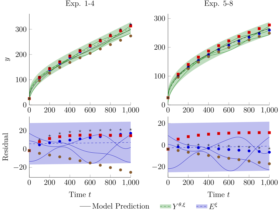
Figure 4.1 Illustration of the Gaussian process Y^{\theta,\xi} (top row) and the modeling discrepancy E^\xi for the thermal problem. The experimental data and the corresponding residuals are displayed by various marks. The mean functions of the Gaussian processes are displayed in dashed and some realizations are shown with thin lines.
