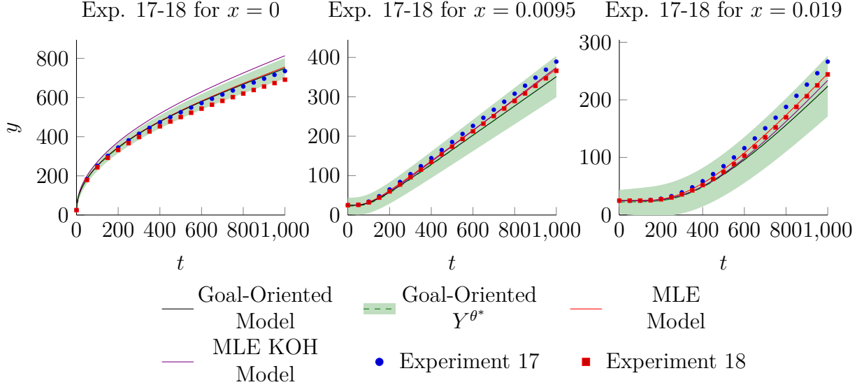
Figure 4.12 Accreditation data and model predictions for the second goal-oriented calibrated model (black), the MLE calibrated model (red) and the MLE KOH calibrated model (violet). The Gaussian process Y^{\theta^*} for the second goal-oriented calibration is displayed in green.
