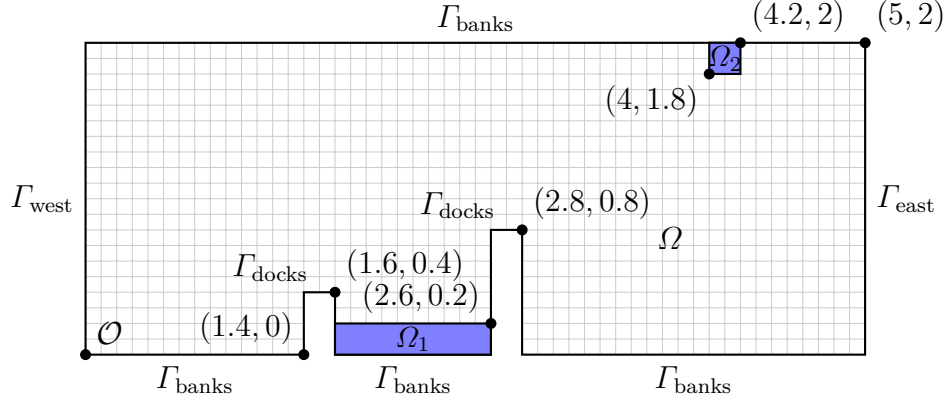
Figure 3.6 Domain \Omega and its boundaries for the contaminant transport model. The regions for which we seek the mean pollutant concentration are indicated by \Omega_1 and \Omega_2 (respectively employed for the definition of the QoIs). The grid is used to indicate the regions \Omega_{\text{obs}} in which the mean concentration of pollutant can be observed.
