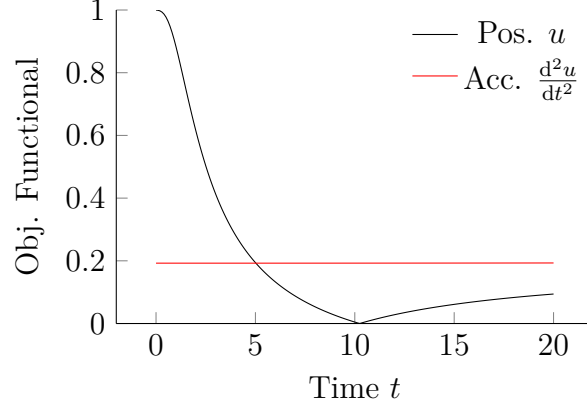
Figure 3.4 Objective functional of Problem (3.14) associated with the observation functionals h_{\text{obs}}(x_{\text{val}}, \Theta, z) := u and h_{\text{obs}}(x_{\text{val}}, \Theta, z) := d^2u/dt^2 .
