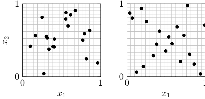
Figure 2.1 Monte Carlo sample (left) and Latin Hypercube sample (right) for N = 20 .
