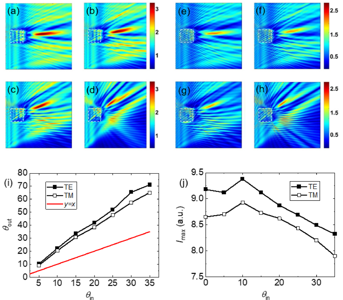
Figure 9. (a–d) The electric field distributions of the TJ formed by a BDS-coated dielectric cube with R = 300 \mu\text{m} and d_{DS} = 1.5 \mu\text{m} at Fermi energy of E_F = 55 \text{ meV} for source rotation angles of (a) 5^\circ , (b) 10^\circ , (c) 20^\circ , and (d) 35^\circ for the TE case. (e–h) The TM counterparts of (a–d). The dashed squares represent the boundary of the cube. (i, j) The output angle and intensity of the TJ, respectively, as a function of the uniform beam rotation angle.
