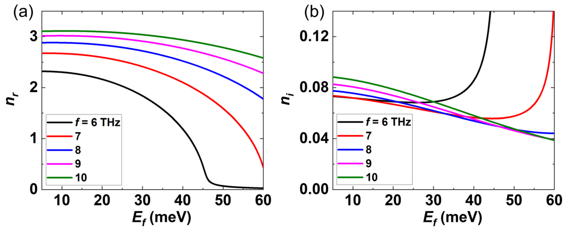
Figure 2. The index of refraction of a BDS, mimicking \text{Na}_3\text{Bi} or \text{Cd}_3\text{As}_2 , versus E_f at several THz frequencies at room temperature: (a) real and (b) imaginary part.
