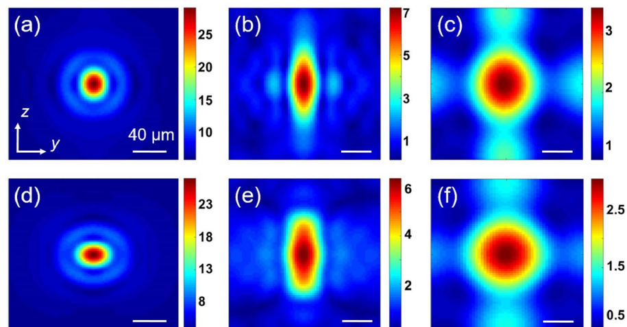
Figure 6. Distribution of the electric field inside and around a BDS-coated (a, d) sphere ( R = 500 \mu\text{m} and d_{DS} = 1.5 \mu\text{m} ), (b, e) cylinder ( R = 300 \mu\text{m} and d_{DS} = 1.5 \mu\text{m} ), and (c, f) cube ( R = 300 \mu\text{m} and d_{DS} = 1.5 \mu\text{m} ) at T = 300 K and E_F = 55 meV. Polarization of the incident wave is along the (a–c) z -axis (TE) and (d–f) y -axis (TM). Scale bars are 40 \mu\text{m} .
