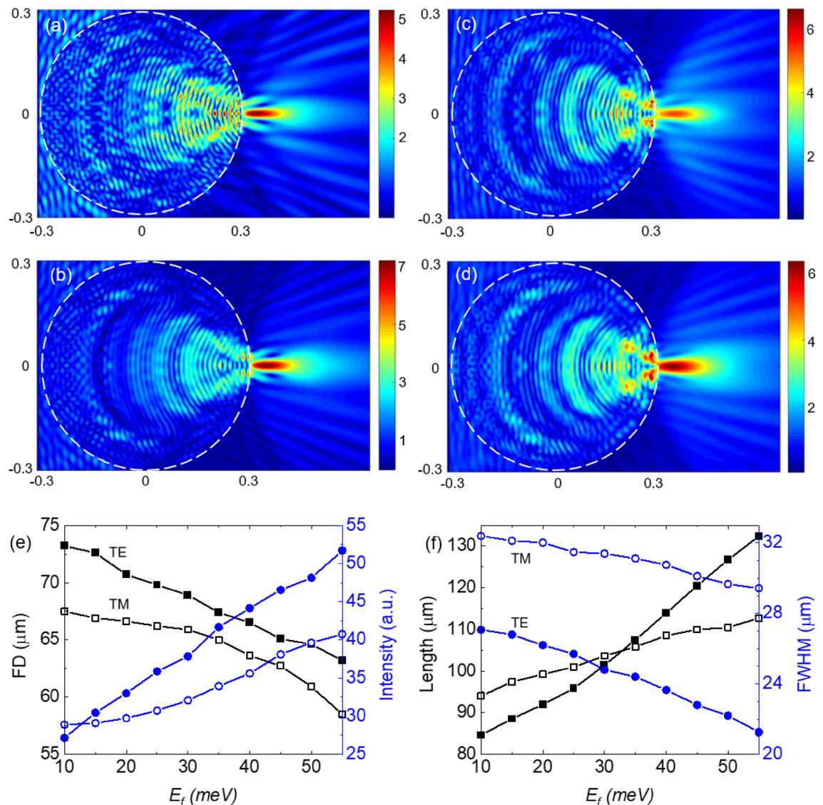
Figure 4. The distribution of the electric field inside and around a BDS-coated cylinder with R = 300 \mu\text{m} and d_{DS} = 1.5 \mu\text{m} at T = 300 \text{ K} for (a) E_F = 10 \text{ meV} (TE), (b) E_F = 55 \text{ meV} (TE), (c) E_F = 10 \text{ meV} (TM), and (d) E_F = 55 \text{ meV} (TM). (e) TJ's FD (square symbols) and intensity (circle symbols) versus E_F . (f) TJ's calculated length (square symbols) and FWHM (circle symbols) versus E_F . Hollow (solid) symbols correspond to TM (TE) polarization of the incident uniform beam.
