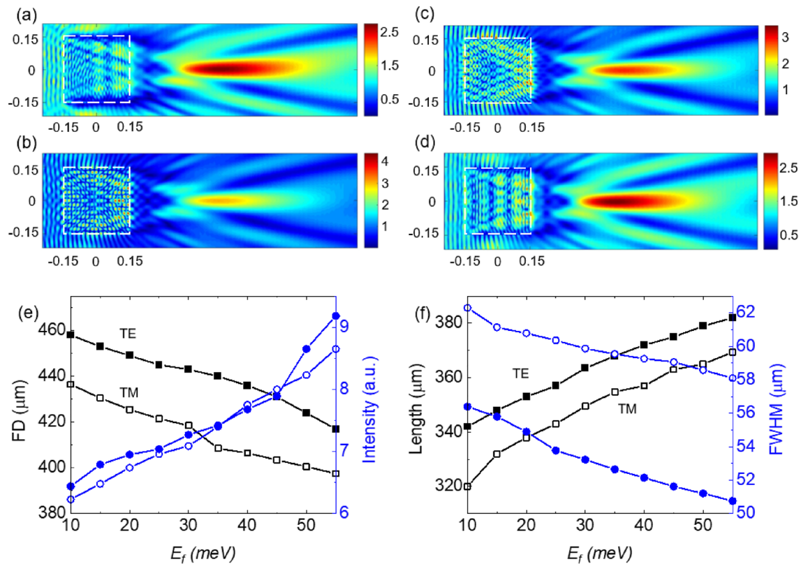
Figure 5. Distribution of the electric field distribution around and inside a BDS-coated cube with R = 300 \mu\text{m} and d_{DS} = 1.5 \mu\text{m} at T = 300 K for (a) E_F = 10 meV (TE), (b) E_F = 55 meV (TE), (c) E_F = 10 meV (TM), and (d) E_F = 55 meV (TM). (e) Plot of FD (square symbols) and intensity (circle symbols) vs. E_F . (f) TJ's length (square) and FWHM (circle) versus E_F . Hollow (solid) symbols correspond to TM (TE) polarization of the light source.
