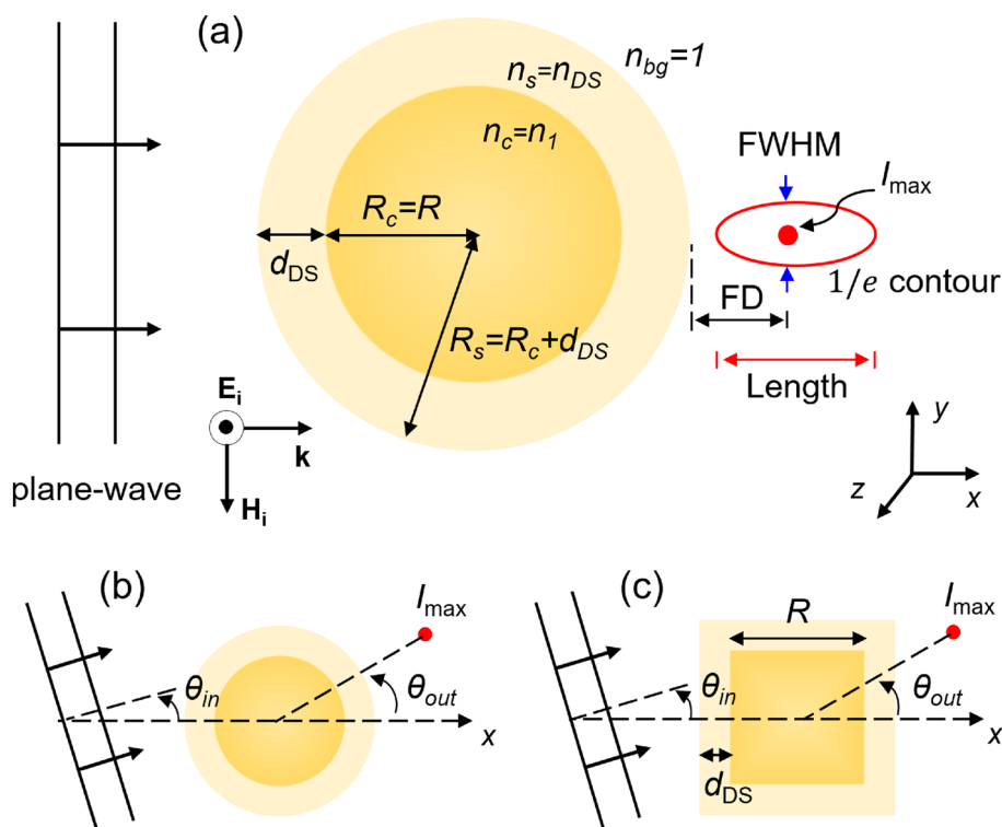
Figure 1. Schematic of the simulation geometry. A uniform beam, propagating along the x -axis, impinges upon a sphere (radius R ), a cylinder (radius R and height h ), and a cube (length R ) with refractive index n_1 coated with a BDS with thickness d_{DS} and index n_{DS} . (a) Terajet characteristics include focal distance (calculated from the proximal surface of the particle to the locus of the maximum intensity), beam FWHM in xy plane, TJ length (measured as the distance between distal to proximal 1/e intensity contour along the direction of the TJ, i.e. x -axis), and the maximum relative intensity. Geometry of oblique incident for a (b) sphere/cylinder and (c) cube. In the core-shell structure shown in panel (a) , n_c ( R_c ) and n_s ( R_s ) represent the refractive indices (radii) of the core and shell, respectively. Drawings are not to scale.
