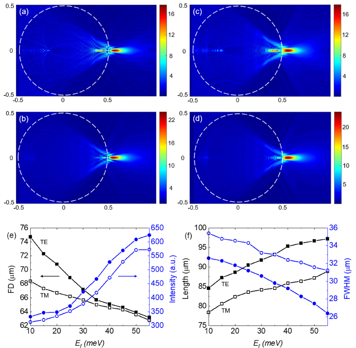
Figure 3. The electric field distribution inside and around a BDS-coated dielectric sphere with R=500\text{ }\mu\text{m} and d_{DS}=1.5\text{ }\mu\text{m} at T=300\text{ K} for (a) E_F=10\text{ meV} (TE), (b) E_F=55\text{ meV} (TE), (c) E_F=10\text{ meV} (TM), and (d) E_F=55\text{ meV} (TM). (e) TJ's calculated FD (square symbols) and intensity (circle symbols) versus E_F . (f) TJ's length (square symbol) and FWHM (circle symbol) versus E_F . Hollow (solid) symbols correspond to TM (TE) polarization of the incident uniform beam.
