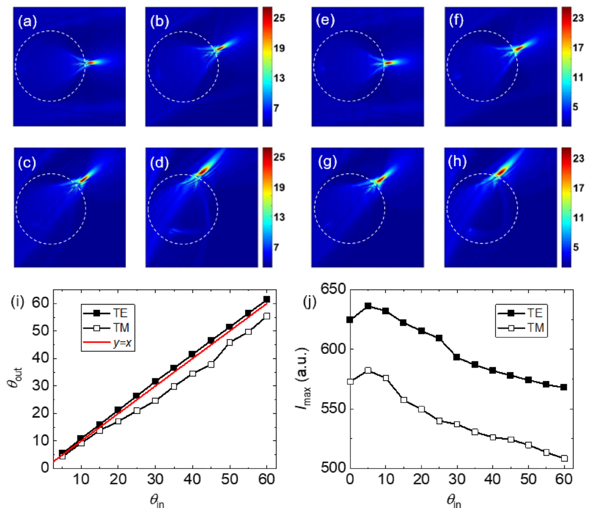
Figure 7. (a–d) The electric field distributions of the TJ formed by a BDS-coated dielectric sphere with R = 500 \mu\text{m} and d_{\text{DS}} = 1.5 \mu\text{m} at Fermi energy of E_F = 55 meV for input angles of (a) 5°, (b) 25°, (c) 40° and (d) 60° for the TE case. (e–h) The TM counterparts of (a–d). The dashed circles show the boundary of the sphere. (i, j) The emergence angle and intensity of the TJ, respectively, as a function of the uniform beam rotation angle.
