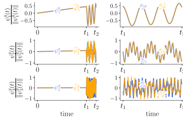
Fig. 4 Visualization [9] of the first three temporal modes (normalized) with and without Aiken acceleration, herein denoted \tilde{\psi}_i^q and \psi_i^q , respectively
