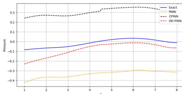
Figure 14. Numerical validation for 2D Cylinder Wake: solution evaluation against reference solution and comparison against the baseline PINN and recent related works (CPINN).
