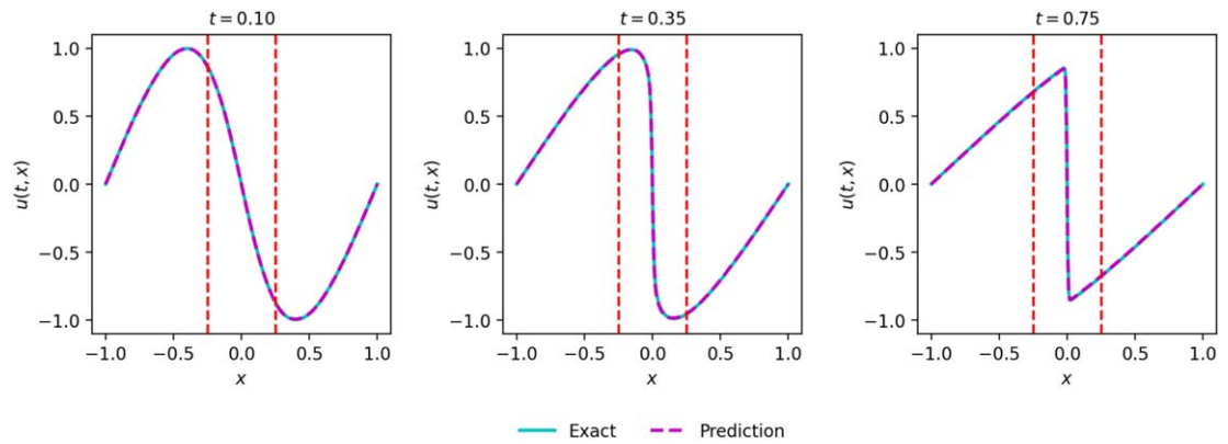
Figure 17. The DD-PINN solution and comparison of exact and predicted solutions at t = 0.10 , t = 0.35 , and t = 0.75 for the viscous Burgers equation. The red dashed lines indicate the locations of the interfaces.
