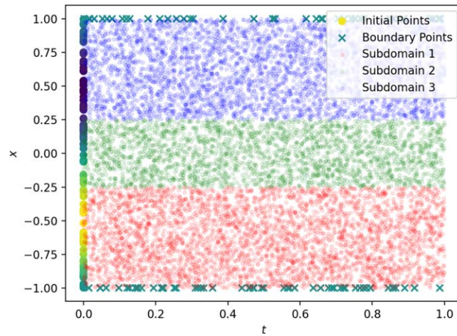
Figure 16. The problem domain: one-dimensional viscous Burgers equation.
