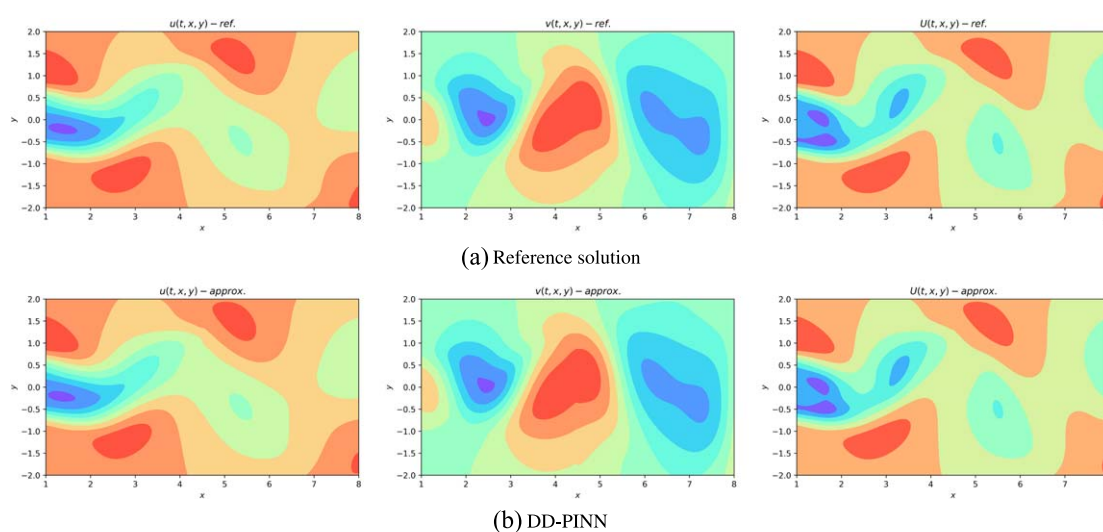
Figure 15. 2D cylinder wake problem; velocity fields. From the left to the right: velocity components at x direction, y direction and velocity magnitude.
