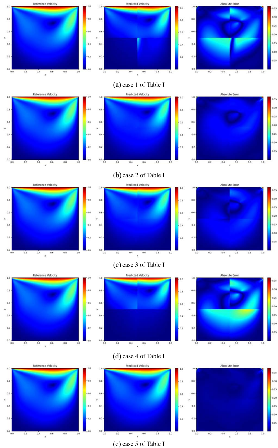
Figure 5. LDC problem: velocity fields.
