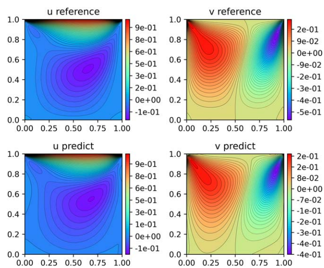
Figure 8. Velocity components contours: from top to bottom: reference solution, and DD-PINN with TRF.
