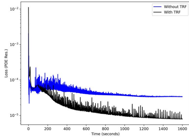
(a) Residual loss
