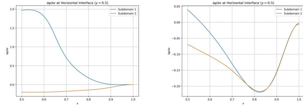
(b) Differentiability of \psi at horizontal interface ( x -direction)
