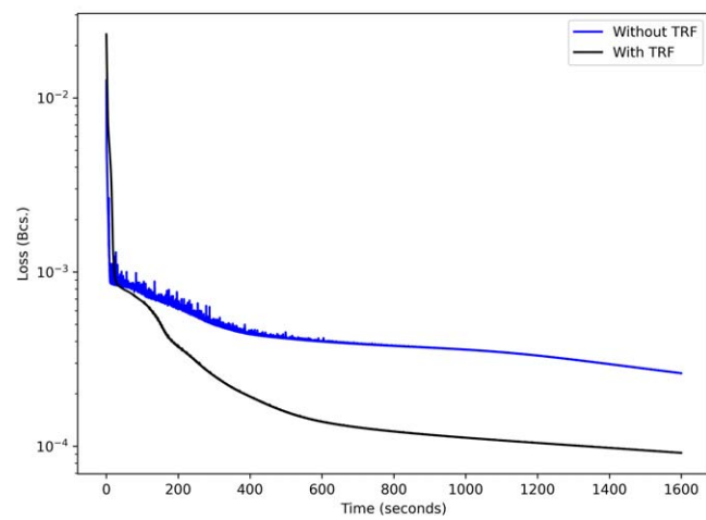
(b) BCs loss
