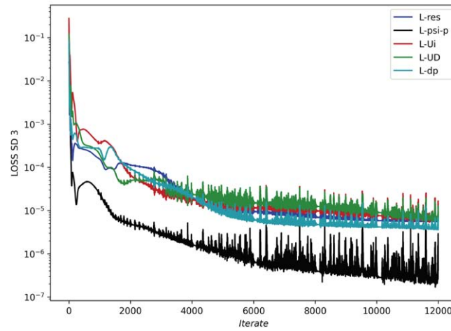
(b) DD-PINN with sub-network TRF
