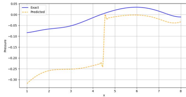
Figure 12. Dominant subdomain: analysis of subdomains in terms of solution accuracy.
