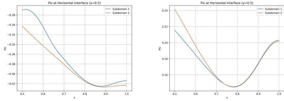
(a) Continuity of \psi at horizontal interface
