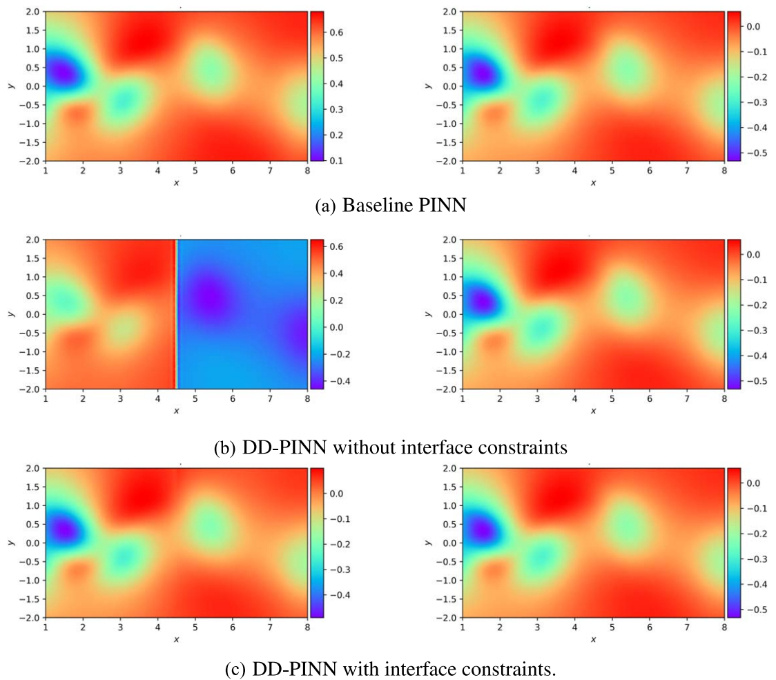
Figure 13. 2D cylinder wake problem; Pressure fields. Left and right columns show approximated and reference pressure fields, respectively.
