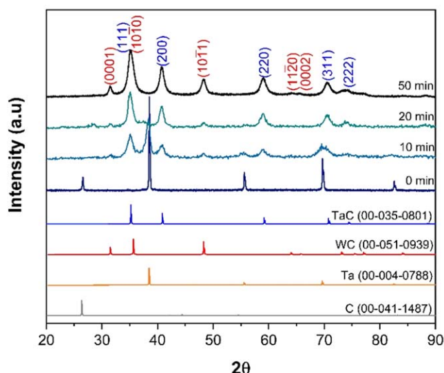
Figure 1. X-ray powder diffraction patterns of sample at different milling times.
