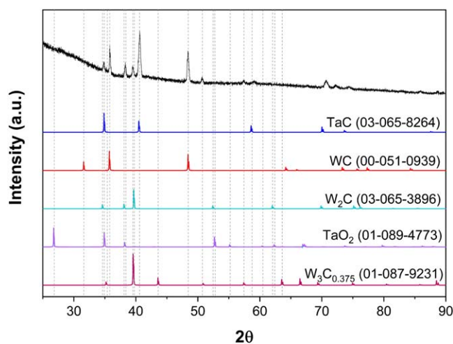
Figure 12. XRD pattern of the TaC-WC pellet.
