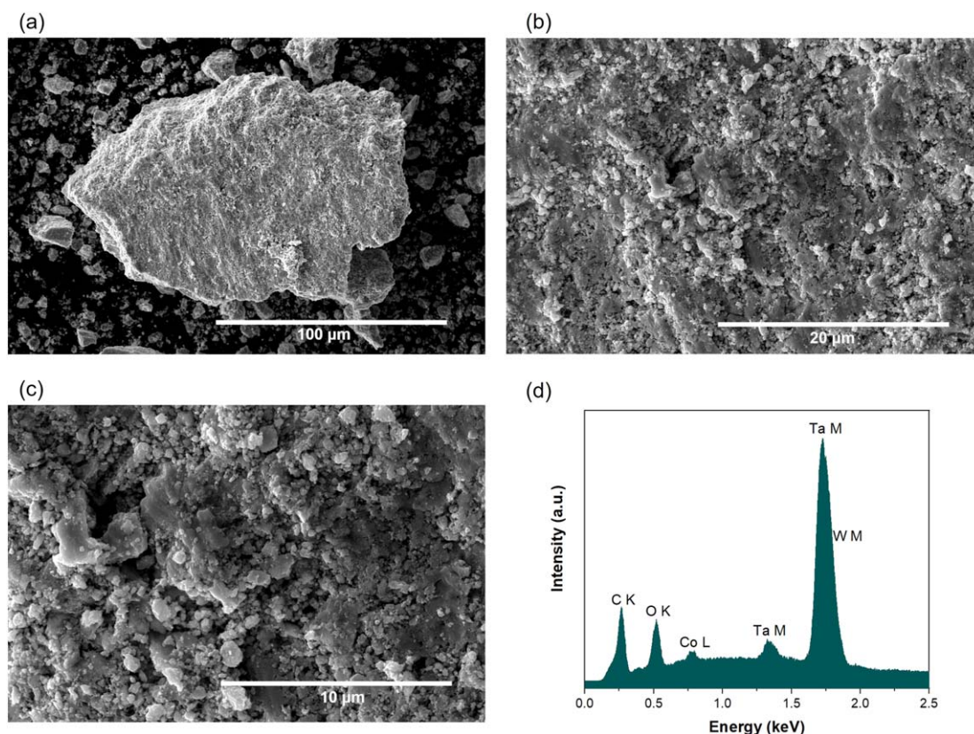
Figure 5. SEM micrographs and EDS of the sample at 50 min of milling, (a)–(c) SE images at different magnifications and (d) EDS spectra.
