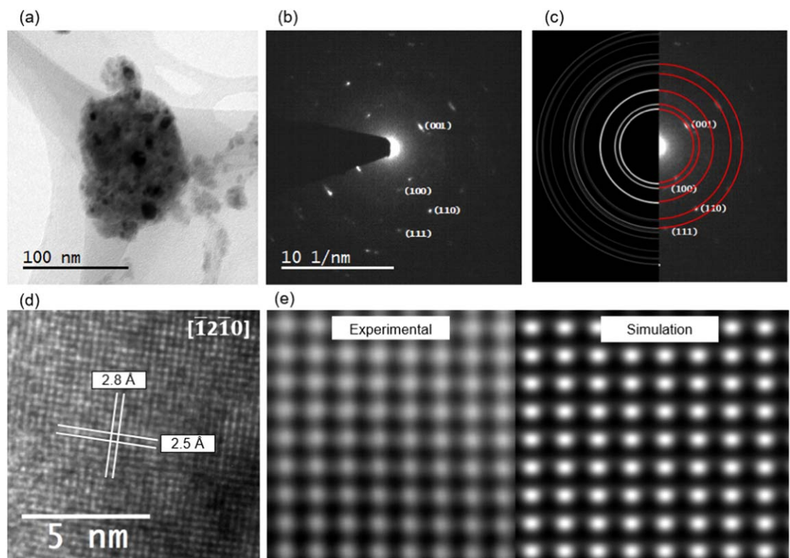
Figure 7. TEM analysis of the TaC-WC sample at 50 min of milling, showing WC particles, (a) low magnification BF image, (b) experimental DP from image (a), (c) simulated DP versus experimental DP, (d) HR-TEM micrograph from (a) and (e) experimental HR-TEM versus simulated HR-TEM.
