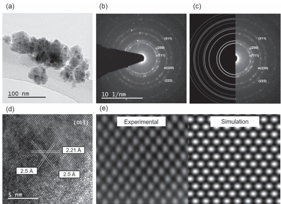
Figure 6. TEM analysis of the TaC-WC sample at 50 min of milling, showing TaC particles, (a) low magnification BF image, (b) experimental DP from image (a), (c) simulated DP versus experimental DP, (d) HR-TEM micrograph from (a) and (e) experimental HR-TEM versus simulated HR-TEM.
