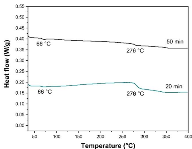
Figure 9. DSC curves at 20 and 50 min of milling time.
