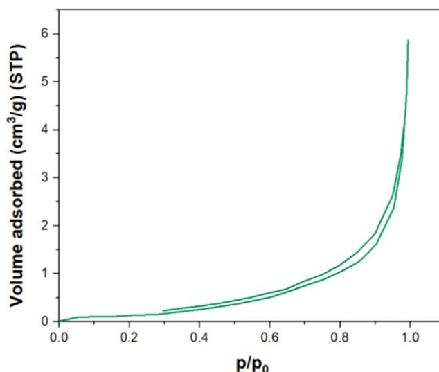
Figure 8. Nitrogen adsorption and desorption isotherms by BET method.
