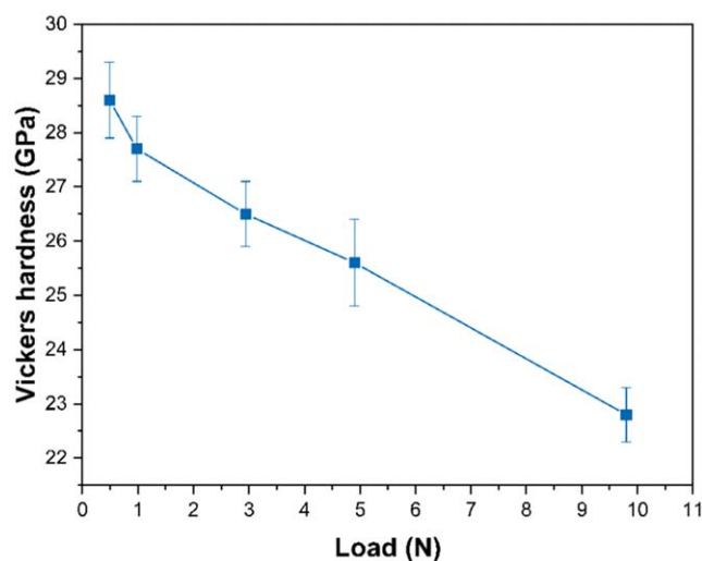
Figure 13. Vickers hardness graph of the TaC-WC at different loads.
