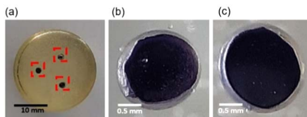
Figure 10. (a) TaC-WC pellets formed with an electric arc furnace mounted on an EPOXY resin, (b) and (c) magnification of pellets in (a).
