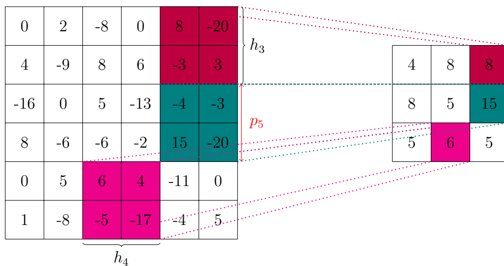
Figure 2.5 Max-pooling
