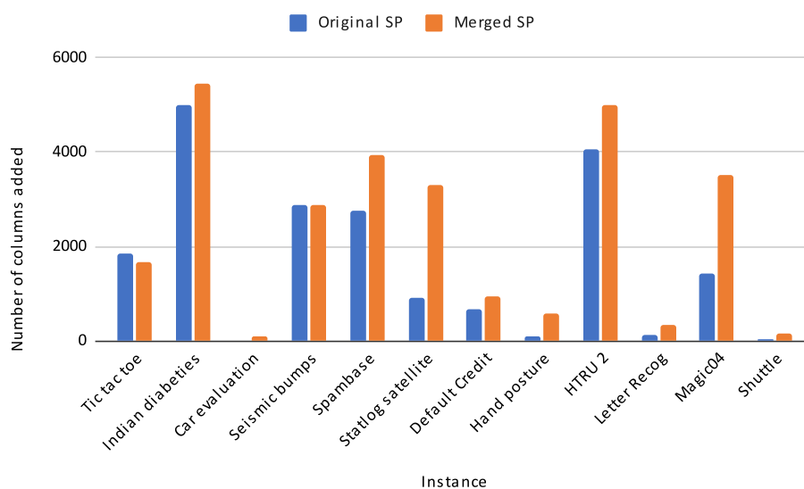
Figure 4.3 Number of columns added with original and merged SPs.
