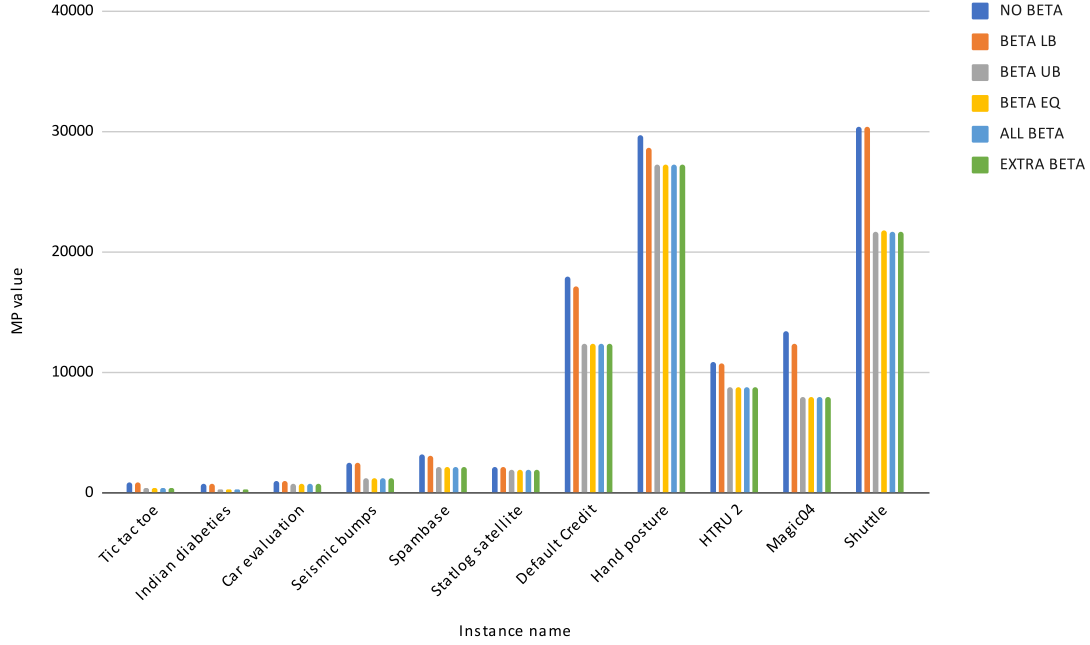
Figure 4.6 MP value for different ways of using constraints (4.1c).
