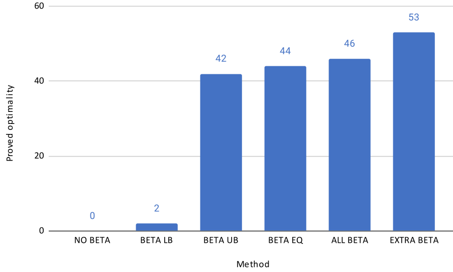
Figure 4.8 Number of instances solved to optimality for different ways of using constraints (4.1c).
