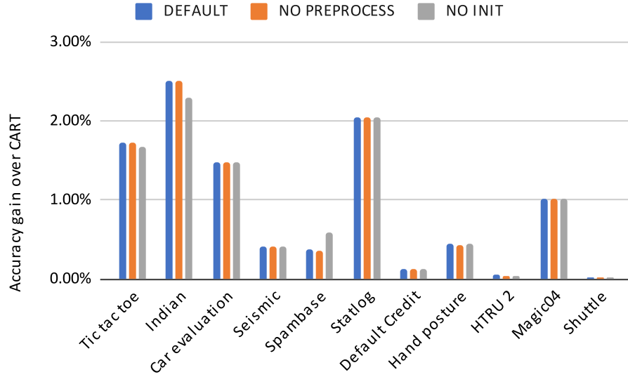
Figure 4.2 Accuracy gain over CART for different ways of using preprocessing and initialization.
