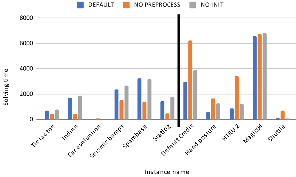
Figure 4.1 Solving time for different ways of using preprocessing and initialization.
