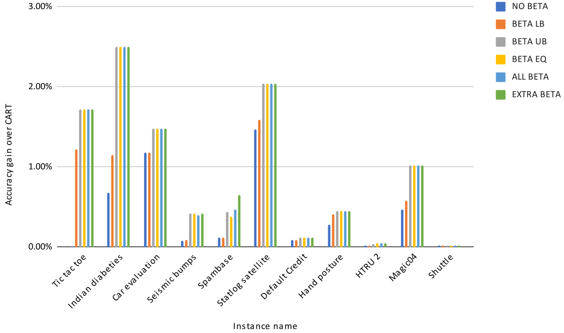
Figure 4.7 Training accuracy gain over CART for different ways of using constraints (4.1c).
