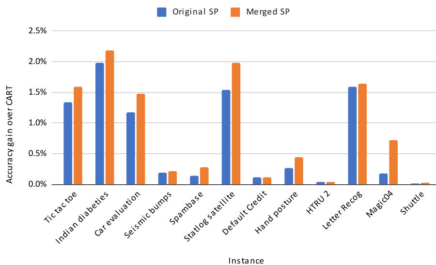
Figure 4.4 Accuracy gain over CART on training datasets with original and merged SPs.
