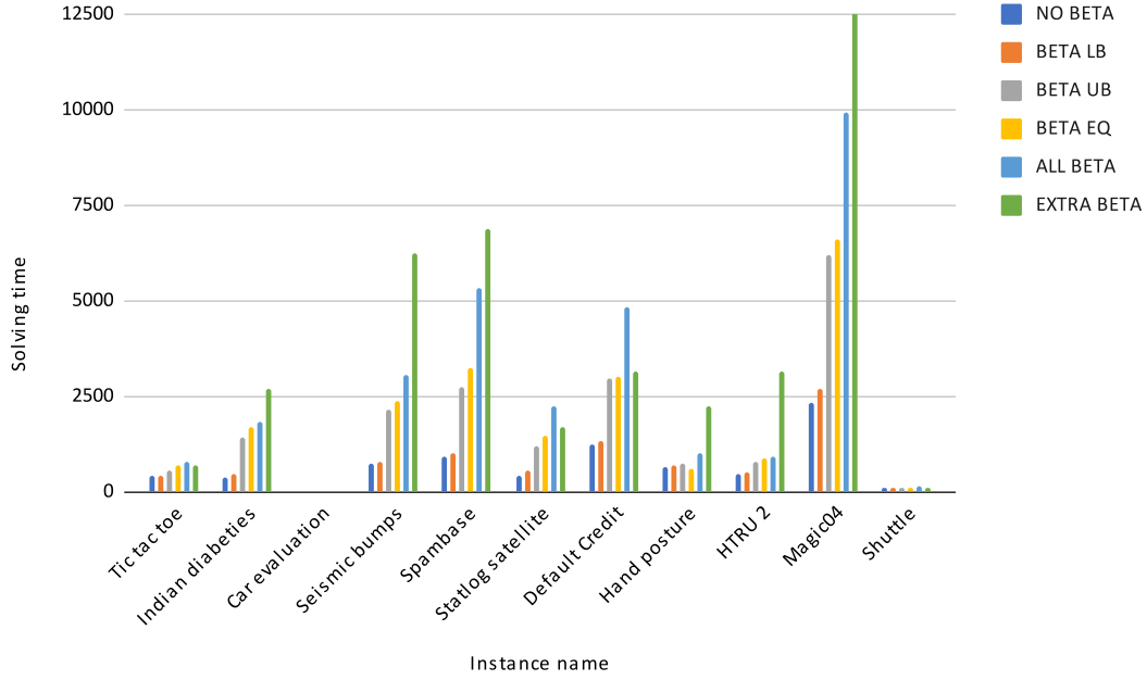
Figure 4.5 Solving time for different ways of using constraints (4.1c).
