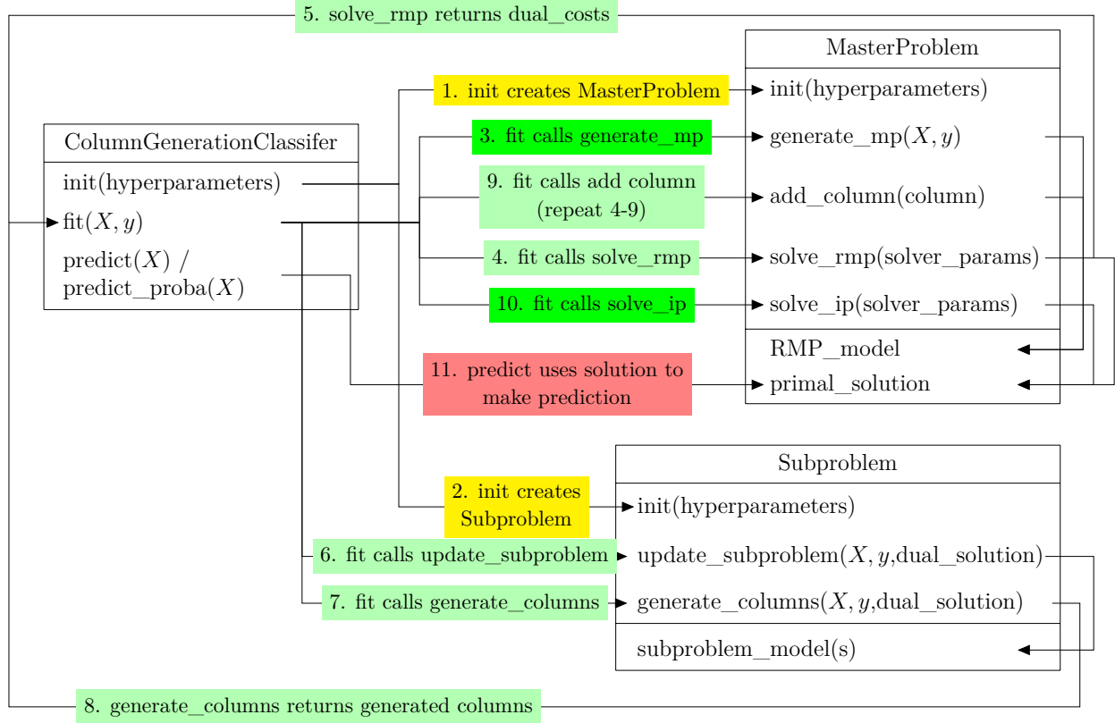
Figure 5.1 Interaction between different classes in the workflow of the CG Framework.
