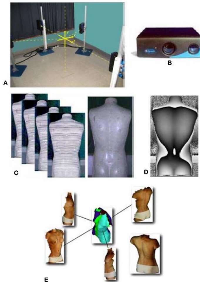
Figure 2.7 Trunk topography measurement and reconstruction A) Experimental set-up at Sainte-Justine Hospital of four Creaform optical digitizers. (B) Example of a Capturor II LF 3D optical digitizer, consisting of a CCD camera coupled with a structured light projector. (C) Set of four fringe images, each offset by 1/4 phase, projected by a digitizer onto the back of a mannequin; the fifth image provided the surface texture. (D) Resulting phase image from the four fringe images (E) The process of registering and merging the partial surfaces from the different digitizers produces the complete trunk surface
