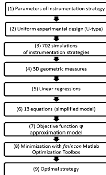
Figure 2.15 Flow chart summarizing the Materials and Methods
