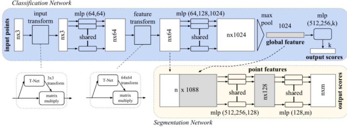
Figure 2.22 Architecture of PointNet [52]
