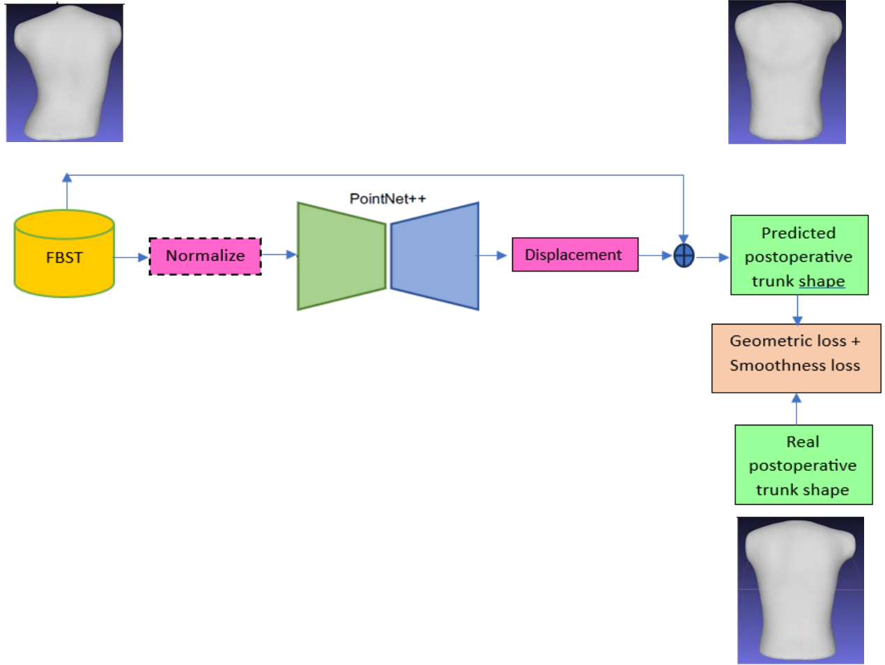
Figure 3.1 Workflow of the proposed method
