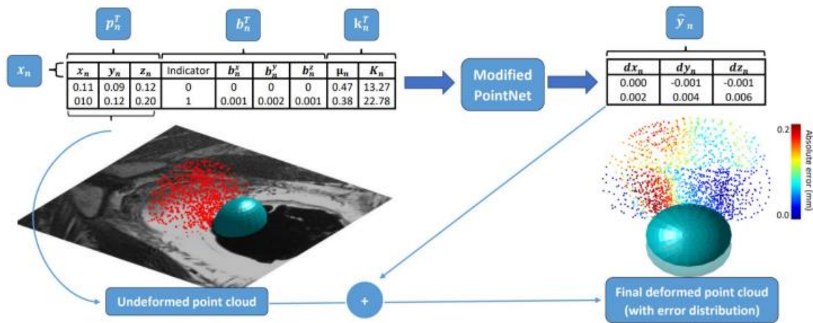
Figure 2.18 Overview of methodology of final deformed point cloud
