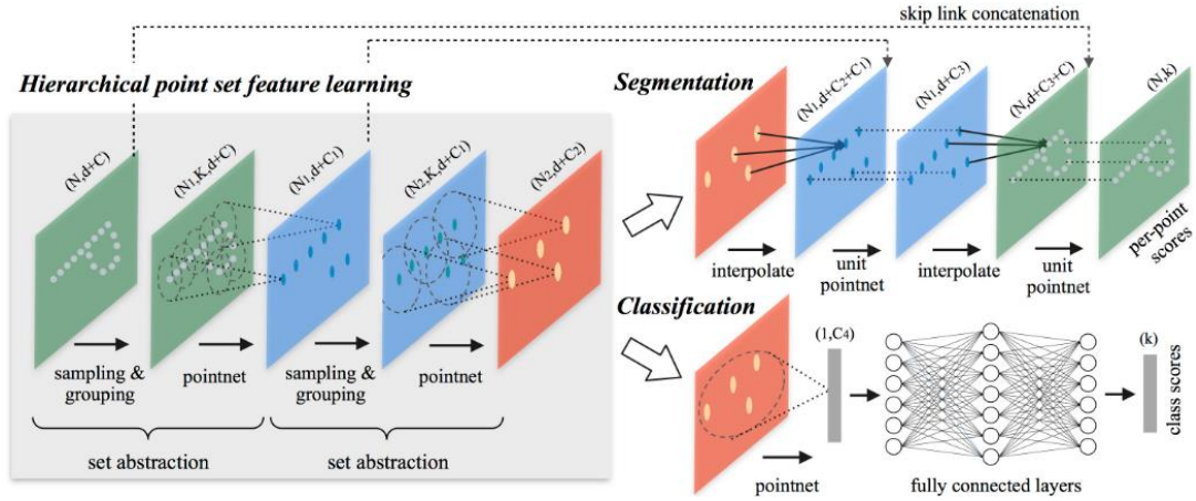
Figure 2.23 Architecture of PointNet++ [53]
