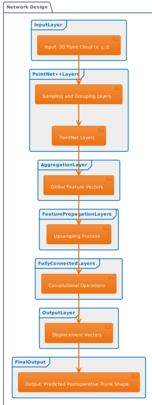
Figure 3.3 PointNet++ Network Design
