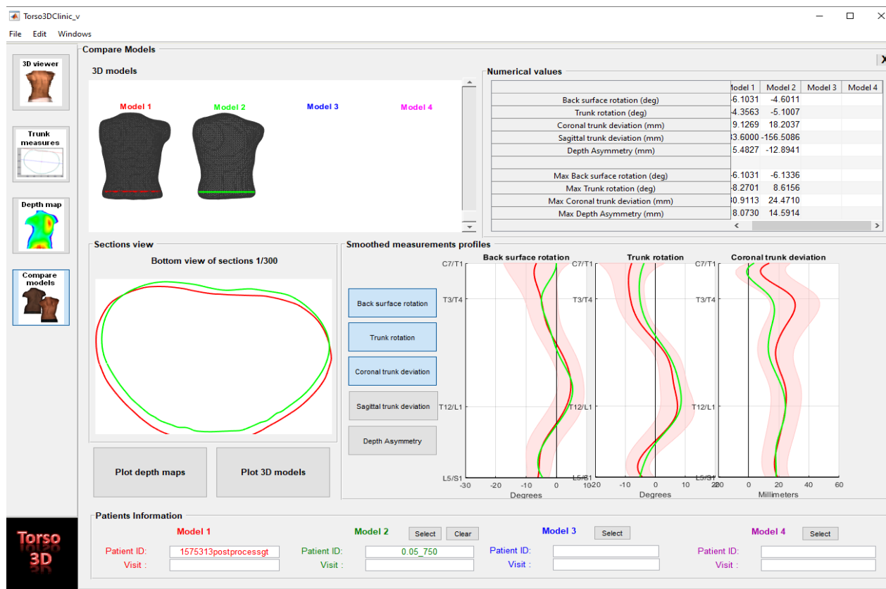
Figure 4.1 Torso 3D- Graphical User Interface to view measurements by using the slider (top left). Bottom left: sections of the trunk seen from below. Top right: Calculated Measurements of the trunk. Bottom Right: Curves representing measurements along the trunk for each acquisition. The two colors represent two different sources (Red: InSpeck, Green: Predicted postop trunk shape).
