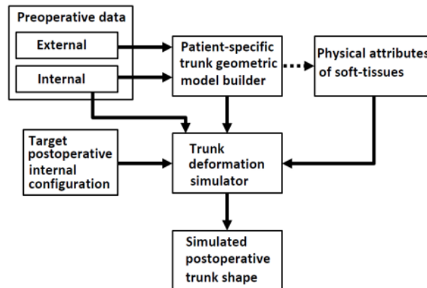
Figure 2.13 Flow chart of the postoperative trunk shape simulation
