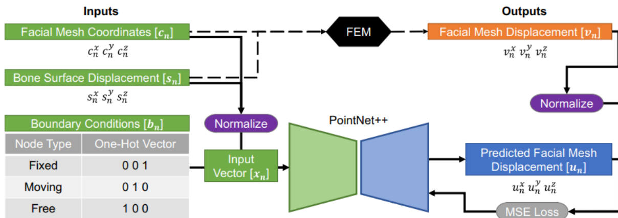
Figure 2.17 Overview of the method used for the deformation prediction
