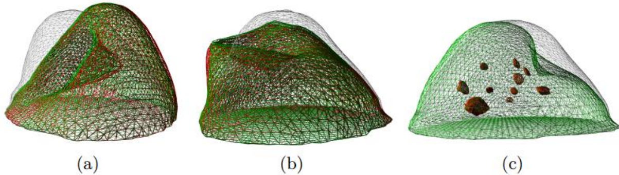
Figure 2.19 (a) Sample with maximal deformation. (b) Sample with maximal mean norm error. The green mesh is the U-Net prediction and the red mesh is the FEM solution. The initial rest shape is shown in grey. (c) U-Net prediction on phantom data.
