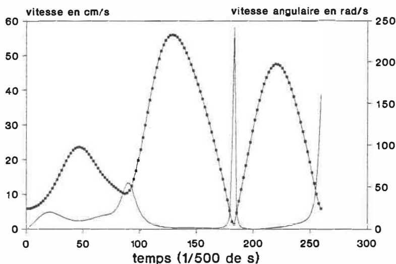
Figure III.2 Non sommation des gaussiennes
