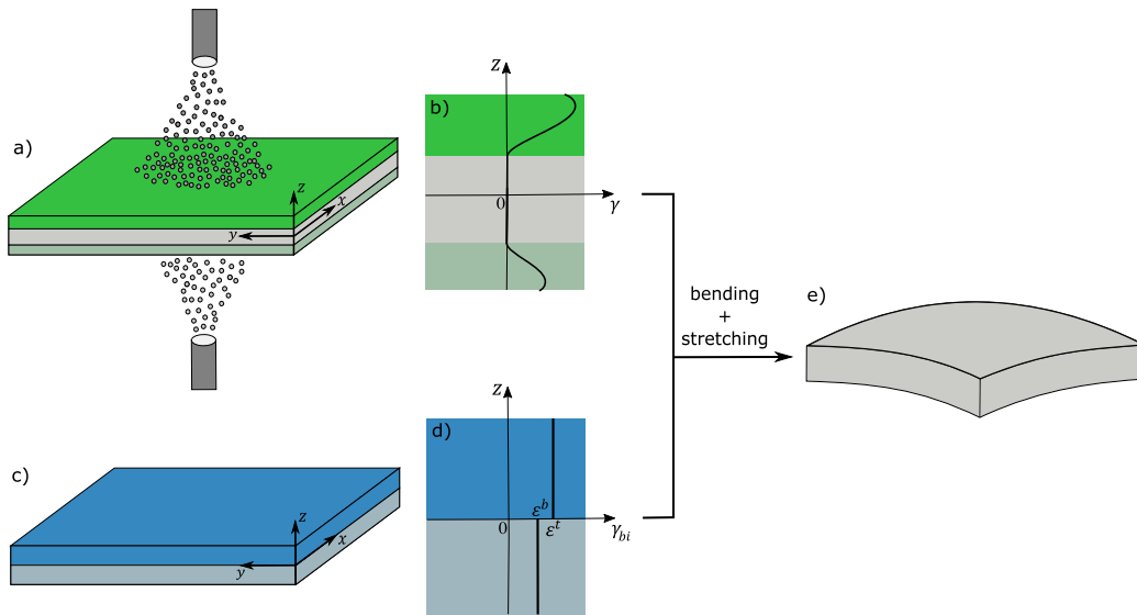
Fig. 2. Idealization of the through-thickness eigenstrain profile. In this example, we suppose that the plate is uniformly peened from both sides and that the top side peening regime is more intense. (a) The treatment induces eigenstrains in the outer layers of the plate (bright green and pale green), while the internal layer (gray) is not affected. (b) The induced eigenstrain prescribes an in-plane expansion to the outer layers, and the expansion magnitude \gamma is non-uniform along the through-thickness lagrangian coordinate z . (c) To idealize the eigenstrain profile, we represent the plate as a bilayer consisting of equally thick layers (bright blue and pale blue). (d) We prescribe a uniform eigenstrain to both layers and thus obtain an idealized through-thickness eigenstrain profile \gamma_{bi} , which is described with two variables: (\epsilon^t, \epsilon^b) . The values of \epsilon^t and \epsilon^b are computed in the way that \gamma_{bi} induces the same final shape as \gamma(z) (see Eqs. (2), (3)), in the sense of plate theory. (e) The final shape induced by \gamma_{bi} and \gamma(z) is stretched with respect to the initial state and convex towards the side where a more intense treatment was applied. (For interpretation of the references to color in this figure legend, the reader is referred to the web version of this article.)
