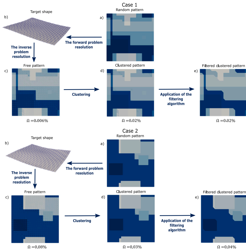
Fig. B.8. Two test cases from series 2. (a) The random peen forming pattern generated on a 1 \times 1 m sized plate using the algorithm presented by Sushitskii et al. [8]. Different colors on the peen forming pattern denote different peening regimes. (b) The target shape generated by application of the random pattern. The deflections are at the original scale. (c) The free pattern computed using the inverse problem resolution algorithm (see [8]). (d) The clustered peen forming pattern computed by application of Algorithm 1 to the free pattern. (e) The filtered clustered algorithm obtained by application of Algorithm 2 to the clustered pattern. We solved the forward problem for the patterns (c), (d) and (e) and computed the dimensionless error \Omega for each case. In case 1, the free pattern reproduces the original random pattern the best. This is due to several elements attributed to wrong clusters during clustering, so the dimensionless error \Omega is higher for the clustered pattern. In case 2, the lowest \Omega is provided by the clustered pattern, which almost exactly replicates the random pattern. Although the filtering algorithm makes the pattern fully reproducible, in case 2 the filtered clustered pattern is further from the random pattern than the clustered one. (For interpretation of the references to color in this figure legend, the reader is referred to the web version of this article.)
