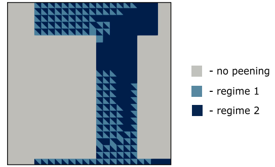
Fig. 4. Example of a peen forming pattern heavily affected by the checkerboard problem after clustering. The pattern is represented on a square plate, which is meshed with triangular finite elements. The elements assigned with different peening regimes of a close intensity are locally mixed, so the proposed pattern is not reproducible in practice.
