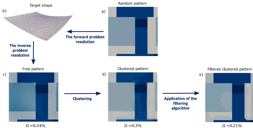
Fig. 5. One of the test cases from series 2 that demonstrated a marked checkerboard problem. (a) The random peen forming pattern generated on a 1 \times 1 m sized plate using the algorithm presented by Sushitskii et al. [8]. Different colors on the peen forming pattern denote different peening regimes. (b) The target shape generated by application of the random pattern. The plate is 6 mm thick, and the Poisson's ratio equals 0.36. The deflections are at the original scale. (c) The free pattern computed using the inverse problem resolution algorithm (see [8]). (d) The clustered peen forming pattern computed by application of Algorithm 1 to the free pattern. (e) The filtered clustered pattern obtained by application of Algorithm 2 to the clustered pattern. We solved the forward problem for the patterns (c), (d) and (e) and computed the dimensionless error \Omega for each case. In the presented case, the filtered clustered pattern reproduces the original random pattern better than the free pattern, so it leads to a lower dimensionless error \Omega . (For interpretation of the references to color in this figure legend, the reader is referred to the web version of this article.)
