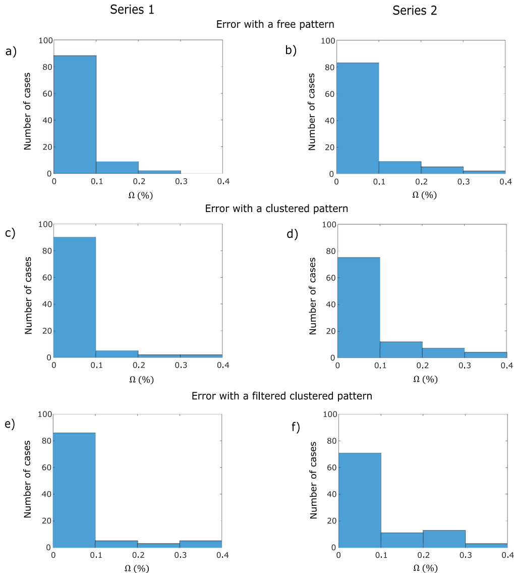
Fig. 6. Histograms plotting the dimensionless error \Omega between the target shapes and the final shapes computed during the validation of the clustering and filtering algorithms. We considered 200 test cases that were divided in two series of 100 cases each. In each case, we solved the inverse problem, clustered the peen forming pattern and applied the filtering algorithm. One peening regime was available for clustering in series 1, and four regimes were available in series 2. We simulated the application of the peen forming patterns at each stage and computed the dimensionless error \Omega . Figures (a) and (b) plot the simulated \Omega provided by the unclustered free patterns in series 1 and 2 respectively. Figures (c) and (d) trace the simulated \Omega provided by the clustered patterns, and Figures (e) and (f) show \Omega provided by the filtered clustered patterns. The filtered clustered patterns induce a slightly larger \Omega than the free patterns in general, but \Omega does not exceed 0.4% for all the types of patterns.
