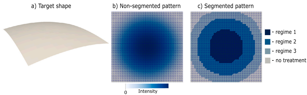
Fig. 1. Examples of a non-segmented and of a segmented peen forming pattern. Both patterns make a flat square plate deform into a spherical patch (a) when applied from both sides of the plate. The non-segmented pattern (b) prescribes a gradual variation of the peening intensity over the plate, which is hardly reproducible with peening equipment. The segmented pattern (c) is reproducible because it consists of uniformly treated segments. Both patterns are discretized with triangular finite elements, and the effect of their application can be simulated using the eigenstrain approach. For this, one must establish in advance a one-to-one correspondence between the peening regimes or the intensities, and the induced eigenstrains.
