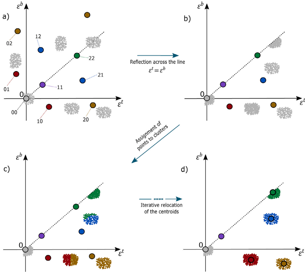
Fig. 3. Example of clustering with N = 2 available peening regimes. (a) At the beginning, the clustering algorithm traces the points (gray dots) that are to be clustered at coordinates (\epsilon^t, \epsilon^b) . Each point represents a finite element, and its coordinates reflect the eigenstrain assigned to the element by the inverse problem solver. The clustering algorithm randomly initializes the peening regimes and traces the cluster centroids (colored squares), each of which is a combination of two peening regimes for all possible permutations. The coordinates of centroid ij represent the eigenstrain induced by the application of regime i from the top side and of regime j from the bottom side. (b) Next, the algorithm eliminates the symmetry by reflecting the points that lie above the line \epsilon^t = \epsilon^b across this line. The centroids that lie above this line are deleted. (c) Subsequently, each point is assigned to the closest centroid (cluster) in terms of squared Euclidean distance. (d) The algorithm iteratively adjusts the peening regimes, derives new centroid positions and reassigns the points until the stabilization of the centroids. The centroid (0,0) is fixed at the origin during all iterations. In this example, no points were attributed to cluster 11 (purple), which corresponds to the treatment with regime 1 from both sides. (For interpretation of the references to color in this figure legend, the reader is referred to the web version of this article.)
