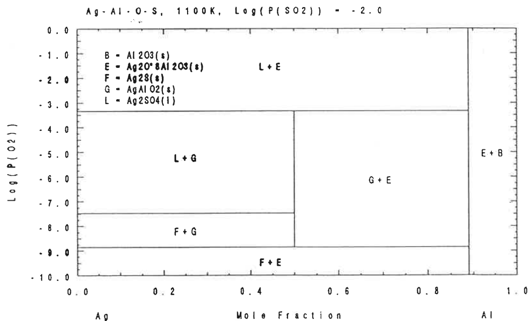
Figure 32. POTCOMP diagram for the Ag-Al-O-S system
