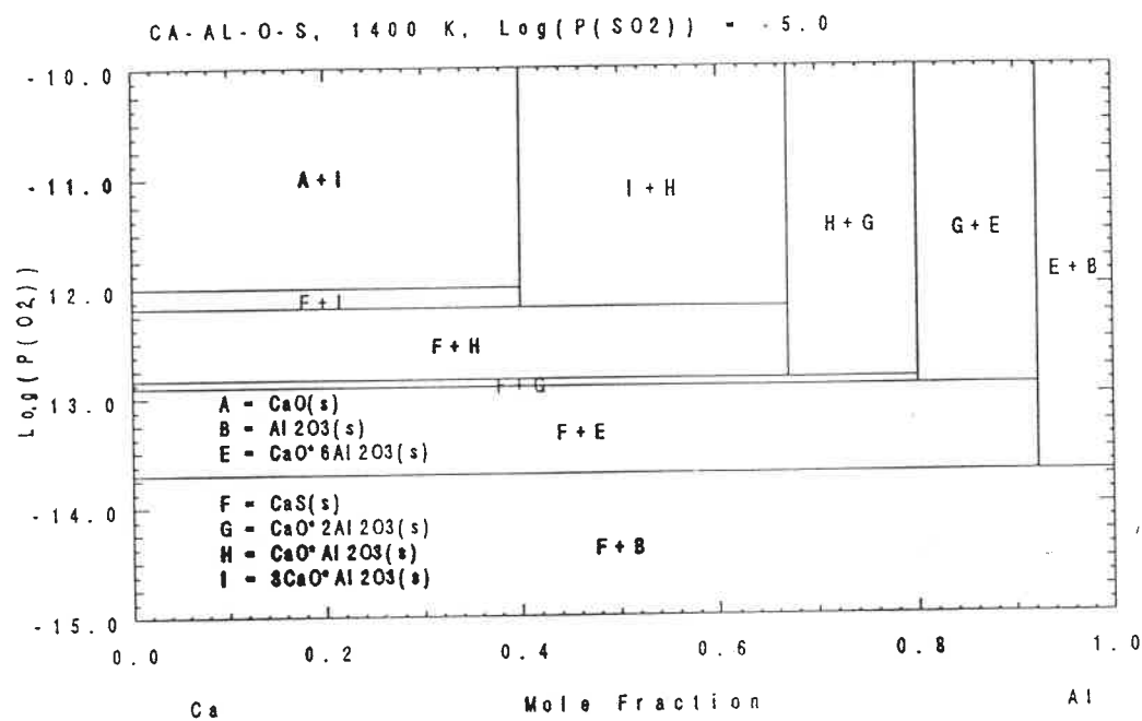
Figure 59. POTCOMP diagram for the Ca-Al-O-S system
