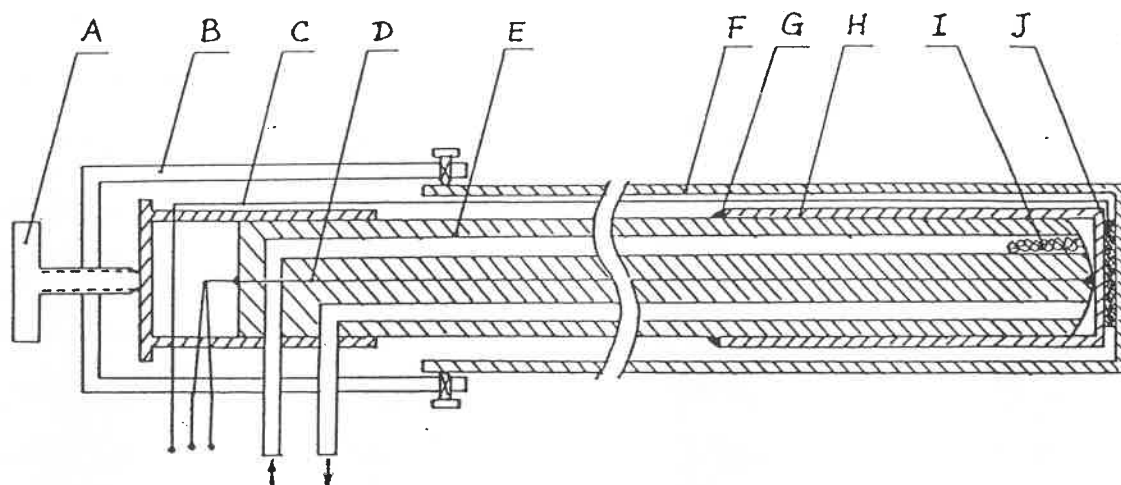
A. Set screw; B. Aluminium guide; C. Silver wire; D. Pt-10%Rh, Pt thermocouple; E. 4 bores alumina tube; F. Alumina support tube; G. Cement; H. Ag-Beta-alumina; I. Platinum wire; J. Silver plate.
