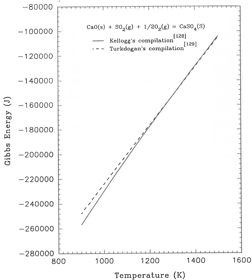
Figure 3.15 Comparison of Standard Gibbs energy for \text{CaSO}_4 from different sources
