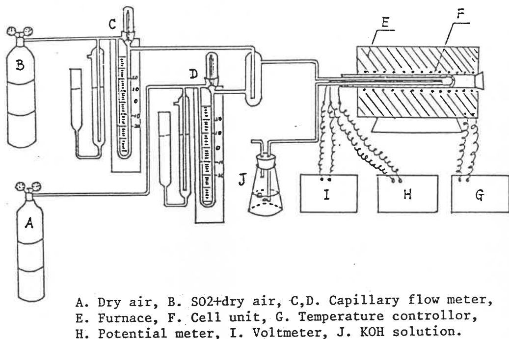
Figure 4.3 Schematic view of experimental assembly
