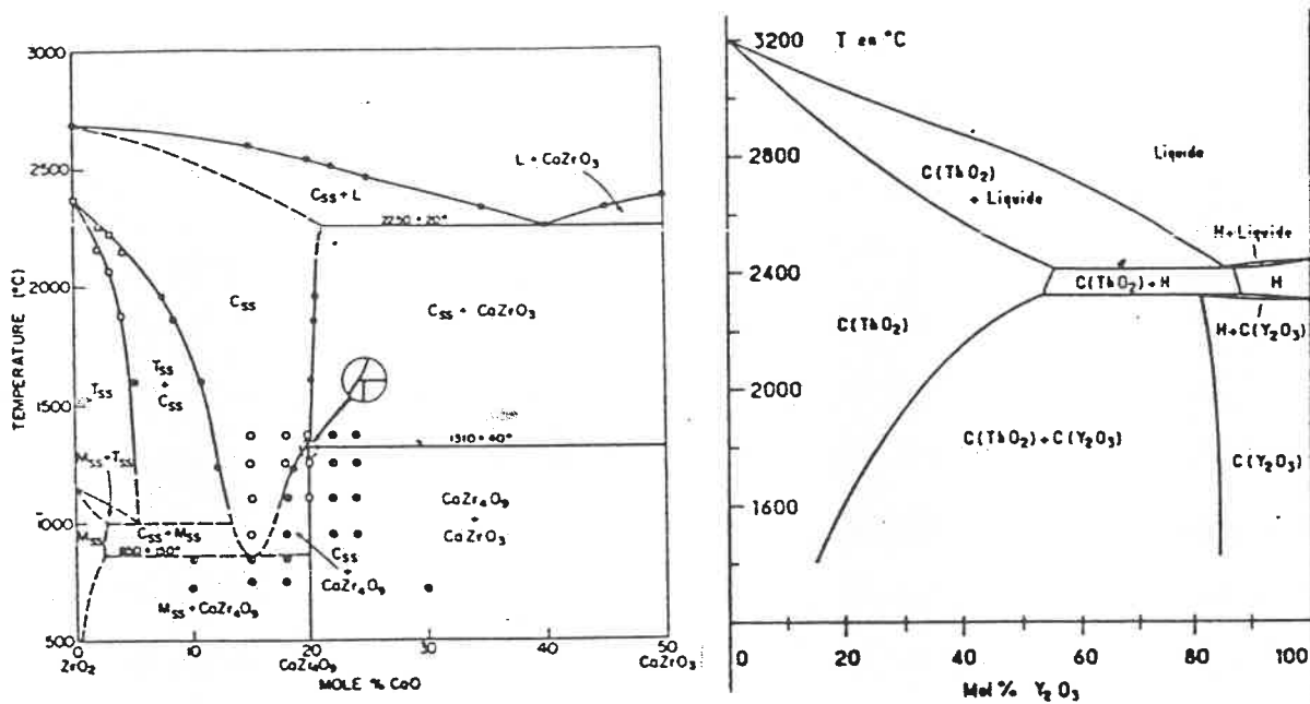
Figure 2.2 \text{ZrO}_2 -CaO and \text{ThO}_2 - \text{Y}_2\text{O}_3 phase diagrams [113, 114]
