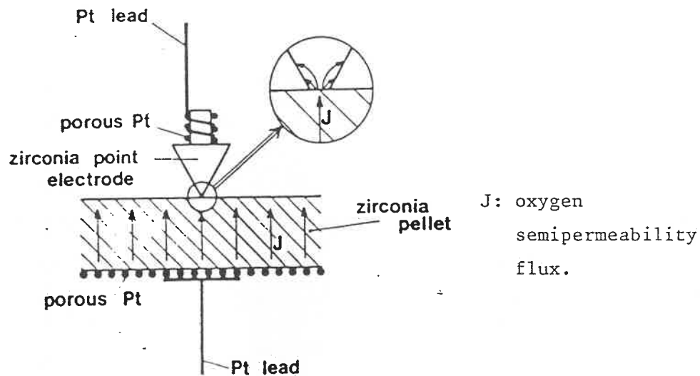
Figure 2.7 Oxygen gauge with \text{ZrO}_2 point electrode [49] .
