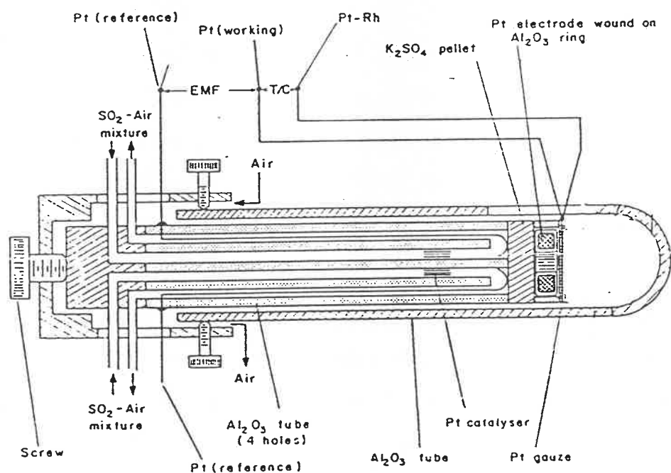
Figure 2.11 The cell using pure K 2 SO 4 (s) electrolyte [58] .
