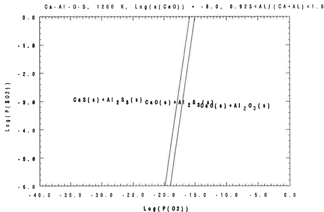
Figure 16. Predominance diagram for the Ca-Al-O-S system
