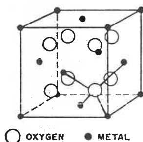
Figure 2.1 The fluorite crystal structure
