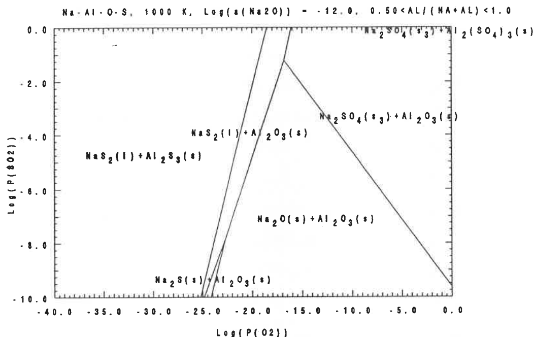
Figure 3.4 Predominance diagram for the Na-Al-O-S system
