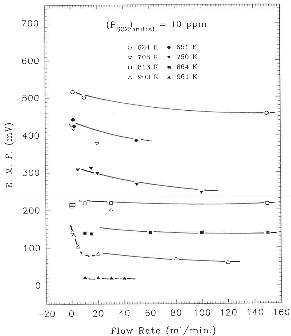
Figure 7 EMF Dependence on Flow Rate for Type 3 Electrode Preparation
