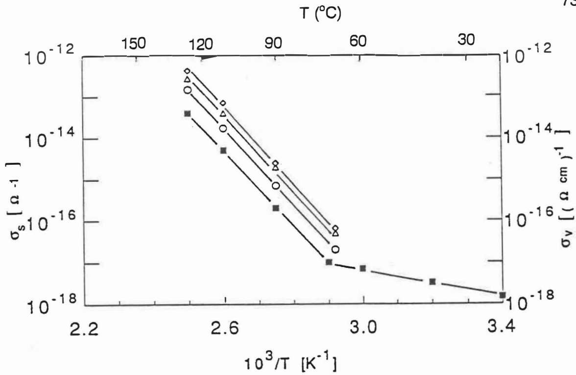
Fig. 4.10 Surface and bulk conductivities as a function of reciprocal temperature. ( \blacksquare ) \sigma_v : PET, ( \circ ) \sigma_s : P-SiN/PET, ( \Delta ) \sigma_s : PET, ( \diamond ) \sigma_s : P-SiO 2 /PET.
