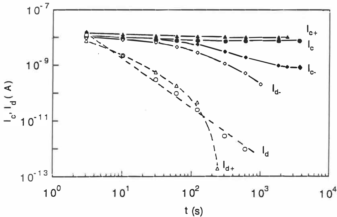
Fig.4.3 Charging I_c (●, ▲, ◆), and discharging I_d (○, △, ◇) currents as a function of time for PI and for P-SiO 2 /PI at 120°C. PI ( I_c : ●, I_d : ○), P-SiO 2 (+)/PI ( I_{c+} : ▲, I_{d+} : △), P-SiO 2 (-)/PI ( I_{c-} : ◆, I_{d-} : ◇).
