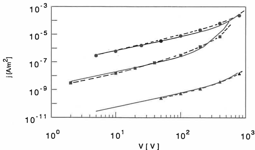
Fig.6.2 Comparison of measured (---: \Delta , \blacksquare , \bullet ) and calculated (—) bulk current densities as a function of applied voltage for PI at 24°C ( \Delta ) and at 120°C ( \bullet ), and for PET at 90°C ( \blacksquare ).
