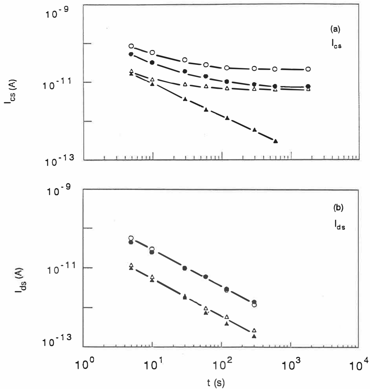
Fig.4.8 Surface charging I_{cs} (a) and discharging I_{ds} (b) currents as a function of time at 25°C before heating using 100 V. ○: P-SiO 2 /PET in atmosphere (RH = 50%), ●: P-SiO 2 /PET in vacuum ( 10^{-5} Torr), △: P-SiN/PET in atmosphere (RH = 50%), ▲: P-SiN/PET in vacuum ( 10^{-5} Torr).
