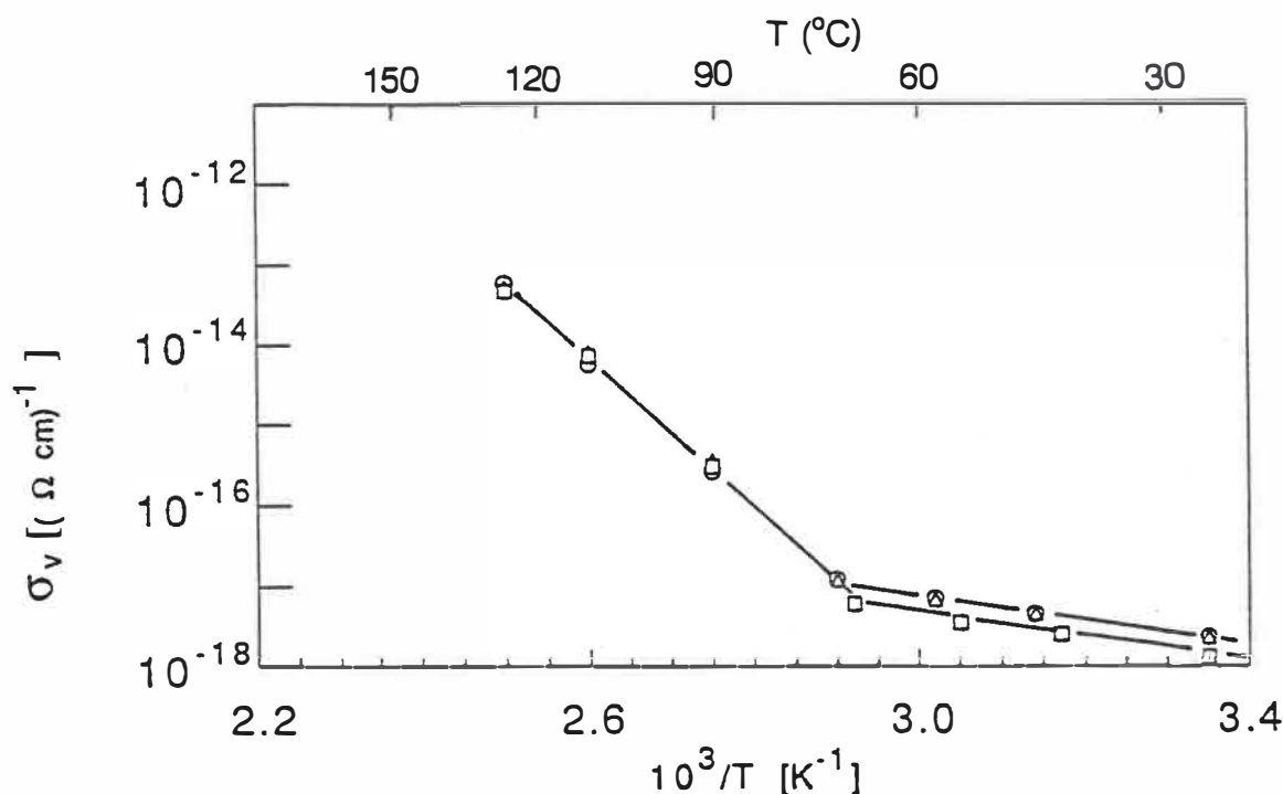
Fig.4.7 Bulk conductivity as a function of reciprocal temperature for PET (○), P-SiO 2 /PET (Δ), and P-SiN/PET (□) using E=8.3 \times 10^4 V/cm.
