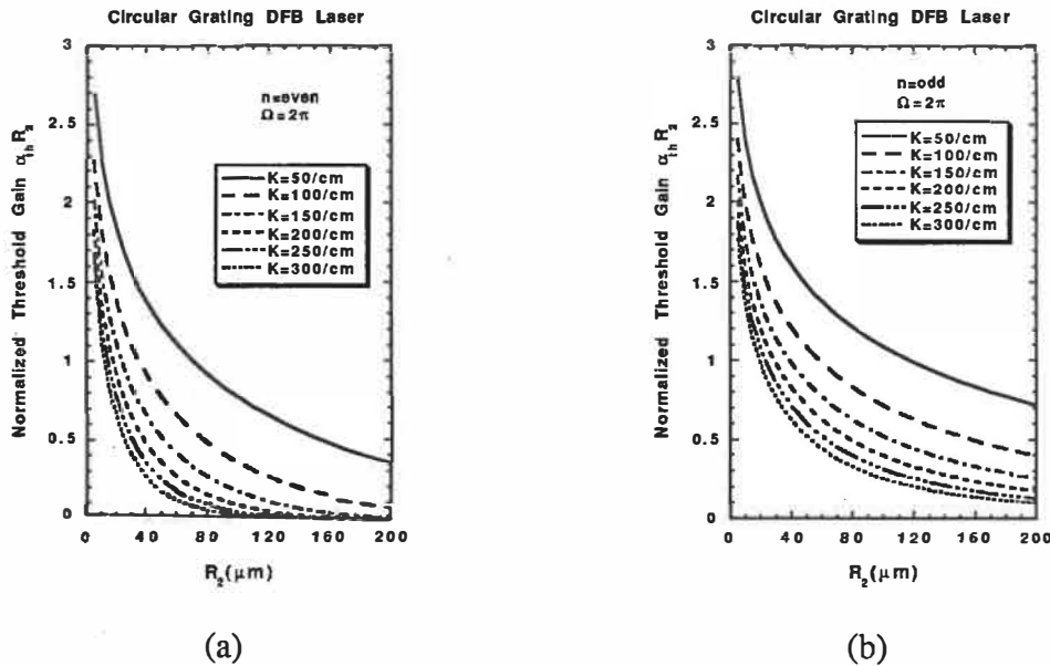
Fig.15 Normalized threshold gain of CG-DFB laser as a function of grating radius R_2 with the coupling coefficient as a parameter : (a) n=\text{even} ; (b) n=\text{odd} .
