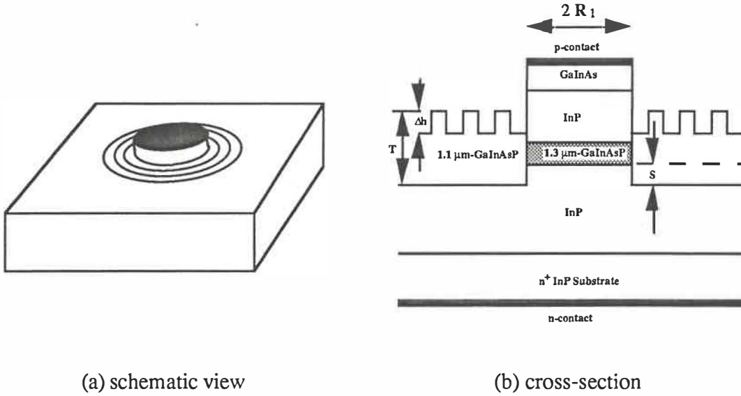
Fig.3.2 Diagram of electrically-pumped circular grating (CG) DBR laser.
