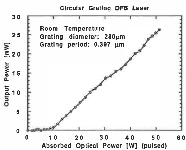
Fig.31 Surface-emitted power against pumping power.
