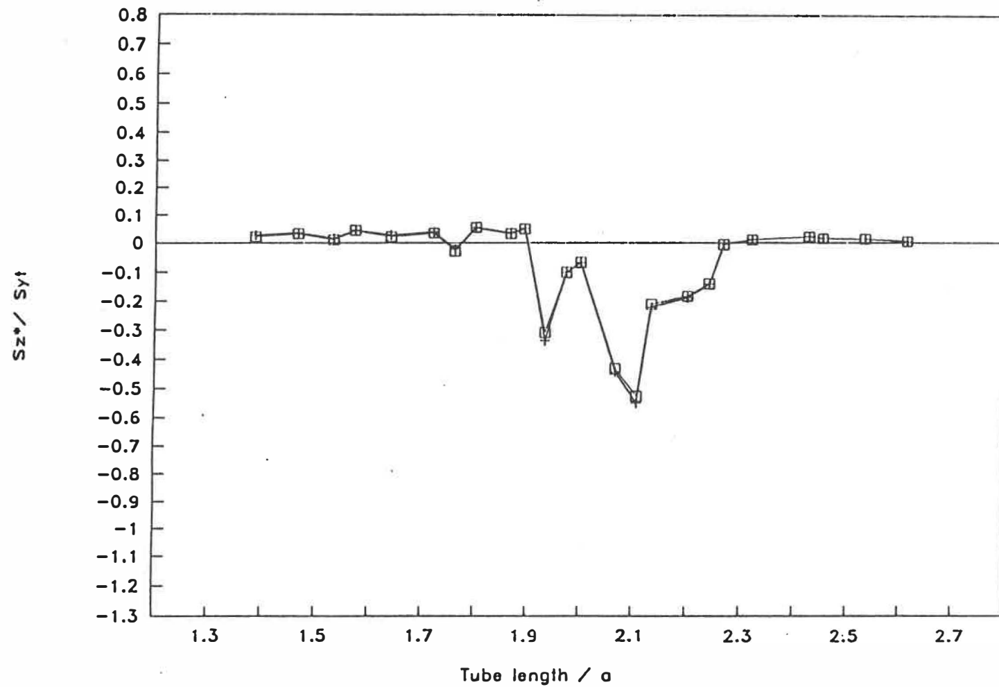
Figure 2.11 c) Residual axial stress ( outer surface of tube)
