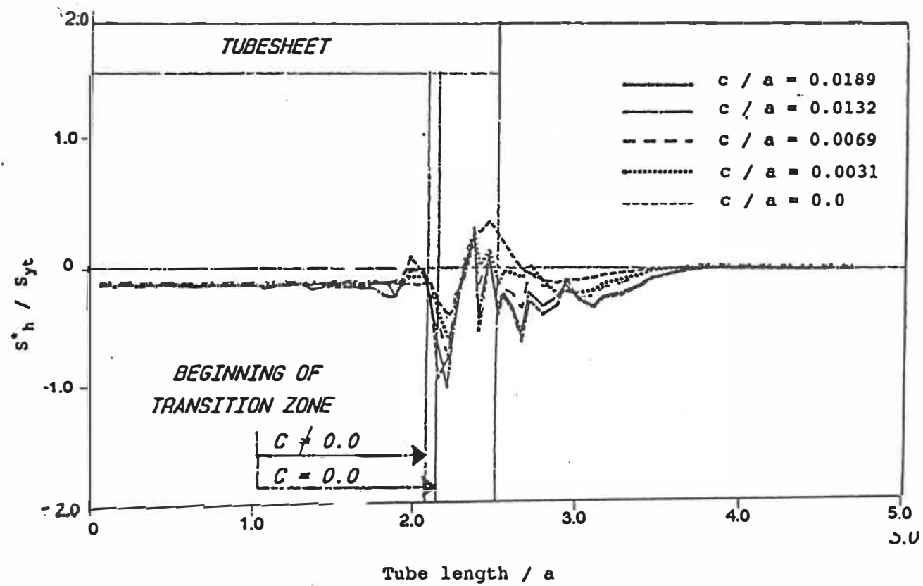
Figure 3.1 (con't) d) Hoop residual stress at outer surface of the tube.
