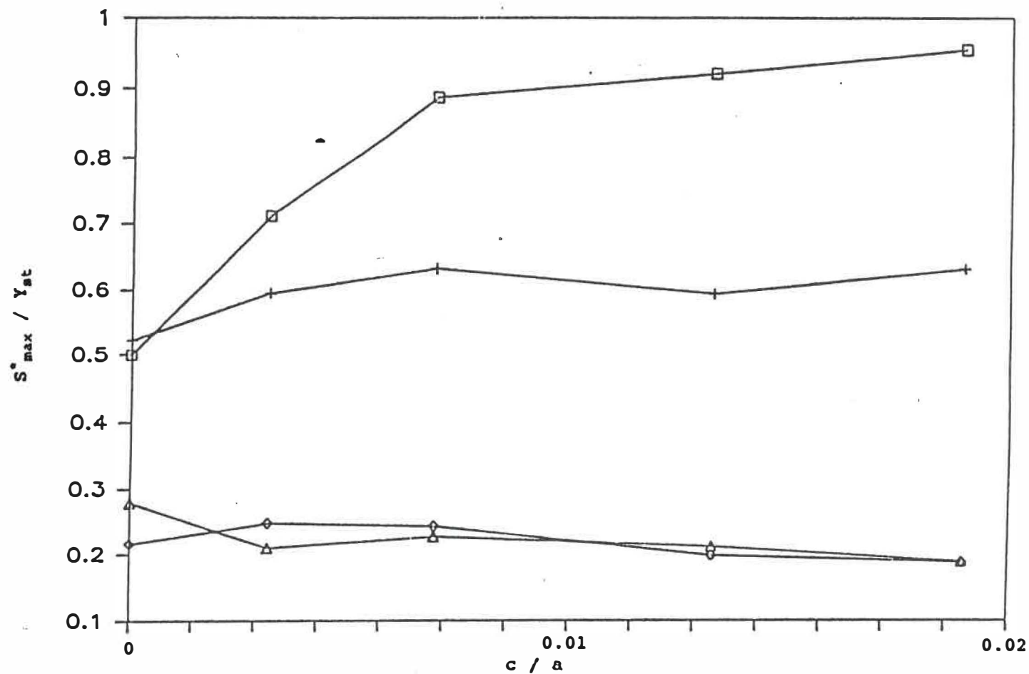
Figure 3.2 Effect of initial clearance on maximum tensile residual stresses in transition zone
