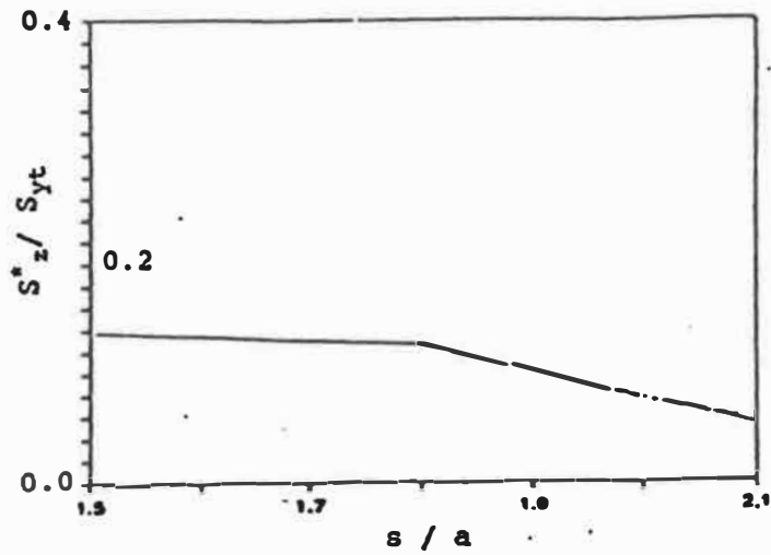
Figure 3.5 (con't) d) Axial residual stress at outer surface (maximum tensile)
