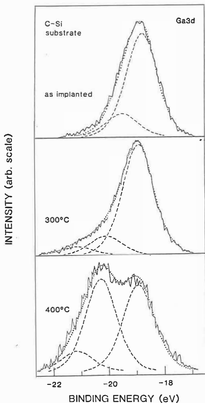
Figure 4.5: Ga3d core level spectra measured on c-Si samples, as-implanted, and annealed at 300 and 400 °C. The experimental signals are shown by solid line. The dashed curves show the results of deconvolution into different components and the dots are the sums of the components. Intensities are shown on an arbitrary scale.
