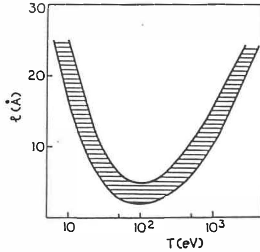
Figure 2.2: Kinetic energy dependence of the mean free path of electrons in solids. The shaded area corresponds to the region occupied by the actual experimental points for most materials (from Margaritondo and Weaver (1985)).
