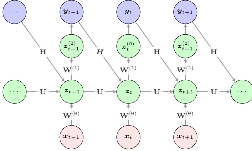
Figure 2.10 The teacher forcing setup for RNN where the output-to-hidden recurrent connection is defined between the observations \mathbf{y}_{t-1} and the hidden states \mathbf{z}_t .
