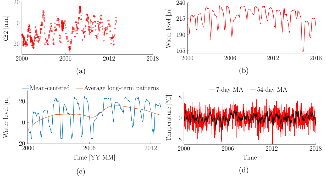
Figure 2.2 Dataset from the international Benchmark Workshop organized by the International Commission of Large Dams (ICOLD) [11], (a) inverted pendulum, (b) raw reservoir's water level, (c) components extracted from the raw reservoir's water level, and (d) moving-averages for air temperature.
