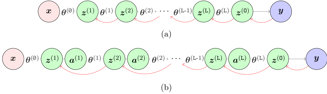
Figure 3.5 Layer-wise inference procedure to update the hidden states for a feedforward neural network (a) without, and (b) with activation units shown explicitly. Black arrows represent the network forward connections, red arrows represent the layer-wise inference paths.
