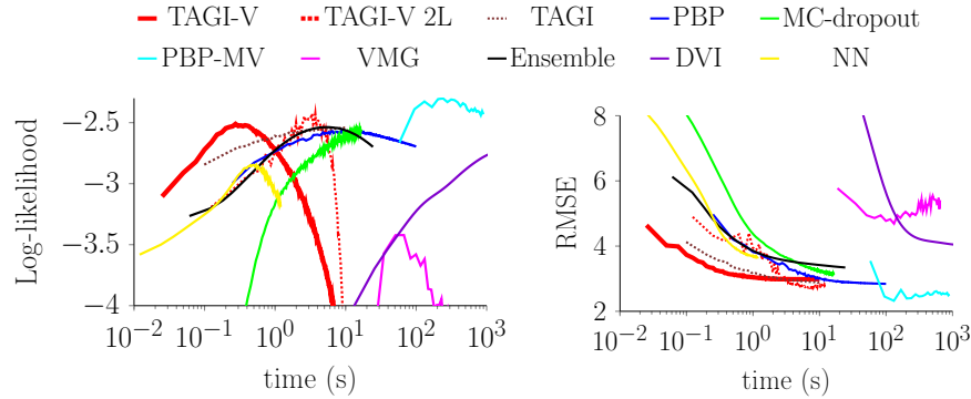
Figure 2.15 Comparison for the test log-likelihood and test RMSE for the Boston dataset among various Bayesian neural network methods. The figures are reused from [13].
