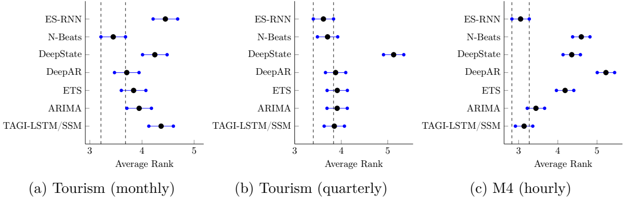
Figure 4.5 Average ranks and 95% confidence intervals for all methods over all time series in each dataset based on the multiple comparisons with the best (MCB) test using the p50 metric. Dashed lines present 95% confidence intervals for the best method.
