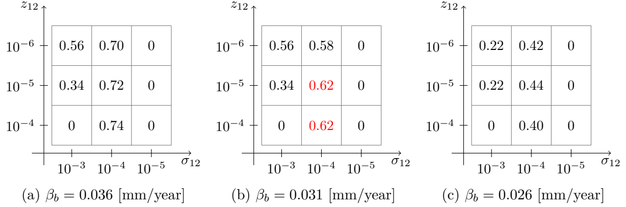
Figure 5.21 Case study #3: crack opening. Probability of detection for different anomaly's slopes.
