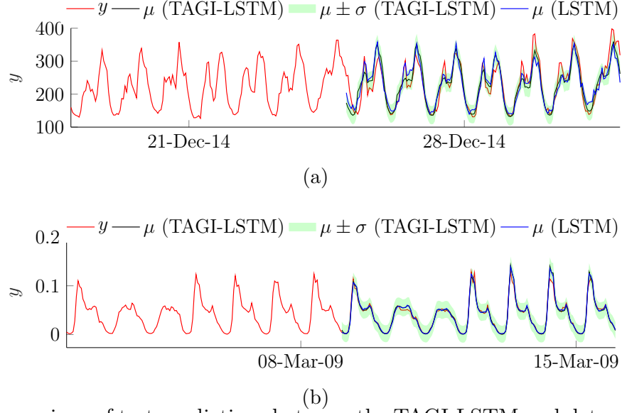
Figure 3.9 Comparison of test predictions between the TAGI-LSTM and deterministic LSTM models for a time series in (a) Electricity, and (b) Traffic datasets. The \pm\sigma regions contain both the epistemic (parameter's) uncertainties obtained from the prior predictive distribution of z^{(0)} as well as the aleatory uncertainties associated with the error term's variance \sigma_V^2 . Only a part of the training set is presented.
