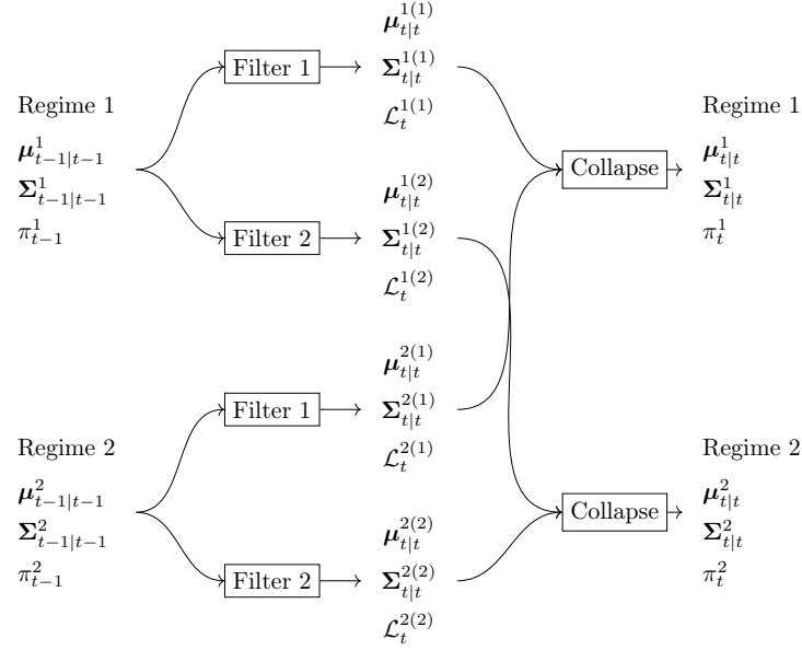
Figure 2.5 Switching Kalman Filter filtering and collapse steps for a case involving two regimes. The number of models increases from 2 to 4 after the filtering step, while the collapse step reduces and keeps 2 models at each time.
