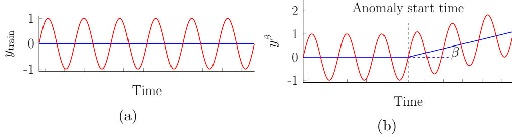
Figure 5.1 Introduction of synthetic anomaly. (a) anomaly-free training time series and (b) time series with synthetic anomaly. The blue line represents the baseline of the data.
