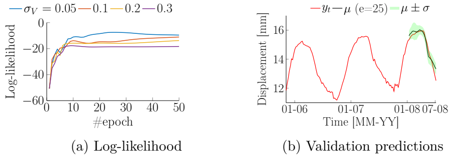
Figure 5.15 Case study #2: dam's displacement. Log-likelihood and multi-step-ahead predictions for the validation set.
