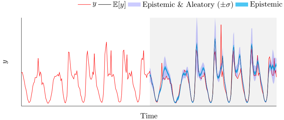
Figure 3.10 Example of learning the time-varying aleatory uncertainty ( \sigma_V ) estimated using the AGVI method [8] for a time series in the traffic dataset. The grey shaded area presents the test set, and only a part of the training set is presented.
