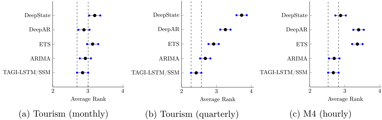
Figure 4.6 Average ranks and 95% confidence intervals for all methods over all time series in each dataset based on the multiple comparisons with the best (MCB) test using p90 metric. Dashed lines present 95% confidence intervals for the best method.
