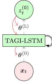
Figure 4.1 The nonlinear transition function for the pattern hidden states is modelled by a TAGI-LSTM network. Red arrows represent the layer-wise inference paths for inferring the posterior knowledge for the TAGI-LSTM's hidden states and parameters from the posterior PDF of the pattern hidden state Z^{(0)} . Black arrows represent the network forward connections, and double arrows represent the recurrent connections.
