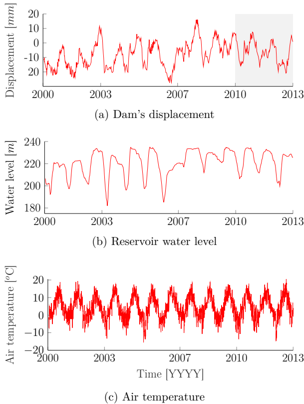
Figure 4.11 Data from a dam in southern France
