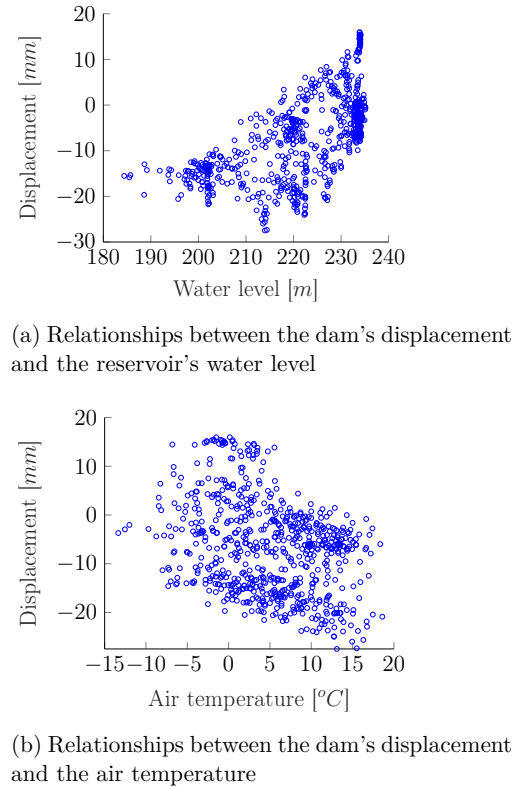
Figure 4.12 Relationships between the dam's displacement and environmental variables.
