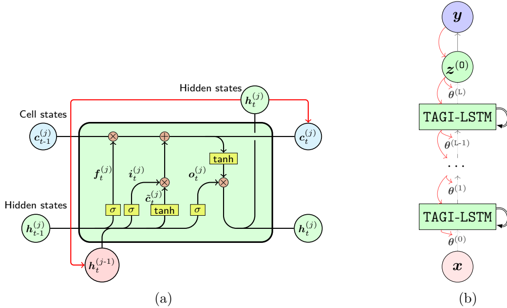
Figure 3.1 (a) Graphical representation of a LSTM cell. Red arrows represent the inference procedure to update the j - 1^{th} LSTM layer from the subsequent j^{th} LSTM layer. (b) Graphical representation of a stacked TAGI-LSTM network. Black arrows represent the network's forward connections, red arrows represent the layer-wise inference paths, and double arrows represent the recurrent connections.
