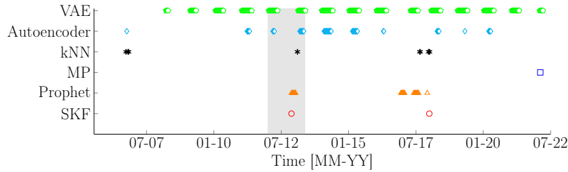
(c) Comparison with others anomaly detection methods
