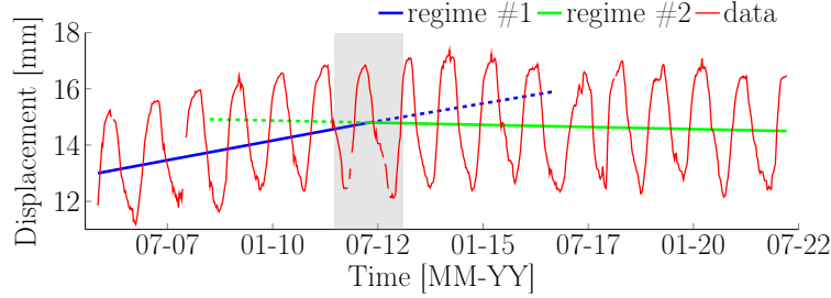
Figure 5.14 Case study #2: dam's displacement. Preliminary analysis to identify visually possible anomalies where the grey shaded area presents the regime switch quantitatively. The dash line with a corresponding colour presents the extension for the regime identified.
