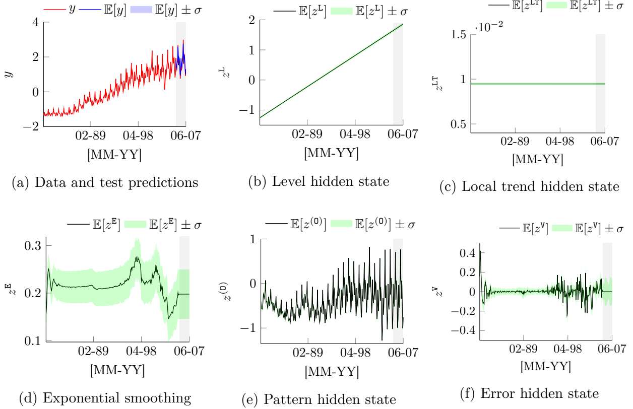
Figure 4.4 An example of interpretable results for the time series #36 of the Tourism (monthly) dataset. Values are presented in standardized space. Red line presents observations, blue line presents test predictions, black lines present components along with \pm\sigma confidence intervals (shade). The grey shaded areas present the forecast period. The \pm\sigma regions in (a) contain both the epistemic (parameter’s) uncertainties obtained from the prior predictive distributions of the hidden states as well as the aleatory uncertainties associated with the error term’s variance \sigma_V^2 .
