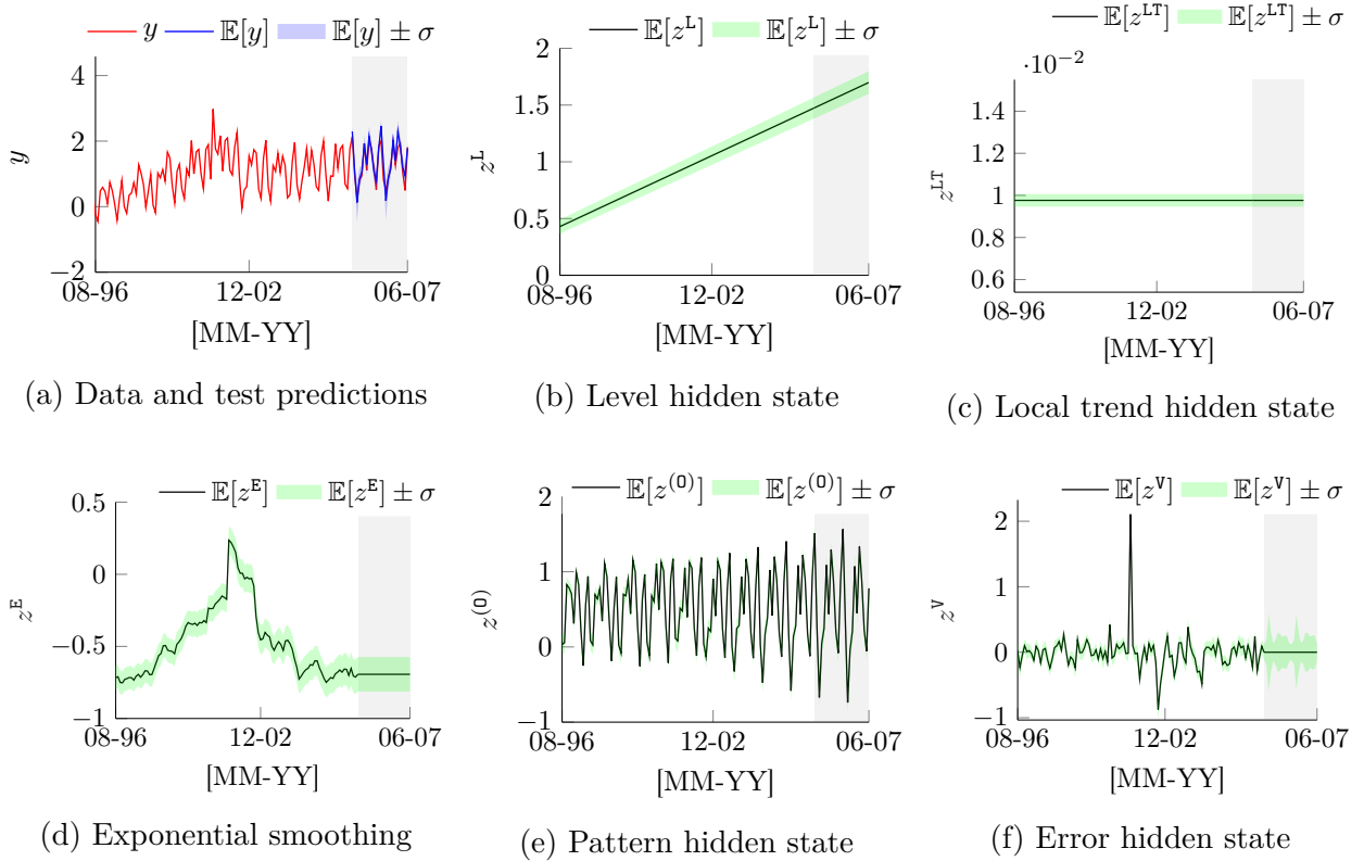
Figure 4.3 An example of interpretable results provided by TAGI-LSTM/SSM using the proposed exponential smoothing component for the time series #30 of the Tourism (monthly) dataset. Values are presented in standardized space. Red line presents observations, blue line presents test predictions, black lines present components along with \pm\sigma confidence intervals (shade). The grey shaded areas present the forecast period. The \pm\sigma regions in (a) contain both the epistemic (parameter's) uncertainties obtained from the prior predictive distributions of the hidden states as well as the aleatory uncertainties associated with the error term's variance \sigma_V^2 .
