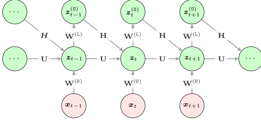
Figure 2.9 The time-unrolled representation of a single-hidden-layer RNN. The arrows depict the casual direction or casual relationship between variables as described in Equation 2.12.
