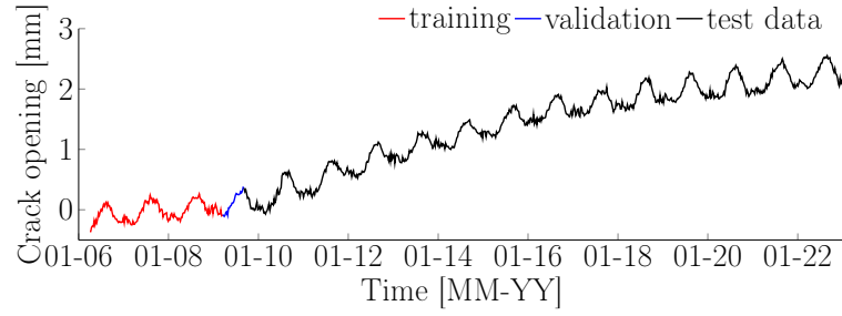
(a) Crack opening
