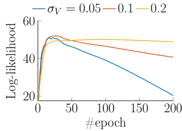
(a) Log-likelihood
