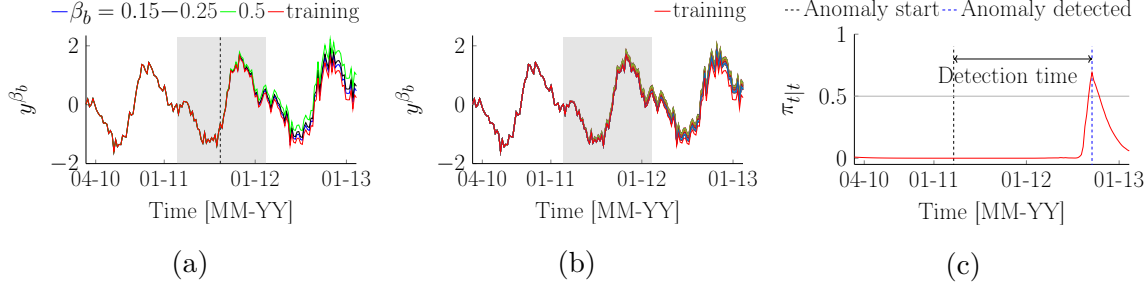
Figure 5.5 (a) Three time series with anomalies of different slopes introduced at the same time step, (b) 50 time series with anomalies of the same slope \beta_b = 0.25 [mm/year] but introduced at different time steps, and (c) the probability of anomaly \pi_{t|t} and detection time for one synthetic time series. The dashed line presents the anomaly's start time, the shaded grey area presents the period where anomalies are randomly introduced with different start times.
