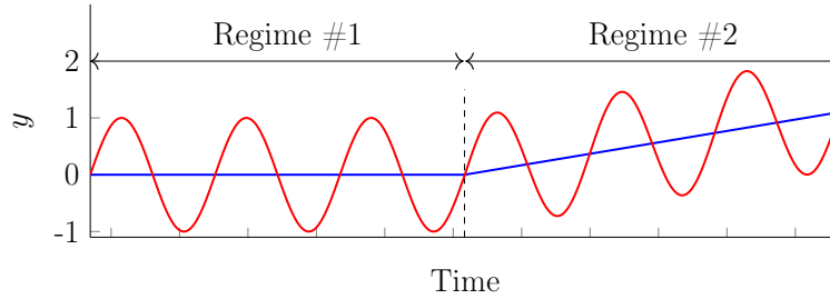
Figure 2.4 Time series with two regimes where the first one has a constant trend and the second one has a linear positive trend. The blue line presents the baseline.
