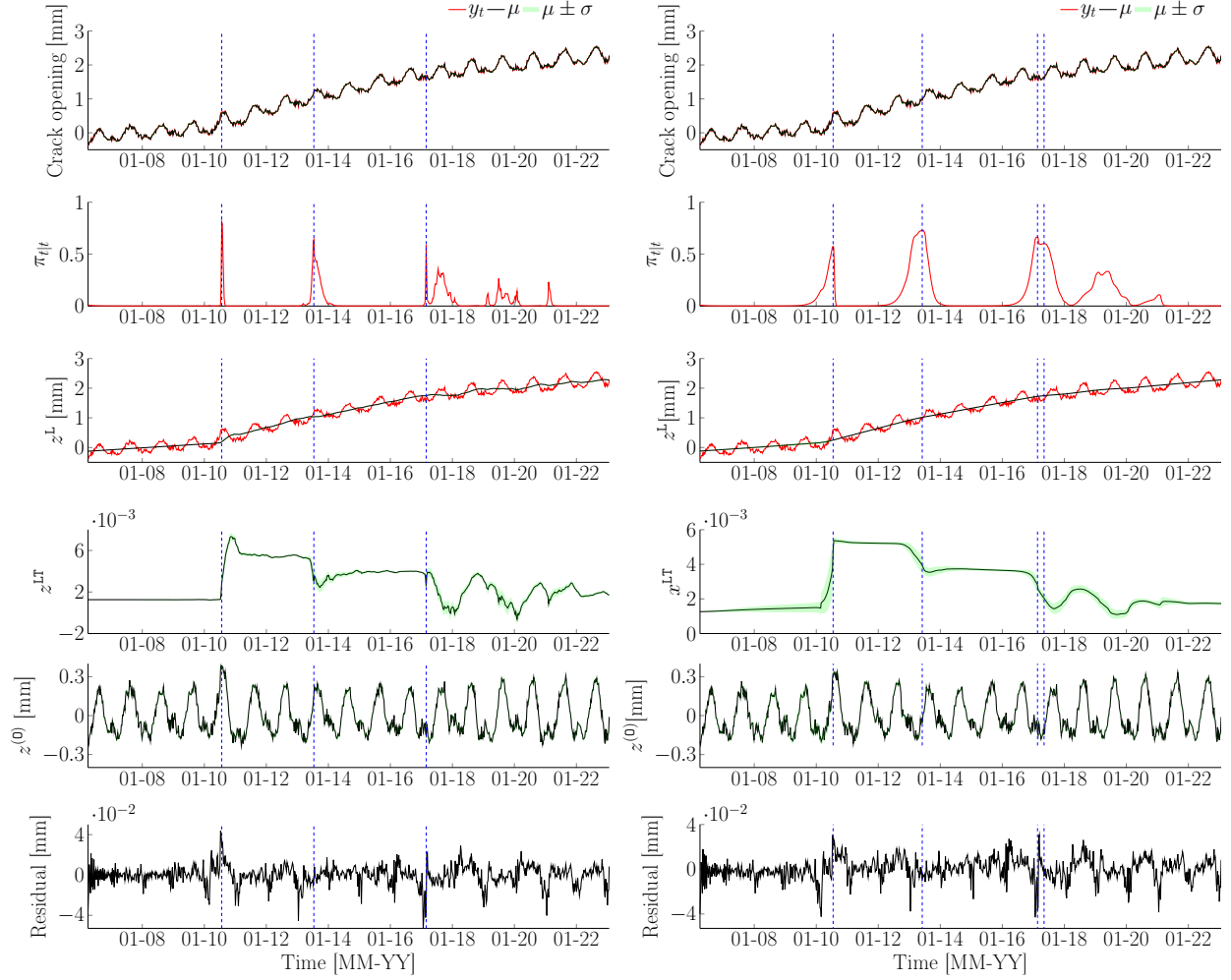
(a) Switching Kalman Filter results
