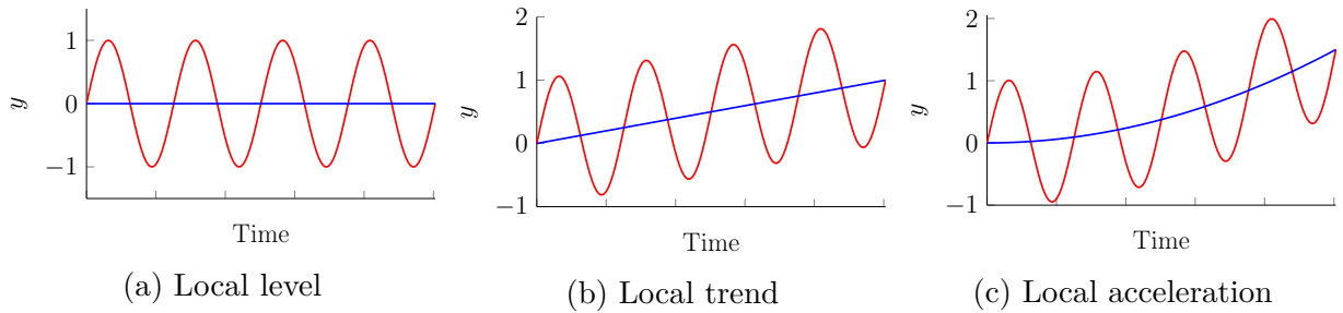
Figure 2.1 Three synthetic time series having different baselines, but sharing the same periodic pattern. The red line presents the data, while the blue line presents the baseline.
