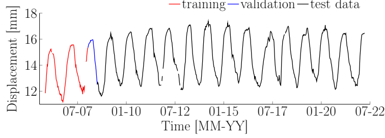
Figure 5.13 Case study #2: displacement data from a dam in Canada.
