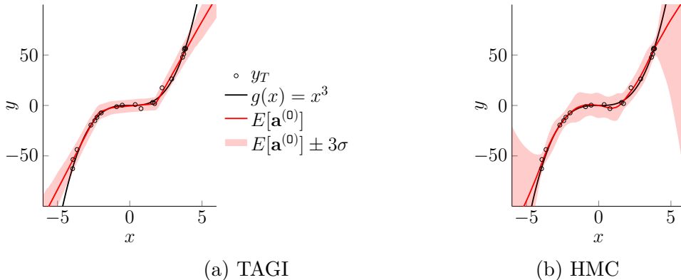
Figure 2.17 Comparison between TAGI with diagonal covariance structures and Hamiltonian Monte-Carlo (HMC) for a 1D regression problem y = x^3 + v . Re-used from [12].
