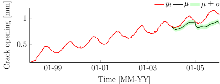
Figure 3.11 Test predictions from the TAGI-LSTM trained using the original trended data. The \pm\sigma regions contain both the epistemic (parameter's) uncertainties obtained from the prior predictive distribution of z^{(0)} as well as the aleatory uncertainties associated with the error term's variance \sigma_V^2 .
