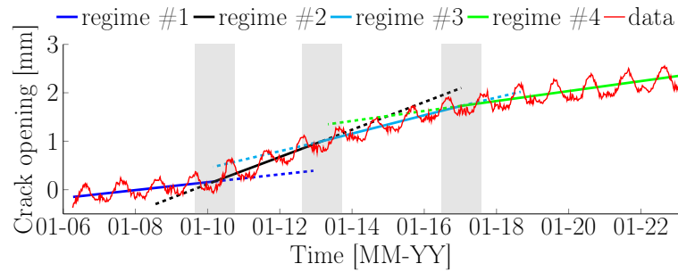
Figure 5.19 Case study #3: crack opening. Preliminary analysis to identify visually possible anomalies where the grey shaded area presents the regime switch quantitatively. The dash line with a corresponding colour presents the extension for the regime identified.
