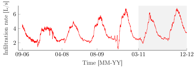
Figure 4.7 Water infiltration rate from a concrete dam in Canada. The grey shaded area presents the forecast period.
