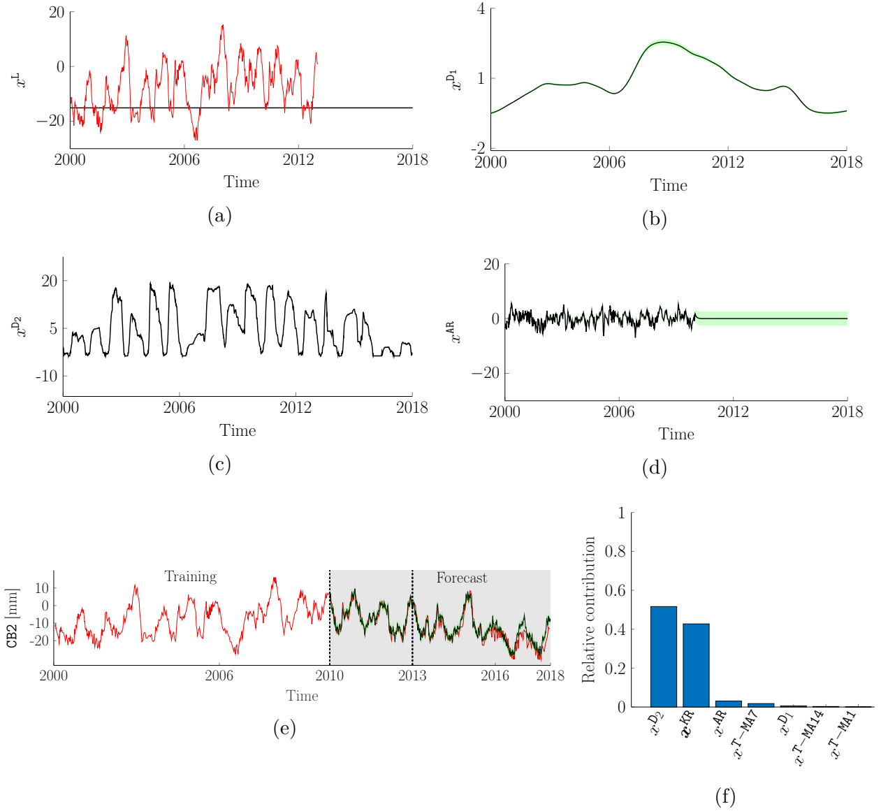
Figure 2.3 Hidden state estimation from BDLM model for the CB2 pendulum dataset, (a) level component, (b) contribution of the water level's average long-term trend x^{WL,2} of the water level, (c) contribution of the water level's mean-centered component x^{WL,1} , (d) autoregressive component, (e) predictions on the validation and test sets, (f) relative importance of each component. The figures are reused from [6].
