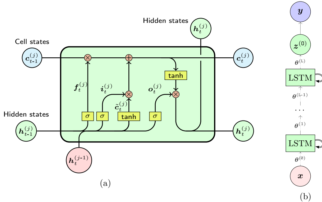
Figure 2.13 (a) The representation of a LSTM cell, and (b) the compact form of a stacked LSTM where single-line arrows present forward connections, and double-line arrows represent the recurrent connections.
