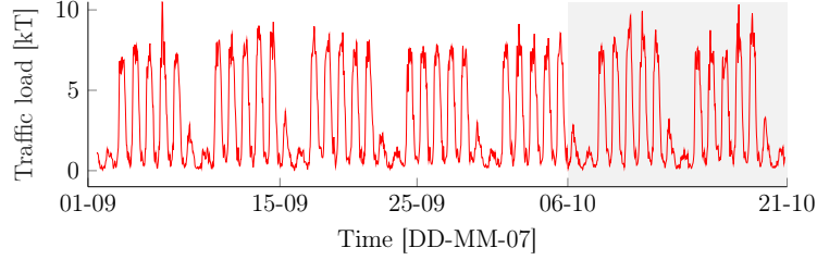
Figure 4.9 Traffic load data on the Tamar bridge in the UK. The grey shaded area presents the forecast period.
