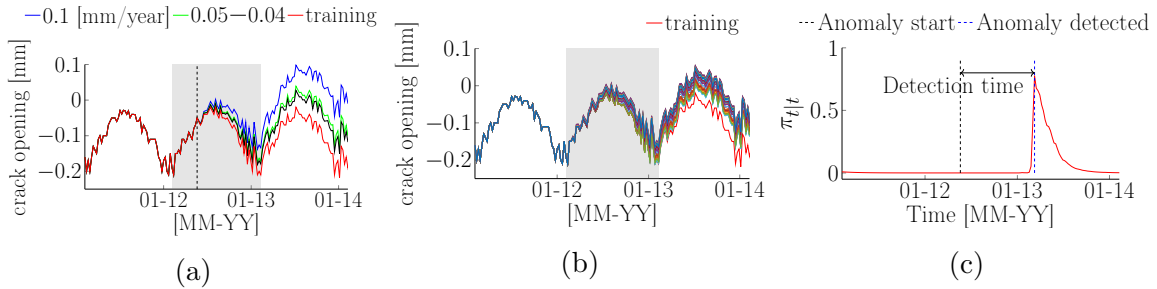
Figure 5.10 Case study #1: crack opening. Synthetic time series (a) with anomalies of different slopes introduced at the same time step, (b) with 50 anomalies of the same slope introduced at different time steps, and (c) the probability of anomaly \pi_{t|t} and detection time for one synthetic time series. The shaded grey area presents the period where synthetic anomaly is randomly added.
