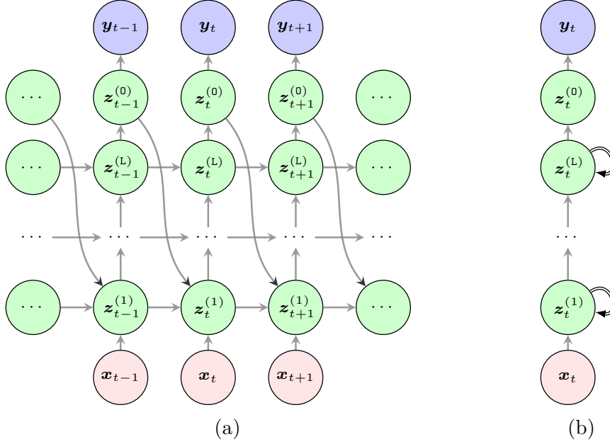
Figure 2.12 (a) Time-unrolled, and (b) compact representation of a stacked RNN where the double line arrow represents recurrent connections. Note that for the first hidden layer, the double arrow implies the both hidden-to-hidden and output-to-hidden recurrent connections, where for other hidden layers it implies only the hidden-to-hidden connection.
