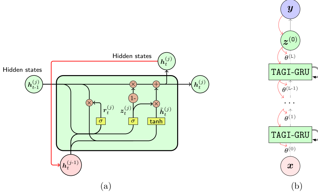
Figure 3.4 (a) Graphical representation of a GRU cell. Red arrows represent the inference procedure to update the j - 1^{th} GRU layer from the subsequent j^{th} GRU layer. (b) Graphical representation of a stacked TAGI-GRU network. Black arrows represent the network's forward connections, red arrows represent the layer-wise inference paths, and double arrows represent the recurrent connections.
