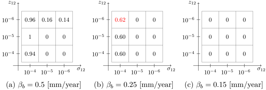
Figure 5.6 Detection probability p^{\beta_b} for detecting anomalies with different slope \beta_b in the simulated time series for models with different sets \mathcal{P}_k .
