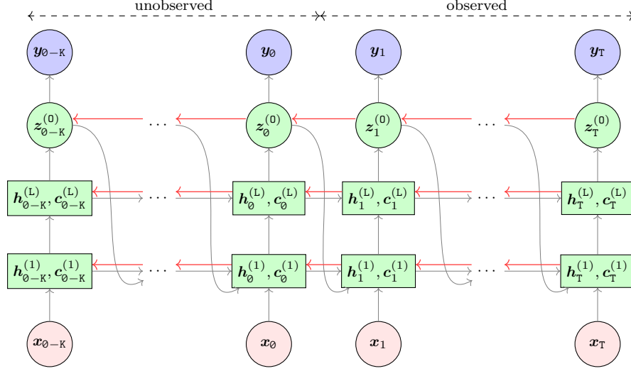
Figure 3.3 Time-unfolded representation of a TAGI-LSTM network with explicit connections between times steps. Black arrows represent the network forward connections, red arrows represent the smoothing procedure. The observed data includes training data, whereas the unobserved one is data K time steps before the first training time step. This smoothing procedure allows to infer not only the smoothed estimates for hidden and cell states, and output during training time steps, but also the past ones before the training history.
