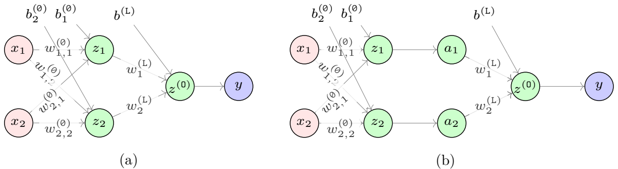
Figure 2.7 Equivalent representations of a single-hidden-layer fully connected feedforward neural network where (a) only the hidden states \mathbf{z} , and (b) both hidden states \mathbf{z} and activations units \mathbf{a} are shown.
