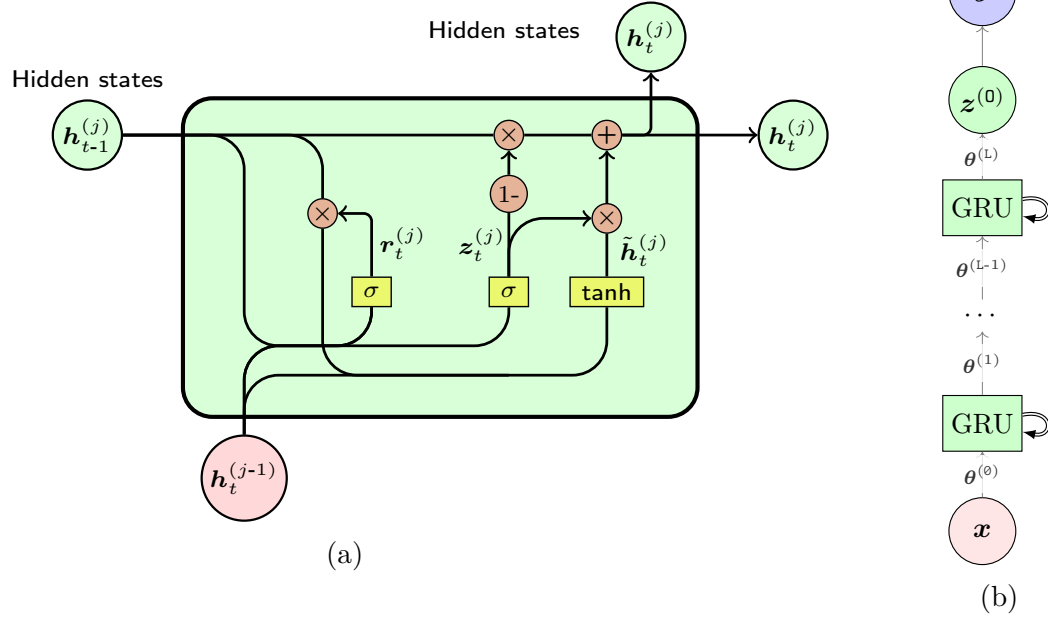
Figure 2.14 (a) GRU cell, and (b) compact representation of a stacked GRU where the double line arrow represents recurrent connections.
