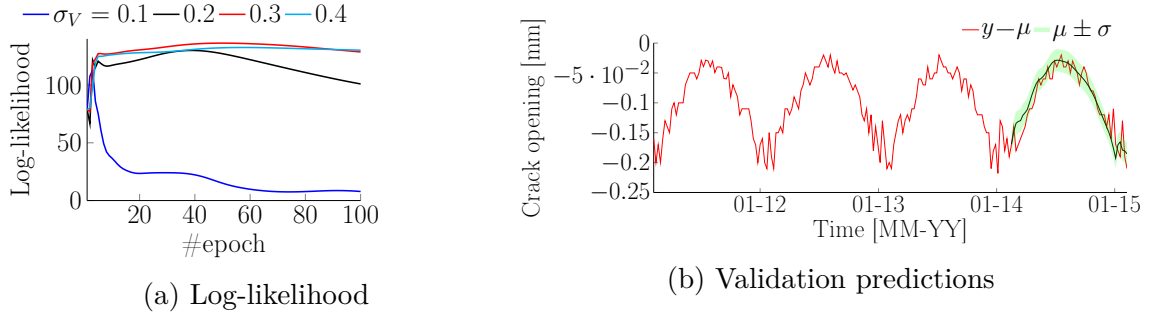
Figure 5.9 Case study #1: crack opening. Log-likelihood and multi-step-ahead predictions for the validation set. The \pm \sigma regions contain both the epistemic (parameter's) uncertainties obtained from the prior predictive distributions of the hidden states as well as the aleatory uncertainties associated with the error term's variance \sigma_V^2 .
