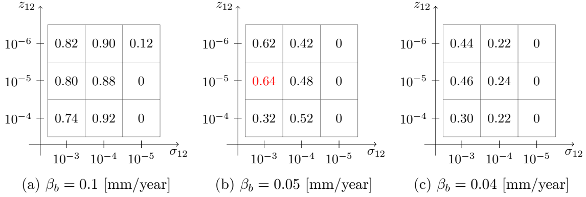
Figure 5.11 Case study #1: crack opening. Probability of detection for different anomaly's slopes.
