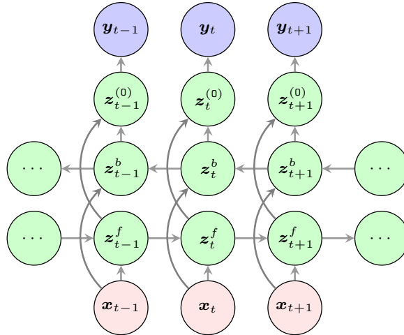
Figure 2.11 Time-unrolled representation of a bidirectional RNN where two separate RNN models are employed at the same time, one moves forward and the another moves backward in time.
