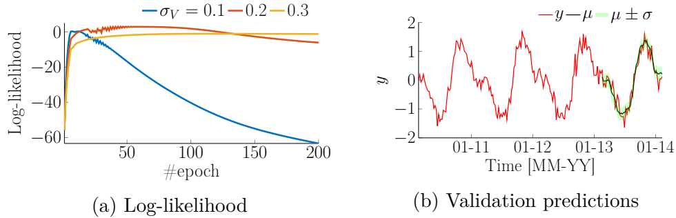
Figure 5.3 Experiment with synthetic data. Log-likelihood and multi-step-ahead predictions for the validation set.
