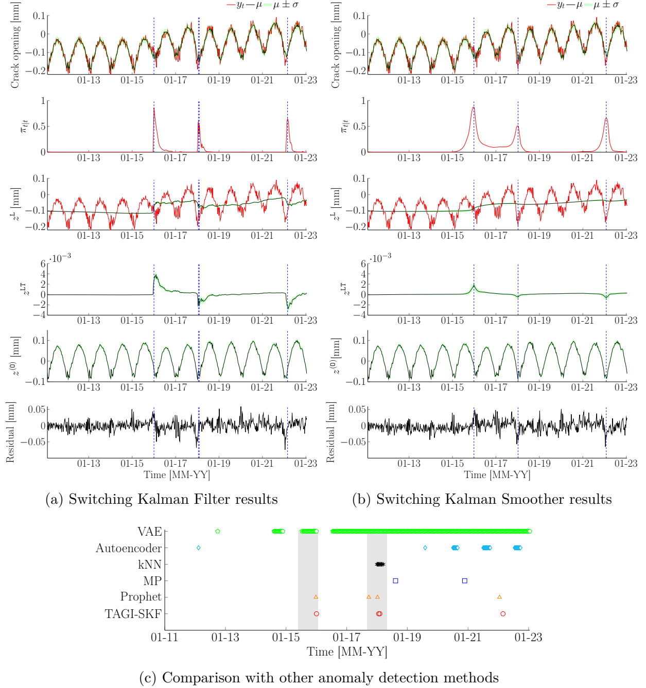
Figure 5.12 Case study #1. Anomaly detection results obtained from our method and other models. Each line of scatter points presents when the alarms are triggered for each method, and the grey shaded area presents the visually identified anomalies from the preliminary analysis. The blue dashed lines present where the anomalies are detected by our method. The \pm\sigma confidence intervals in the top row of (a) and (b) contain both the epistemic (parameter's) uncertainties obtained from the posterior predictive distributions of the hidden states as well as the aleatory uncertainties associated with the error term's variance \sigma_V^2 .
