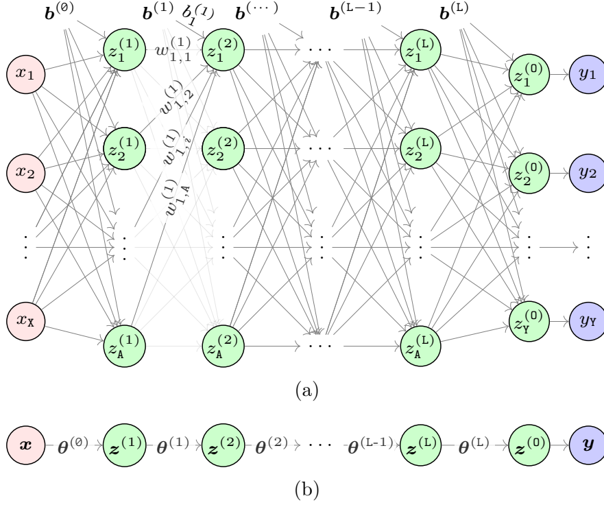
Figure 2.8 The (a) full representation of a multi-hidden-layer FNN where each node represents a unit, and the arrow between any two nodes represents the forward connection, and (b) the equivalent compact representation of the same network where each node represents a vector, and \theta = \{\mathbf{w}, \mathbf{b}\} . The figures are reproduced from [12].
