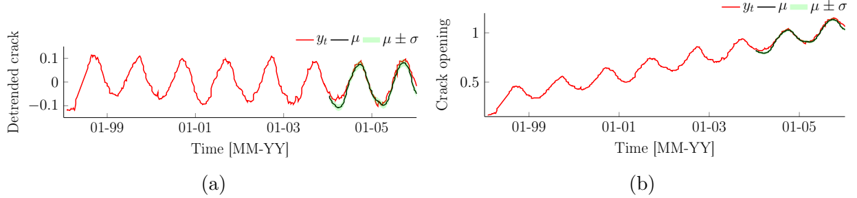
Figure 3.13 (a) The test predictions for the zero-mean recurrent pattern, and (b) the final test predictions obtained by summing up the zero-mean predictions and the trend component. The \pm \sigma regions contain both the epistemic (parameter's) uncertainties obtained from the prior predictive distribution of z^{(0)} as well as the aleatory uncertainties associated with the error term's variance \sigma_V^2 .
