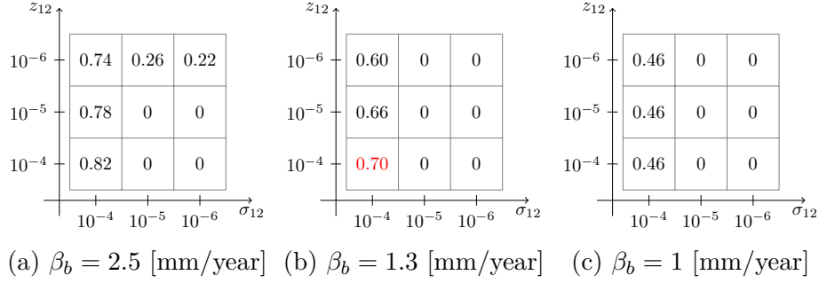
Figure 5.16 Case study #2: dam's displacement. Probability of detection for different anomaly's slopes.
