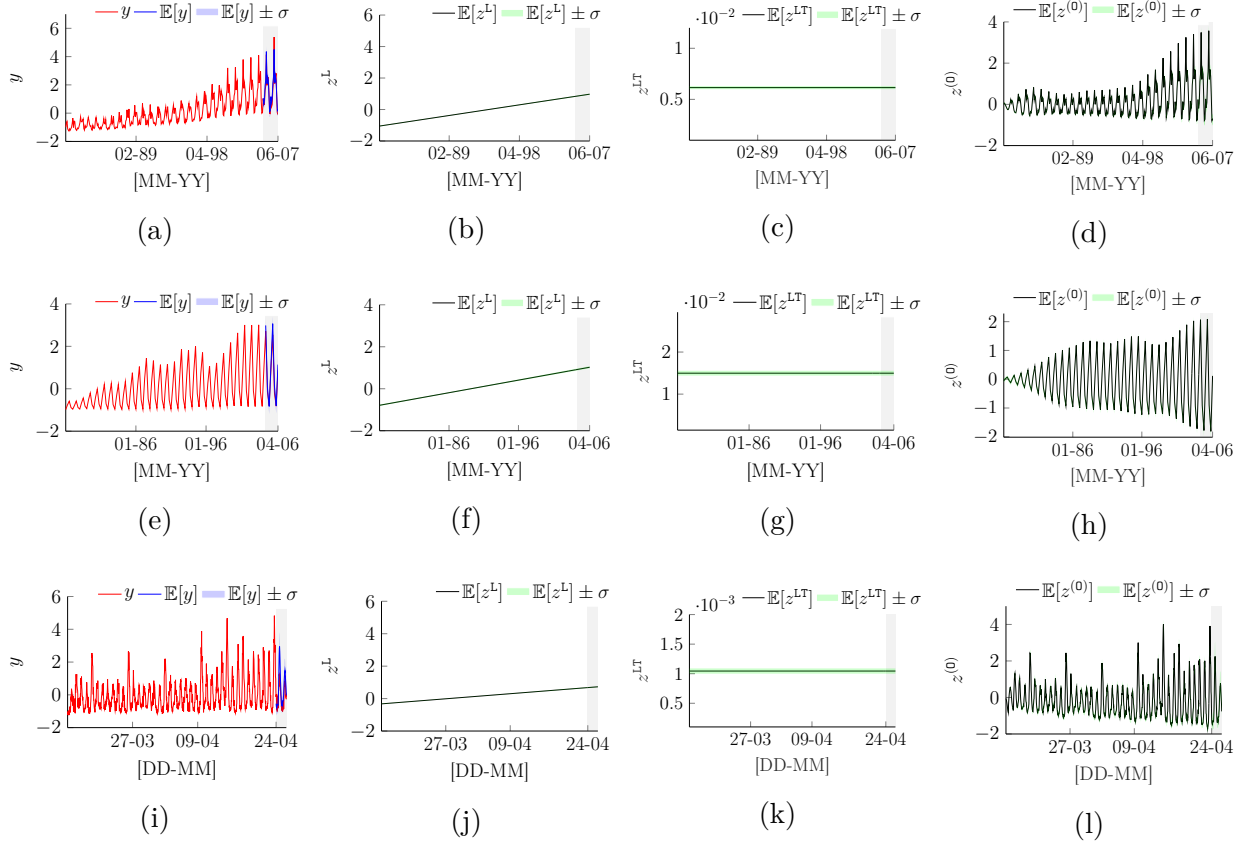
Figure 4.2 An example of interpretable results for several time series. Values are presented in standardized space. Red lines present observations, blue lines present test predictions, black lines present components along with \pm\sigma confidence intervals (shade). The grey shaded areas present the forecast period. (a) predictions on test set, (b) level, (c) trend, and (d) seasonality modelled by TAGI-LSTM for time series #32 of the Tourism (monthly) dataset. (e) predictions on test set, (f) level, (g) trend, and (h) seasonality modelled by TAGI-LSTM for time series #33 of the Tourism (quarterly) dataset. (i) predictions on test set, (j) level, (k) trend, and (l) seasonality modelled by TAGI-LSTM for time series #375 of the M4 (hourly) dataset. In (a), (e) and (i), the \pm\sigma regions contain both the epistemic (parameter's) uncertainties obtained from the prior predictive distributions of the hidden states as well as the aleatory uncertainties associated with the error term's variance \sigma_V^2 . Zoom-in figures for (a), (e) and (i) are provided in Appendix D.
