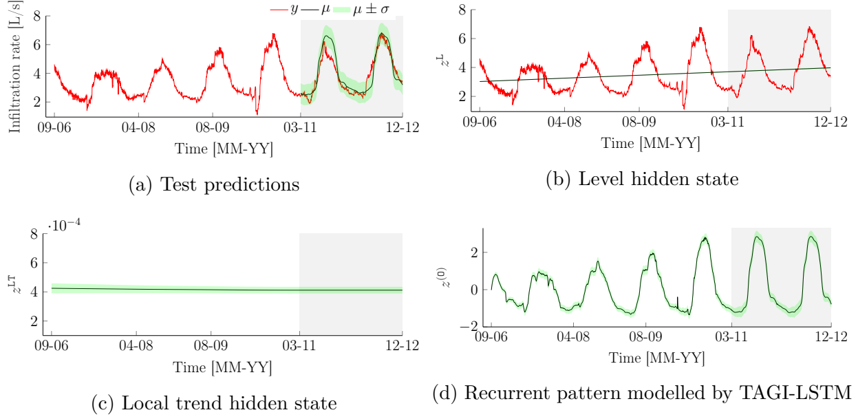
Figure 4.8 Results from our model for the water infiltration rate dataset including the test predictions, the level and local trend hidden states, and the recurrent pattern. The grey shaded area presents the forecast period. The \pm\sigma regions in (a) contain both the epistemic (parameter's) uncertainties obtained from the prior predictive distributions of the hidden states as well as the aleatory uncertainties associated with the error term's variance \sigma_V^2 .
