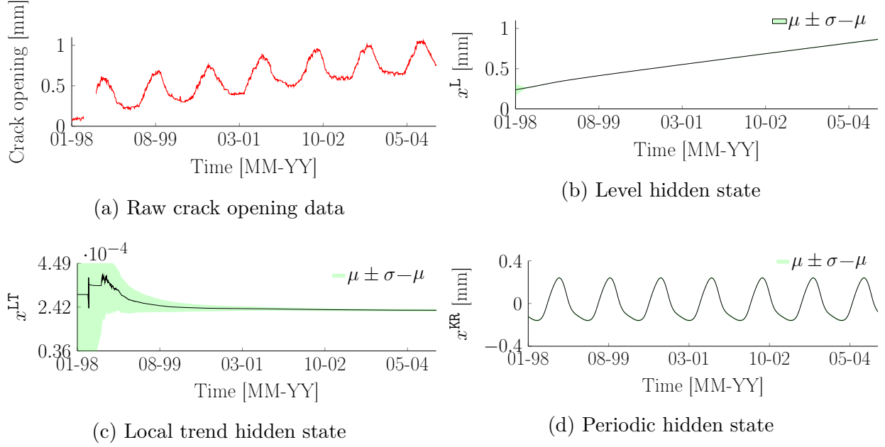
Figure 1.1 Crack opening data from a dam in Canada and unobserved hidden states extracted from the raw data using the BDLM model.
