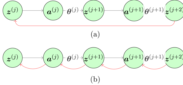
Figure 3.7 Infer the hidden states of a layer j^{th} from the hidden states of layer j + 2^{th} (a) with, and (b) without bypassing the layer j + 1^{th} .
