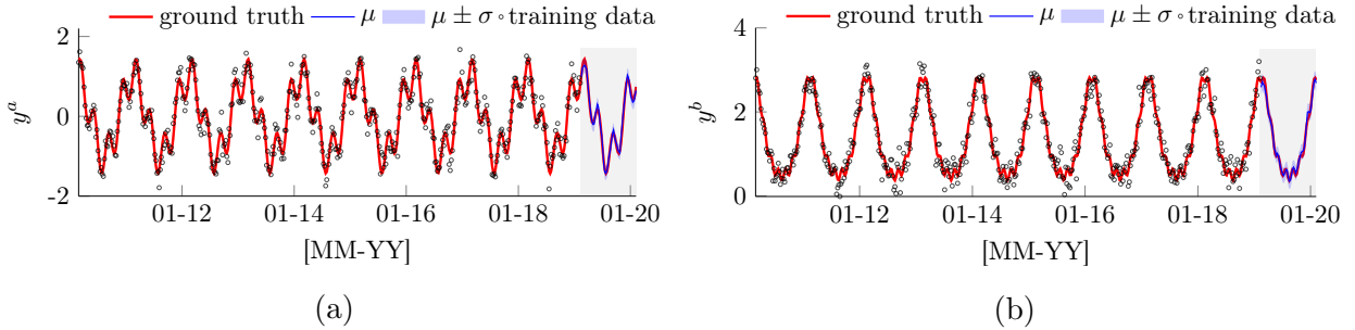
Figure 3.8 Test predictions from TAGI-LSTM models for synthetic data generated using (a) Equation 3.14a, and (b) Equation 3.14b. The grey shaded area presents the forecast period, red line presents the ground truth, blue line presents test predictions along with \pm\sigma confidence intervals (shade), black dots present training data. The \pm\sigma regions contain both the epistemic (parameter’s) uncertainties obtained from the prior predictive distribution of z^{(0)} as well as the aleatory uncertainties associated with the error term’s variance \sigma_V^2 .
