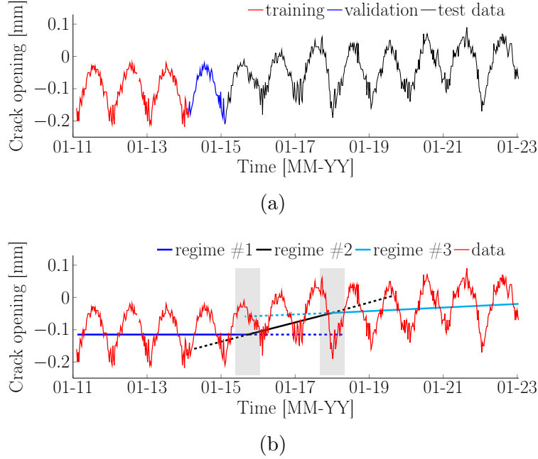
Figure 5.8 Case study #1. (a) Crack opening data from a dam in Canada, and (b) preliminary analysis to identify visually possible anomalies where the grey shaded area presents the regime switch quantitatively. The dash line with a corresponding colour presents the extension for the regime identified.
