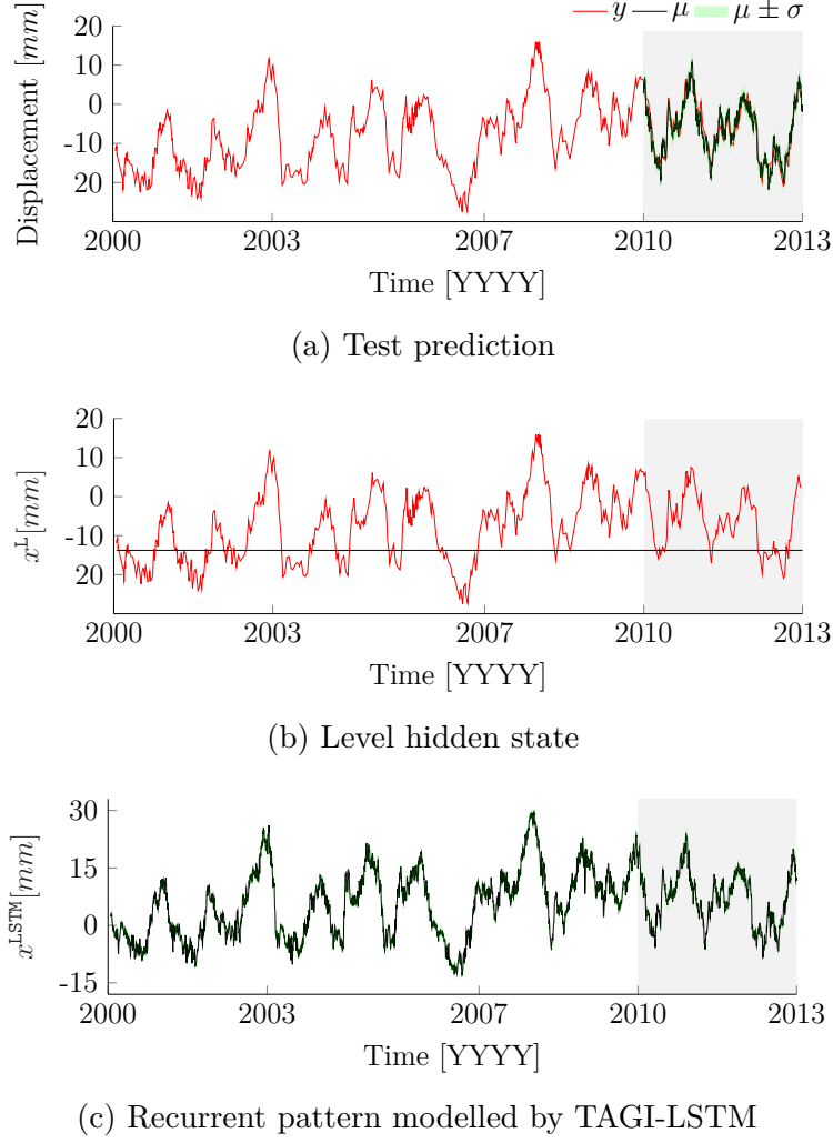
Figure 4.13 Results from our model for the displacement dataset including the test predictions, the level hidden state, and the recurrent pattern. The grey shaded area presents the forecast period. The \pm\sigma regions in (a) contain both the epistemic (parameter's) uncertainties obtained from the prior predictive distributions of the hidden states as well as the aleatory uncertainties associated with the error term's variance \sigma_V^2 .
