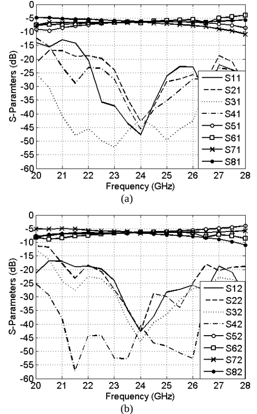
Fig. 11. Simulated results of the 4 × 4 Butler matrix. (a) Signal at port 1.(b) Signal at port 2
