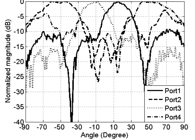
Fig. 14. Measured radiation patterns of the antenna array fed by 4 x 4 Butler matrix at 77GHz
