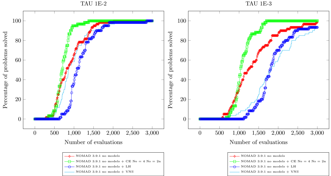
Figure 4.8 Result on the 60 MDO instances between Mads (no models), CE-Mads , VNS-Mads and LH-Mads for \tau = 10^{-2} (left) and \tau = 10^{-3} (right).
