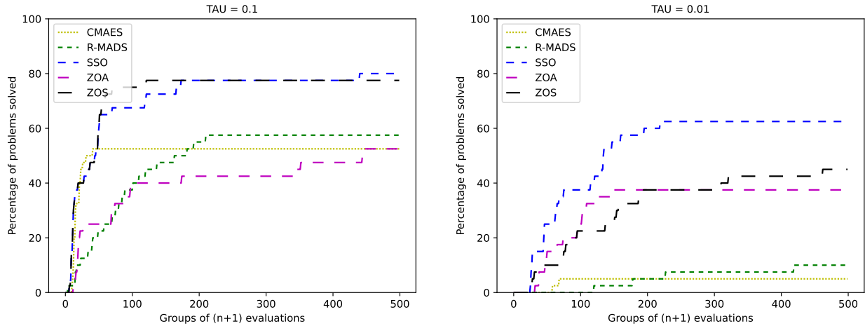
Figure 5.4 Results on test problems with n \geq 10 for \tau = 0.1 (left) and \tau = 0.01 (right) with 5 different seeds for each problem.
