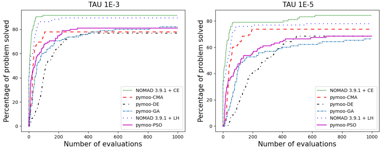
Figure 4.7 Result on the 19 global optimization test problems between CE-Mads, LH-Mads, GA, DE, CMA-ES and PSO for \tau = 10^{-3} (left) and \tau = 10^{-5} (right).
