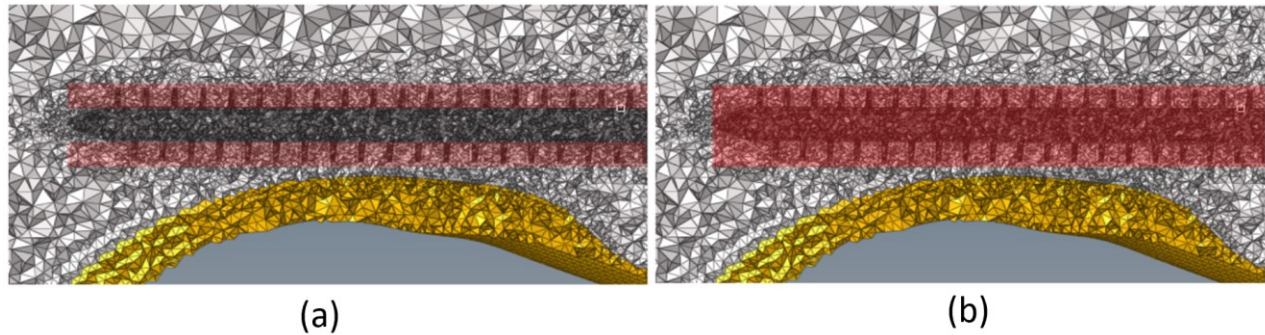
Figure 5.2 Cross-section of (a) a hollow cylinder and (b) a full cylinder that were used to sum the properties in the red region to evaluate the fitness score. The trabecular bone is represented in white and the cortical bone in yellow.
