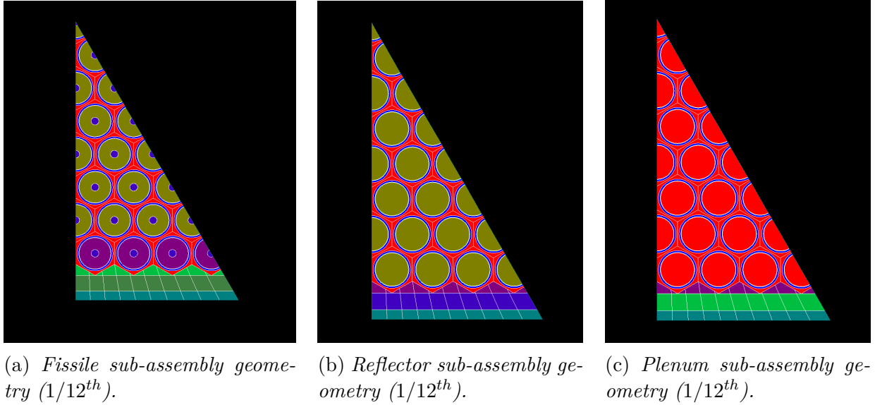
Figure 3.6 INCA generated unstructured geometries for Fissile (a), Reflector (b) and Plenum (c) sub-assemblies. Colors show associated zones, allowing for the assignment of different physical properties.
