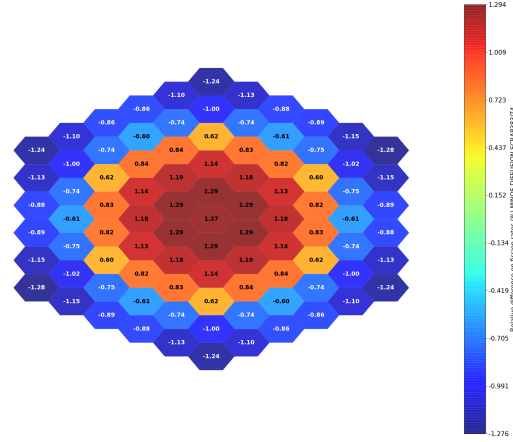
(b) Relative error on fission rates, VOID configuration.
