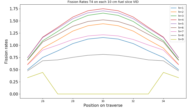
(b) Fission rates at each 10 cm fuel height, VOID configuration.
