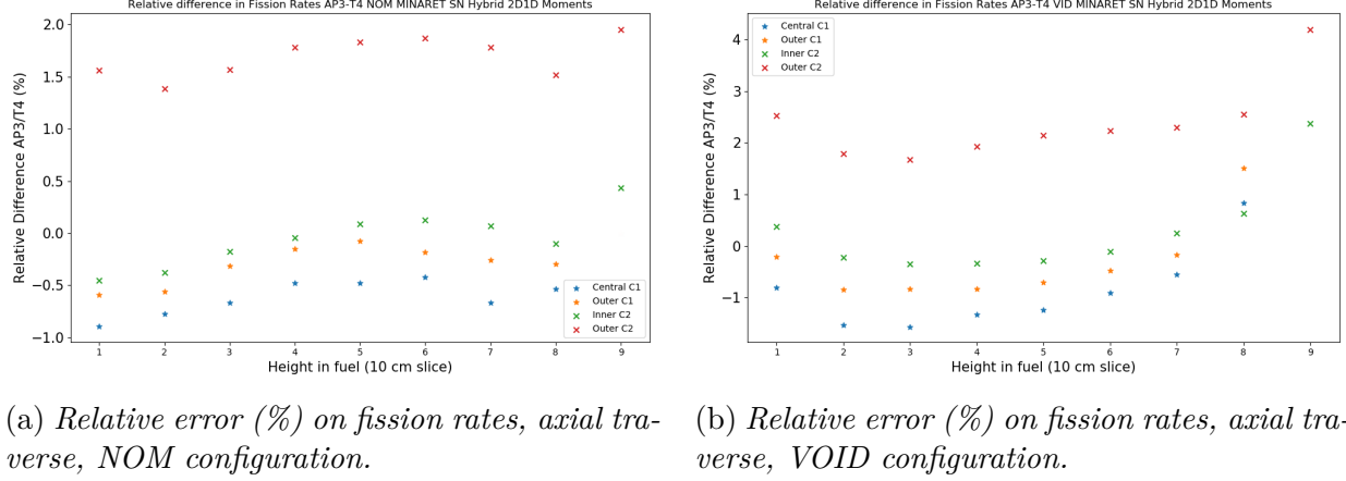
Figure 4.9 Relative error on fission rates on axial traverse, rates integrated over 10cm fuel slices, MINARET with XS from hybrid 2D1D - T4. Axial traverse on central and outer C1 assemblies, inner and outer C2 assemblies.
