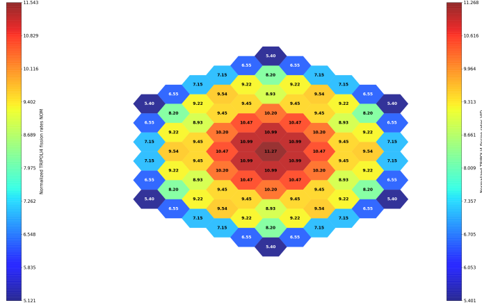
(b) Axially integrated reference fission rates, VOID configuration.
