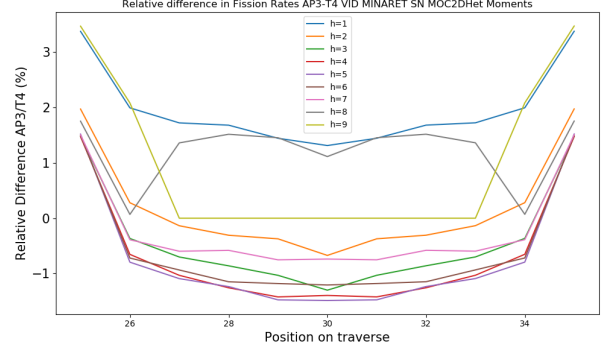
(b) Relative error (%) on fission rates, radial traverse, VOID configuration.
