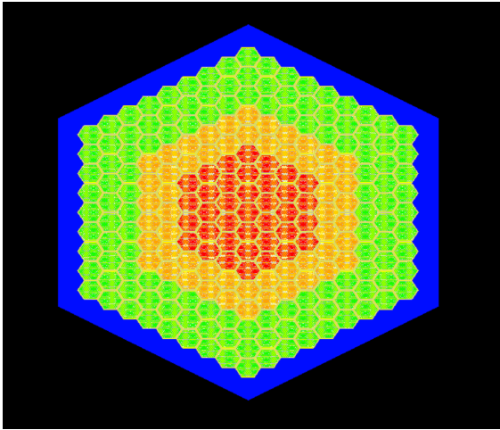
(a) Top view of the ANTOINID core.
