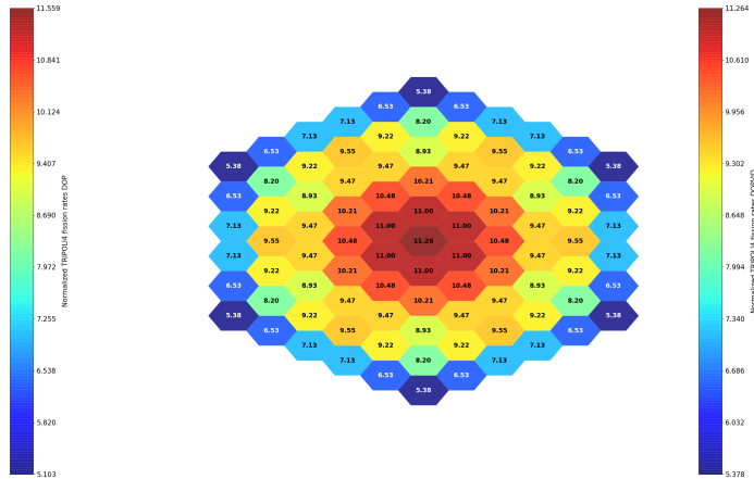
(d) Axially integrated reference T_4 fission rates, DOP+VOID configuration.
