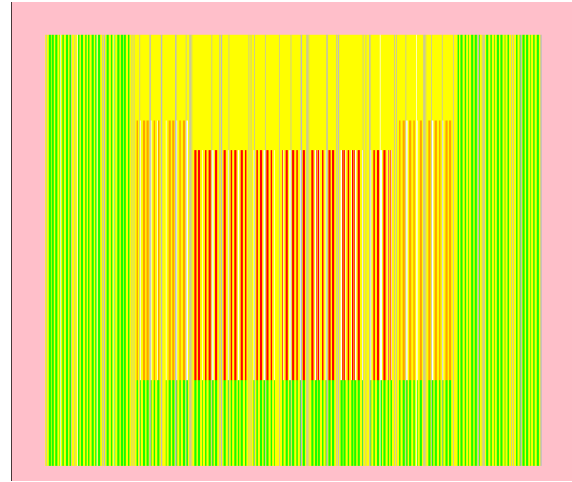
(b) Axial distribution of materials in the core, view on the y=0 axis.
