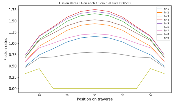
(d) Fission rates at each 10 cm fuel height, DOP+VOID configuration.
