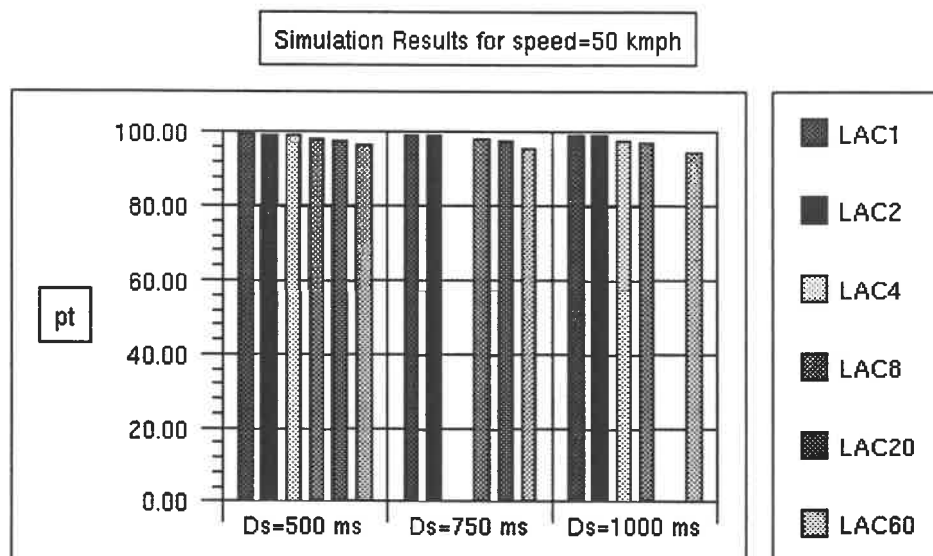
Figure 4.8. p_t Results for \bar{s} = 50 kmph
