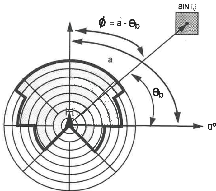
Figure 3.5. Antenna Pattern Loss as a Function of phi
