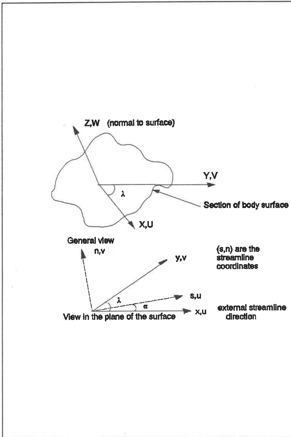
Figure 9 Coordinate System
