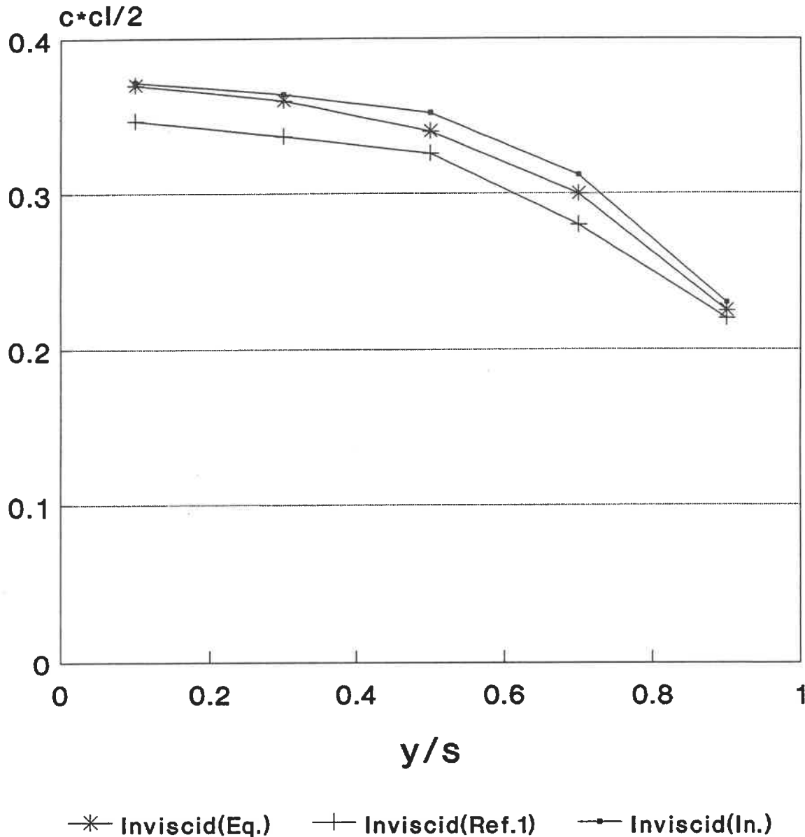
Fig. 16: Comparison of Load Distribution Near Rectangular Wing
