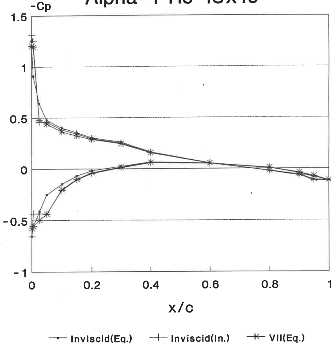
Fig. 19: Comparison of Pressure Distribution Swept Wing: y/s=0.9
