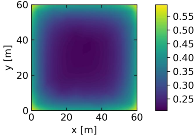
Fig. 3. \rho distribution for an optimized bore field with a penalization of p = 1
