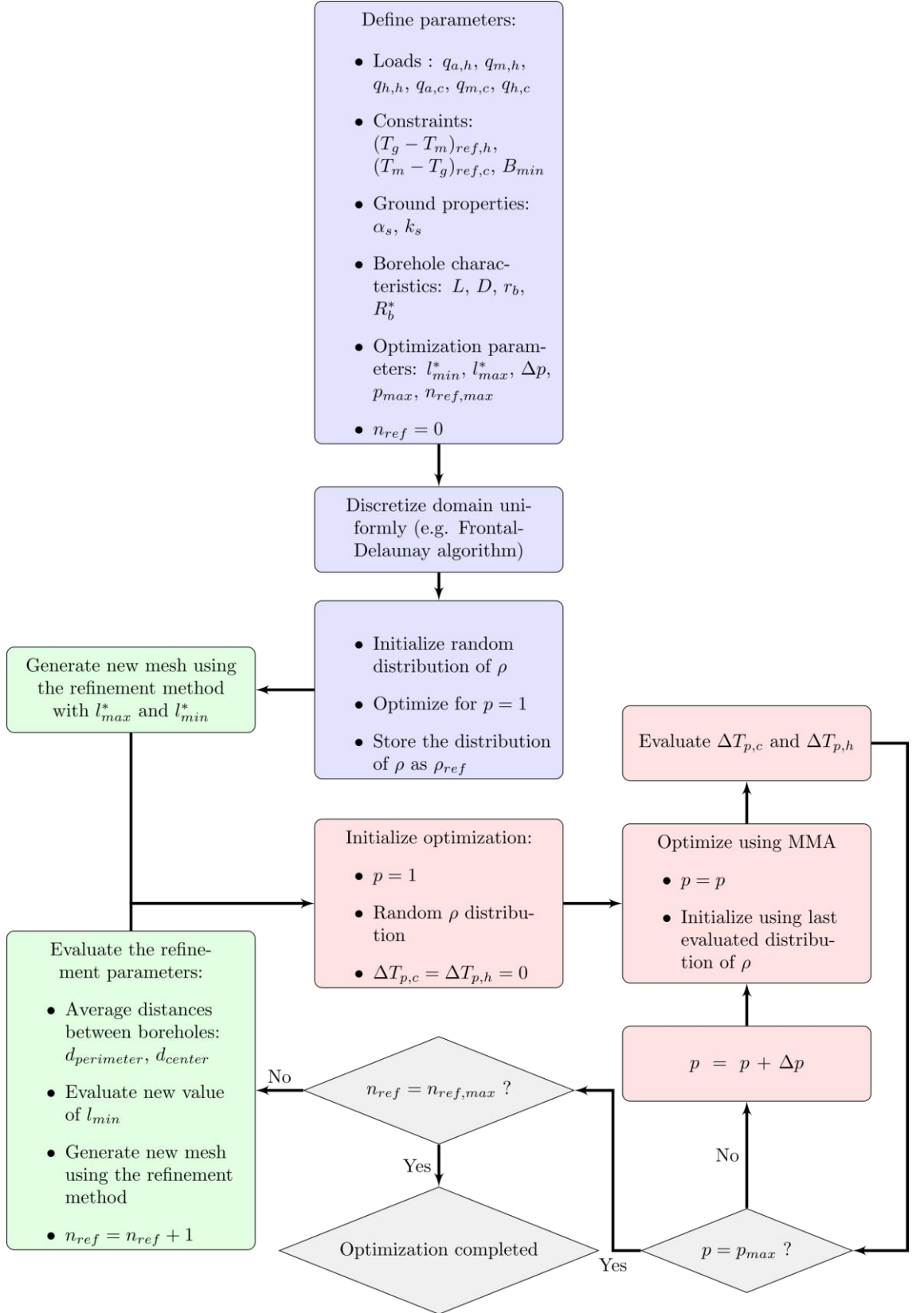
Fig. 2. Bore field optimization procedure
