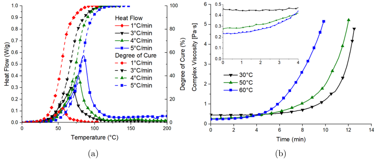
FIGURE 4.2 a) Cure kinetic of the novel polyurethane matrix and b) its rheology behavior
