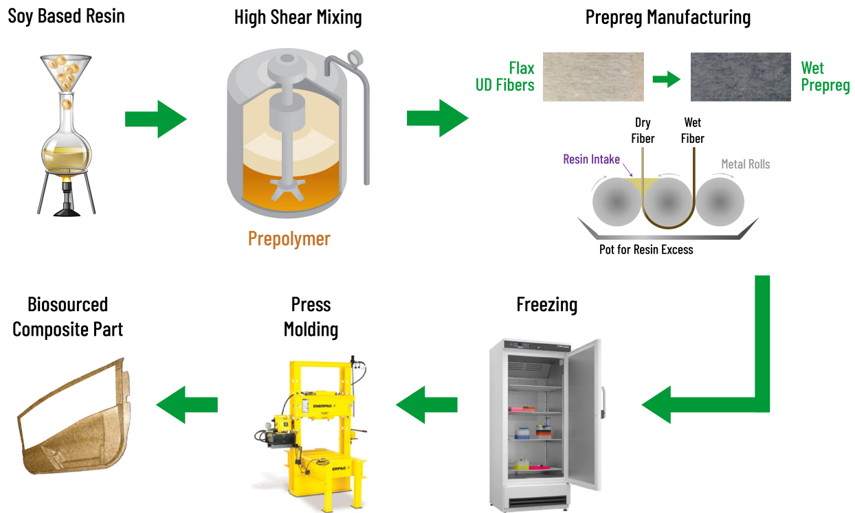
FIGURE 4.4 Processing of the bio-sourced composite material developed in this paper
