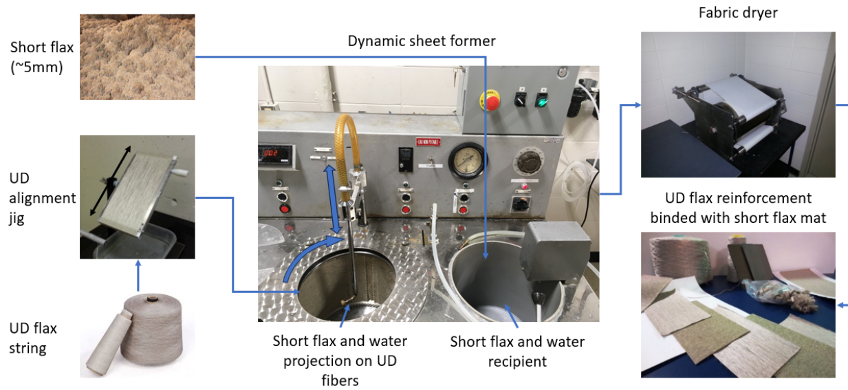
FIGURE 4.3 Manufacturing setup of the UD/mat flax fibers studied in this work [30]
