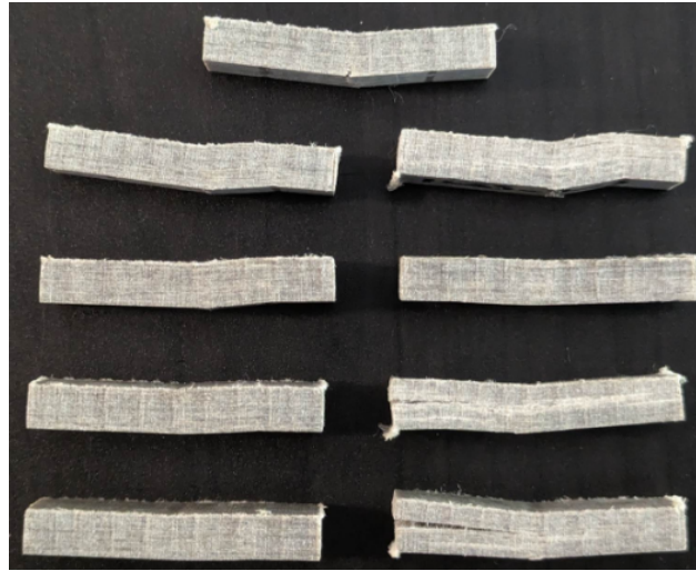
FIGURE 4.11 Short beam shear coupons of flax/PU composites
