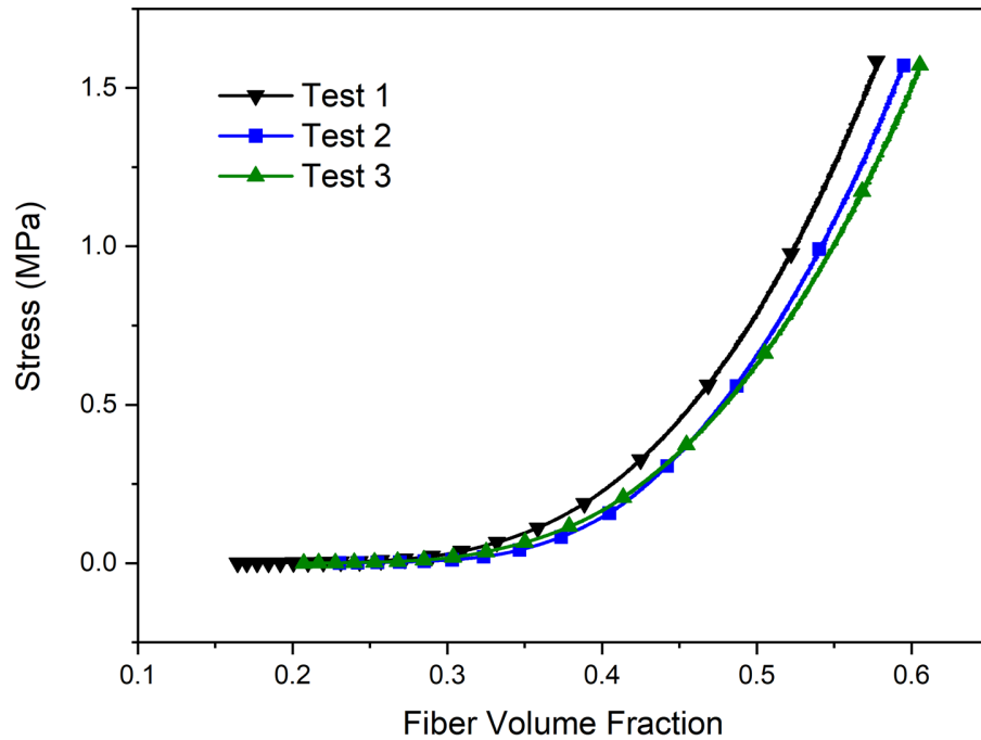
FIGURE 4.5 Compaction tests of the flax fibers studied in this research
