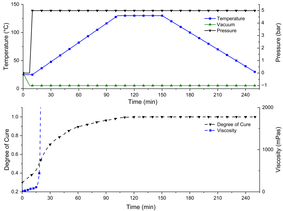
FIGURE 4.6 Temperature and pressure data of the curing cycle used for laminate consolidation. Second chart shows the resulting degree of cure and viscosity
