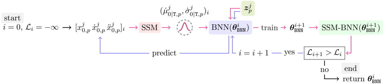
Figure 3.2 The recursive process of estimating the BNN parameters \theta_{\text{BNN}} . At i = 0 , the initial states [x_{0,p}^j, \dot{x}_{0,p}^j, \ddot{x}_{0,p}^j]_i are defined with Equation 3.5 and passed through the SSM to obtain the smoothed initial speeds (\mu_{0|T,p}^j, \sigma_{0|T,p}^j)_i . These are then used to train the BNN, so that it learns to predict them based on the structural attributes \mathbf{z}_p^j . The SSM-BNN model then evaluates the log-likelihood of the validation set \mathcal{L}_{i+1} and compares it to the previous iteration \mathcal{L}_i . If there is an improvement, the BNN uses the structural attributes \mathbf{z}_p^j to define the priors for the initial deterioration speeds \dot{x}_{0,p}^j , and the recursive loop is continued. Otherwise, the loop is terminated and the BNN parameters from the previous iteration \theta_{\text{BNN}}^i are returned. The forward and backward steps of the loop are represented by the magenta and blue arrows.
