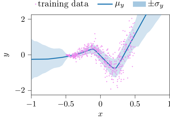
Figure 2.6 Illustration of TAGI’s capacity to learn a mapping to a target variable with heteroscedastic variance. This figure is adapted from [2].
