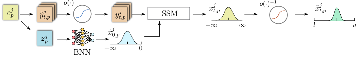
Figure 3.1 Overview of the procedure for estimating the deterioration state of the p -th element from the j -th bridge, denoted by e_p^j , using the proposed SSM-BNN framework. The original visual inspections of the element \tilde{y}_{t,p}^j are first transformed into an unbounded domain using the sigmoid function o(\cdot) , yielding the transformed observations y_{t,p}^j . The BNN then uses the structural attributes of the element z_p^j to define its initial deterioration rate \dot{x}_{0,p}^j . The initial state \mathbf{x}_{0,p}^j and the transformed observations y_{t,p}^j are then passed into SSM to predict the element's deterioration state over time \mathbf{x}_{t,p}^j = [x_{t,p}^j \ \dot{x}_{t,p}^j \ \ddot{x}_{t,p}^j]^\top for t \in \{1, 2, \dots, \tau\} , where \tau denotes the time-horizon of the prediction. These predicted states are finally back-transformed to the original space using o^{-1}(\cdot) , resulting in \tilde{\mathbf{x}}_{t,p}^j = [\tilde{x}_{t,p}^j \ \tilde{\dot{x}}_{t,p}^j \ \tilde{\ddot{x}}_{t,p}^j]^\top .
