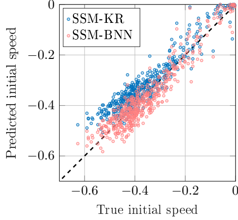
(a) Scatter plot of the true speed \dot{x}_0 versus the predicted speed \dot{\mu}_0 .
