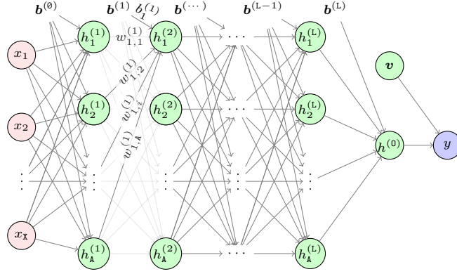
Figure 2.3 Graphical representation of a feedforward neural network consisting of L hidden layers with A hidden units in each one. The network maps the relation between the inputs \mathbf{x} = [x_1 \cdots x_X]^\top and the unit at the output layer h^{(0)} . To simplify visualization, the output is shown here as one-dimensional. The observation y is connected to the output layer unit h^{(0)} and the error term v through the observation model defined in Equation 2.6. The parameters connecting layer j with layer j + 1 consist of a vector of biases \mathbf{b}^{(j)} and a matrix of weights \mathbf{W}^{(j)} , such that w_{m,i}^{(j)} \in \mathbf{W}^{(j)} represents the weight connecting the i -th unit in layer j to the m -th unit in layer j + 1 . This figure is adapted from [1].
