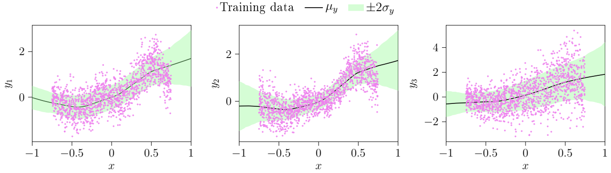
Figure 6.3 Illustration of correlated and highly variable outputs predicted by a Bayesian neural network relying on the proposed inference method.
