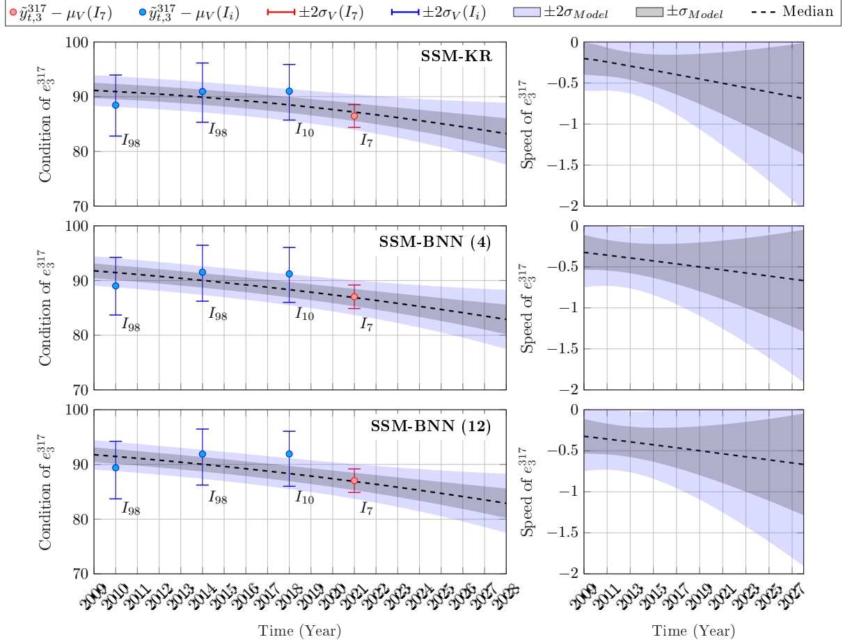
Figure 4.7 The deterioration of element e_3^{317} , as predicted by SSM-KR and SSM-BNN (4) using 4 covariates and SSM-BNN (12) using all 12 covariates. The predicted deterioration is represented by the dashed black lines, with the shaded areas representing the confidence intervals. The observations \hat{y}_{t,3}^{317} corrected by each inspector's estimated bias \mu_V(I_i) are represented by the circles, with the error bars representing each inspector's estimated variance. The inspection shown in red is hidden from the models during training, and is used to gauge their predictive capacity.
