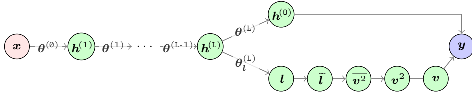
Figure 6.1 Compact representation of the network architecture from Figure 2.3 with modifications to enable inference of the full error covariance matrix. The neural network's parameters connecting layer j to layer j + 1 are denoted by \theta^{(j)} . This figure is adapted from [2].
