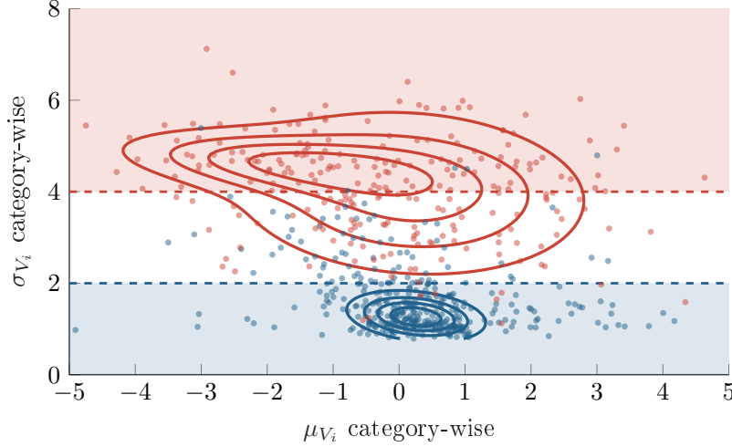
Figure 5.4 Illustration of the variability between inspectors' parameters estimated by the category-wise framework. The scatter points correspond to the inspectors' parameters estimated with the category-wise framework using five structural categories. The blue points are associated with the accurate inspectors ( \sigma_{V_i}^{joint} < 2 ), whereas the red ones correspond to the inspectors with larger uncertainty ( \sigma_{V_i}^{joint} > 4 ). These thresholds are established based on the inspectors' parameters estimated with the joint framework. The contours represent the estimated density of the scatter points.
