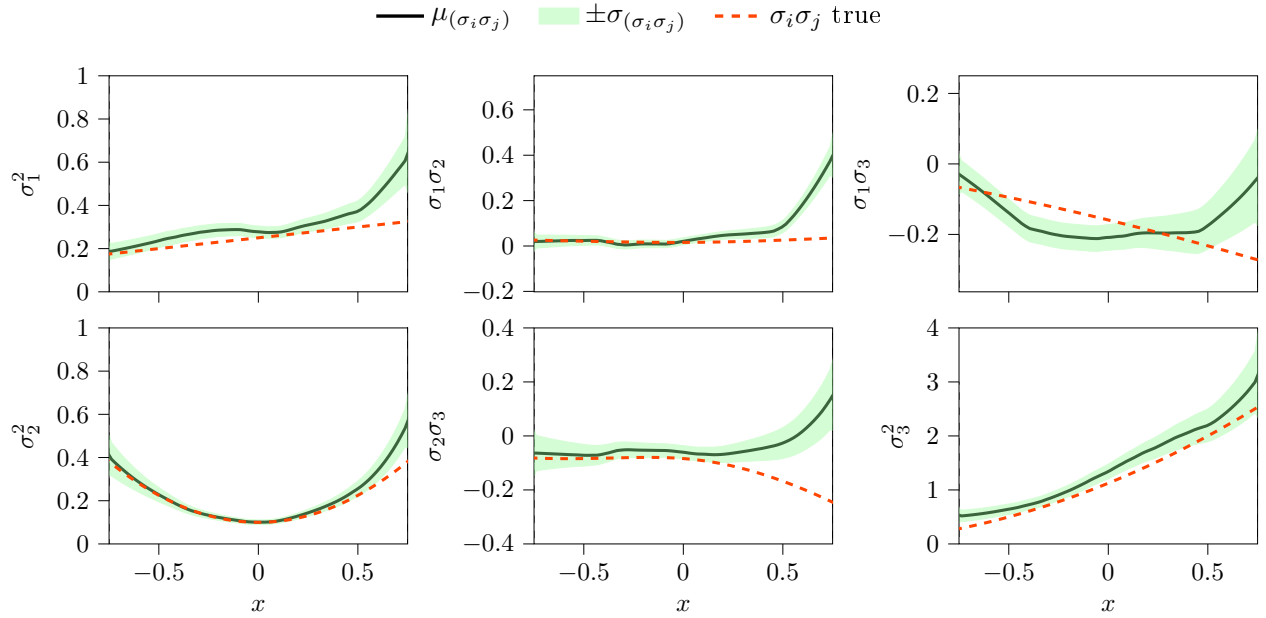
Figure 6.4 Graphical visualization of the full observation error covariance matrix. The true relations are shown by the dashed red lines, while those inferred by the Bayesian neural network are shown by the solid black lines with the shaded regions representing uncertainty.
