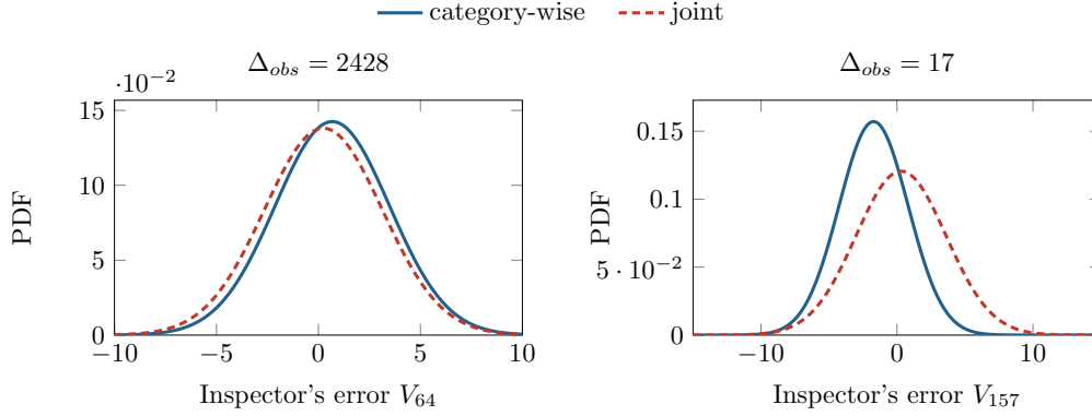
Figure 5.3 Illustration of the observation errors distributions estimated by the category-wise and joint frameworks for inspectors I_{64} and I_{157} . The number of observations for I_{64} increased by 2428, whereas inspector I_{157} only had an increase of 17.
