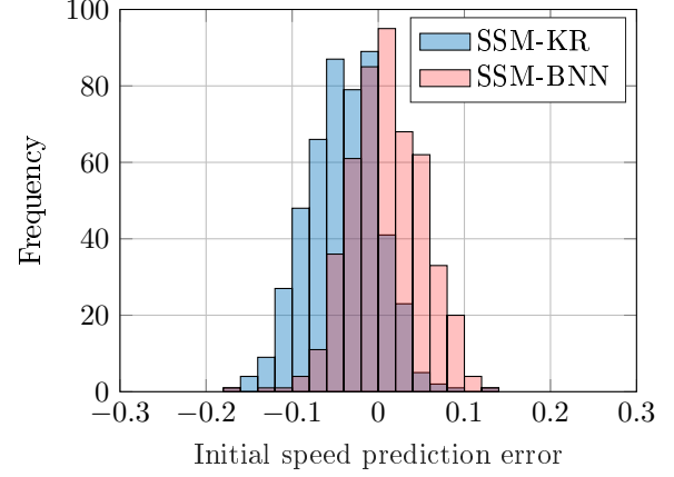
(b) Histogram of the difference between the true speed \dot{x}_0 and the predicted speed \dot{\mu}_0 .
