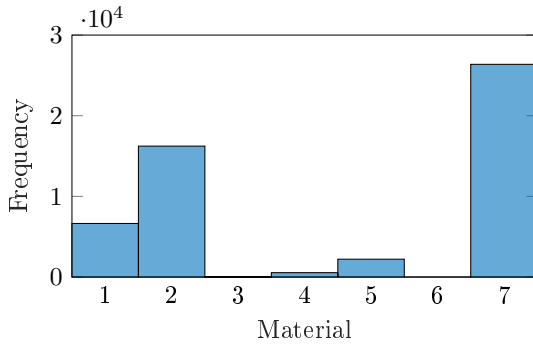
(c) Histogram of materials: 1 \equiv weathering steel, 2 \equiv regular steel, 3 \equiv aluminum, 4 \equiv wood, 5 \equiv high-performance concrete, 6 \equiv prestressed concrete, 7 \equiv regular concrete.
