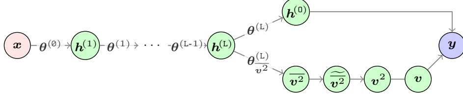
Figure 2.5 Compact representation of the network architecture from Figure 2.3 coupled with the DAG from Figure 2.4. The network parameters connecting layer j to layer j + 1 are denoted as \theta^{(j)} . This figure is adapted from [2].
