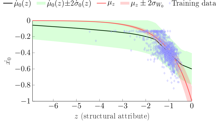
Figure 4.2 The latent relation between the synthetic structural attribute z and the deterioration speed \dot{x}_0 learned by the BNN. The black line represents the expected values predicted by the BNN with the shaded green area representing uncertainty. The true relation is depicted by the red line with the shaded red area representing its variability. Having this variability makes the synthetic attributes resemble reality, where structures with different attributes can deteriorate at the same speed.
