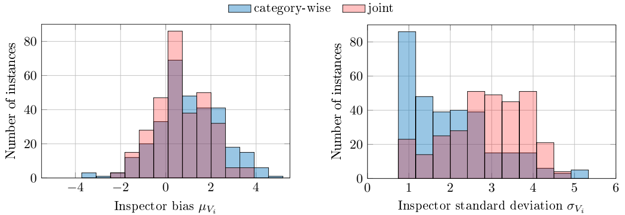
Figure 5.1 Histograms of the inspector parameters obtained using just the beam elements (category-wise) versus using all the element categories (joint).
