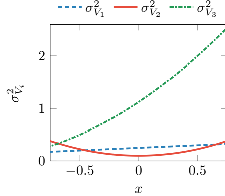
Figure 6.2 Illustration of the heteroscedastic nature of the variance functions used.
