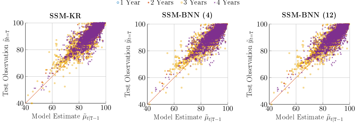
Figure 4.8 Scatter plots of the test observations \tilde{y}_{t=T} versus the model predictions \tilde{\mu}_{t|T-1} for \approx 11000 beam elements. The predictions are obtained by SSM-KR and SSM-BNN using 4 covariates and SSM-BNN using all 12 covariates. Different markers correspond to different forecast durations since the inspection frequency is not uniform among different bridges.
