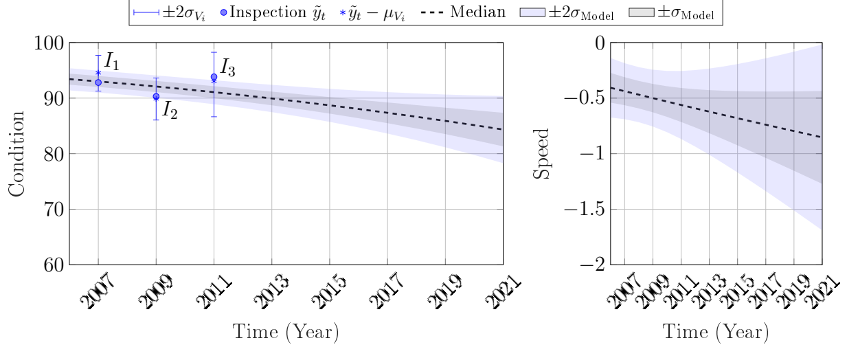
Figure 2.2 Example time series depicting structural deterioration modeled by the SSM.
