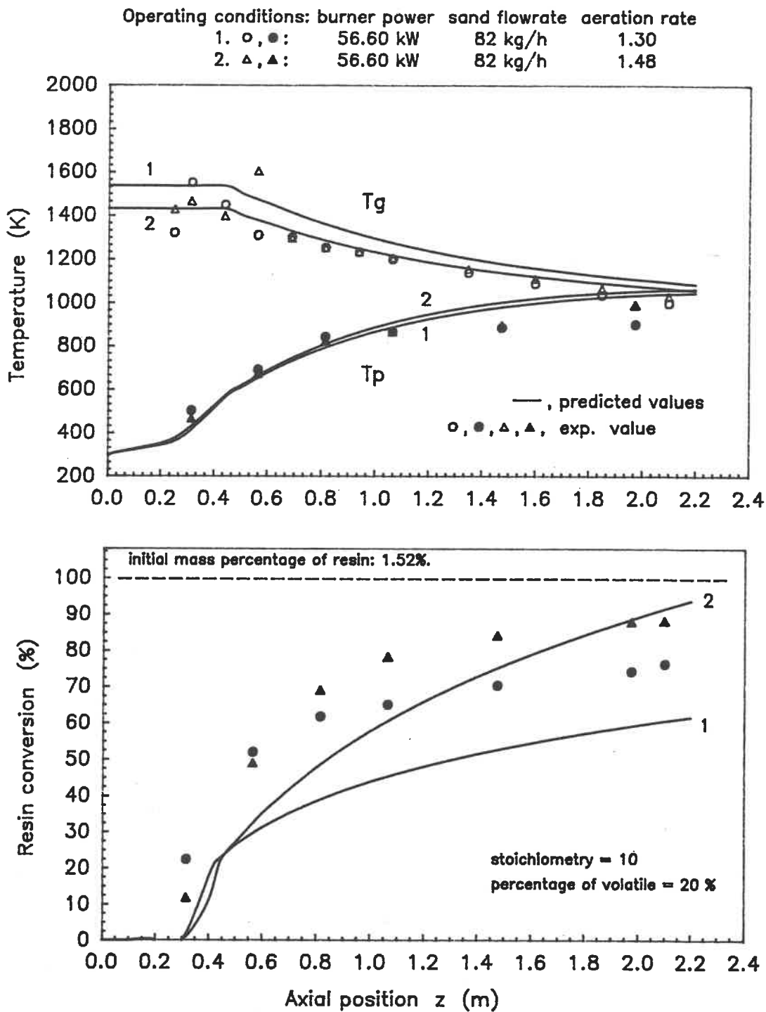
Figure (6-22) Modeling of aeration rate effect for used sand
