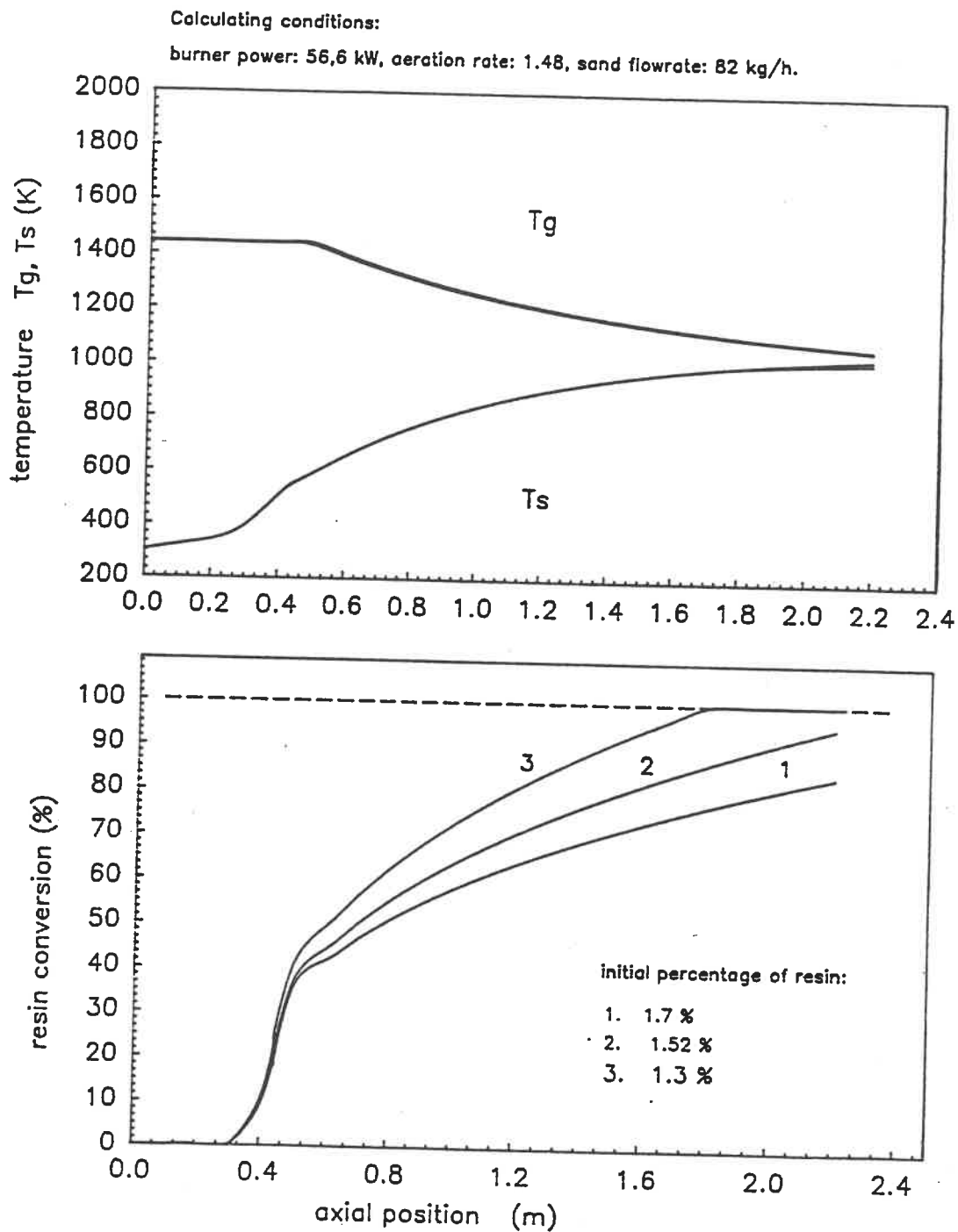
Figure (4-5). Effect of resin content in one model
