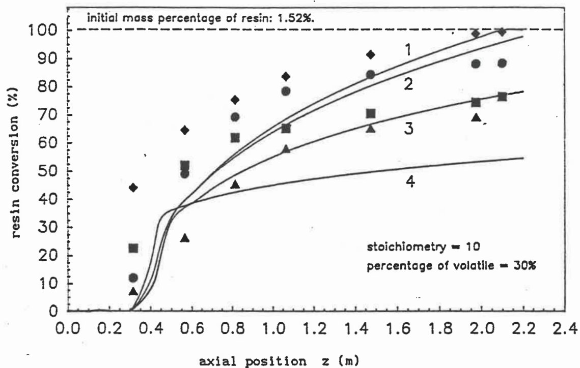
Figure (6-18) Resin conversion (stoichiometry = 10)
