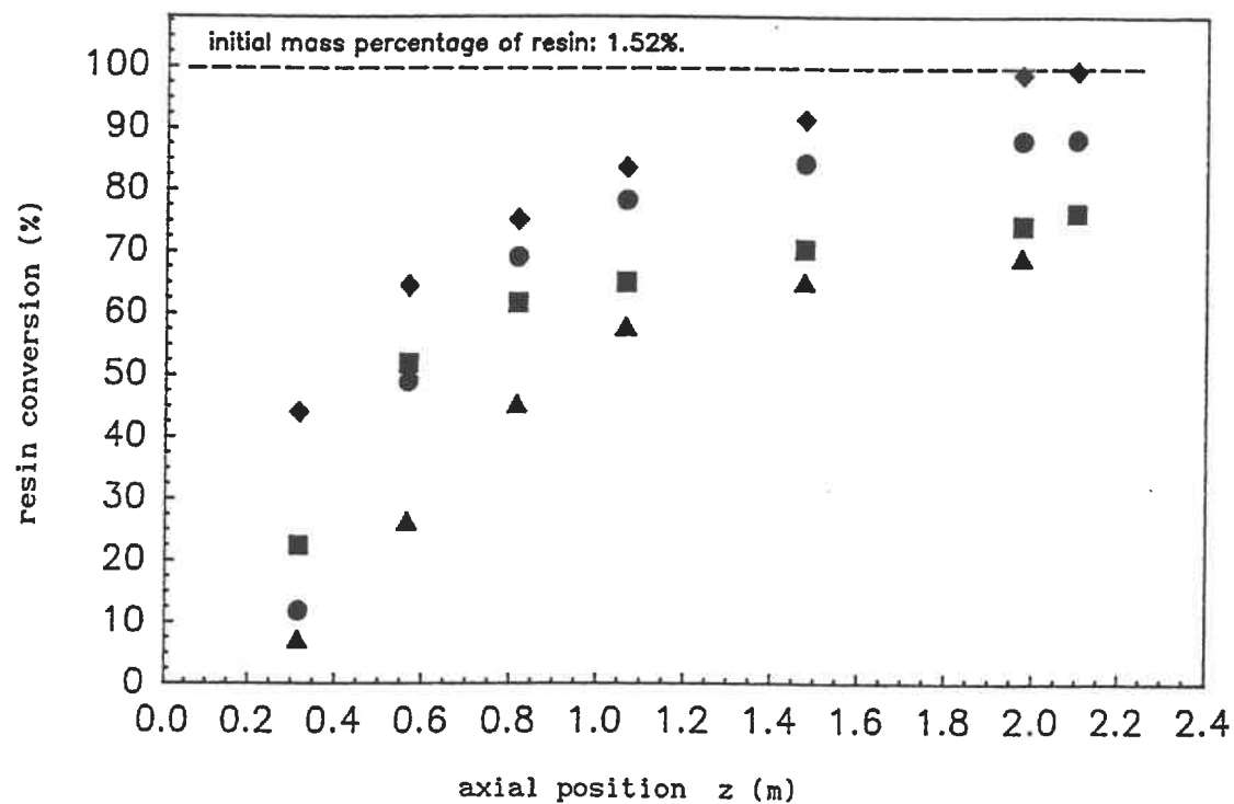
Figure (6-7) Conversion of resin under different operating conditions
