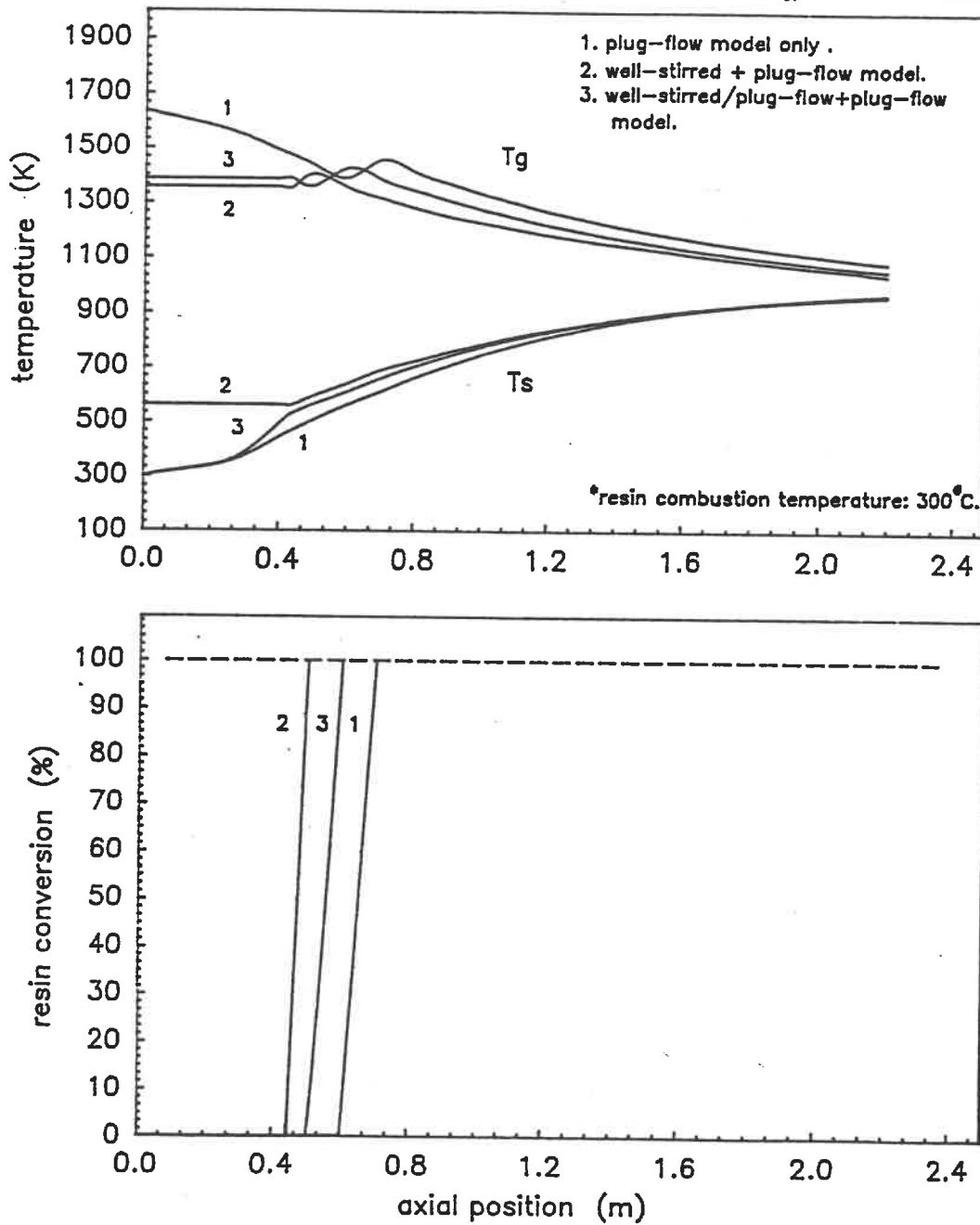
Figure (4-3). Comparison of flow regime models (heat transfer limitation)
