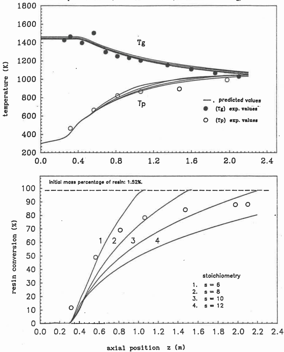
Figure (6-14) Effect of stoichiometry (volatile = 15%)
