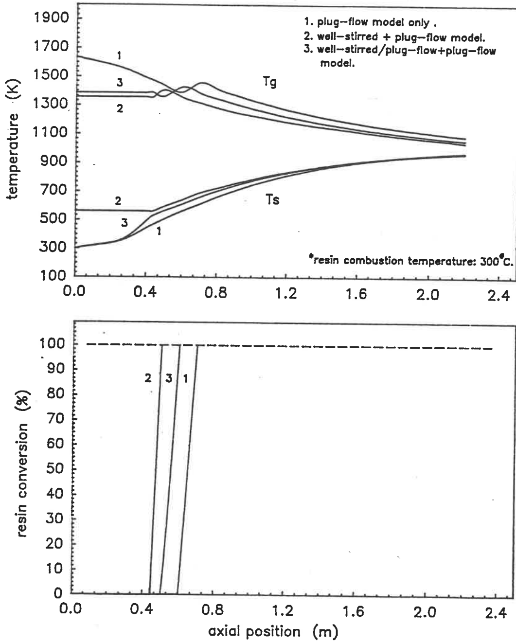
Figure (4-3). Comparison of flow regim models (heat transfer limitation)
