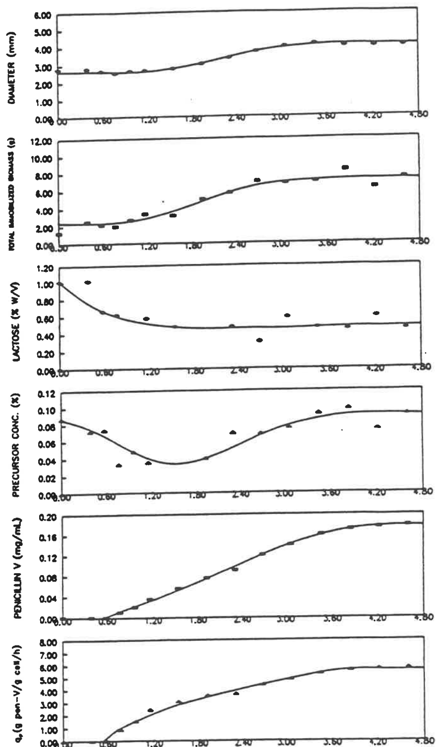
Figure 33: Bioparticle diameter, biomass production, lactose consumption, phenoxyacetic acid consumption, penicillin V production and specific productivity at different t/\text{residence}
