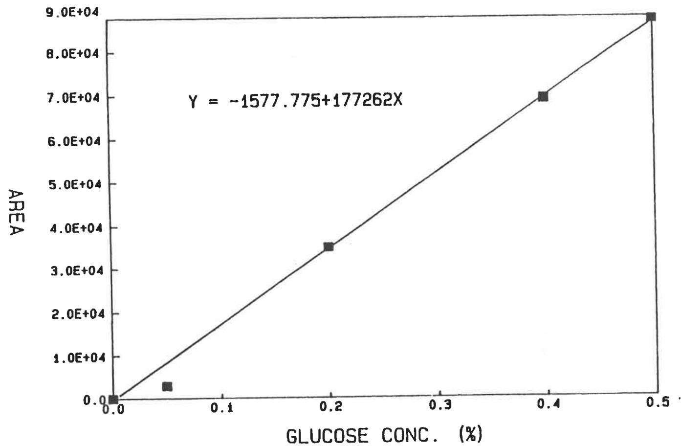
Figure A.3: Glucose standard curve
