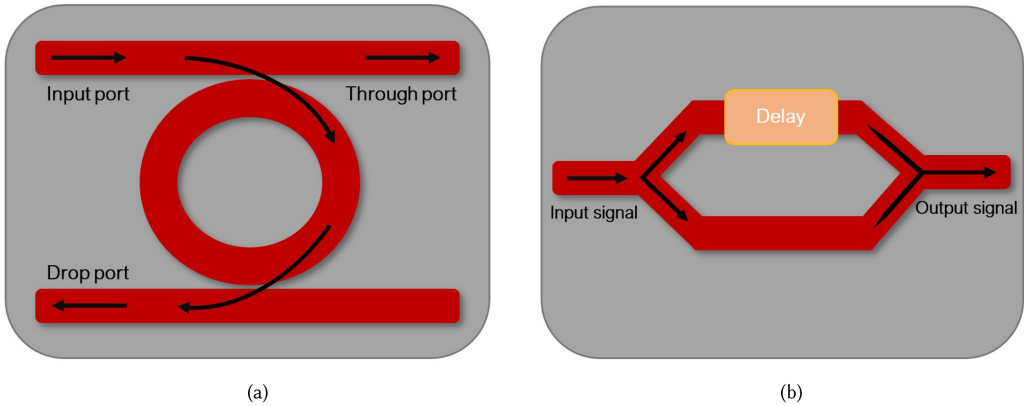
Fig. 2. Schematics of the structure of a MRR (a) and a MZI (b).
