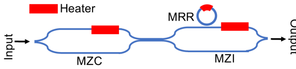
Fig. 6. Schematic of the device under test. Reprinted with permission from Reference [59] (2023 The Optical Society).
