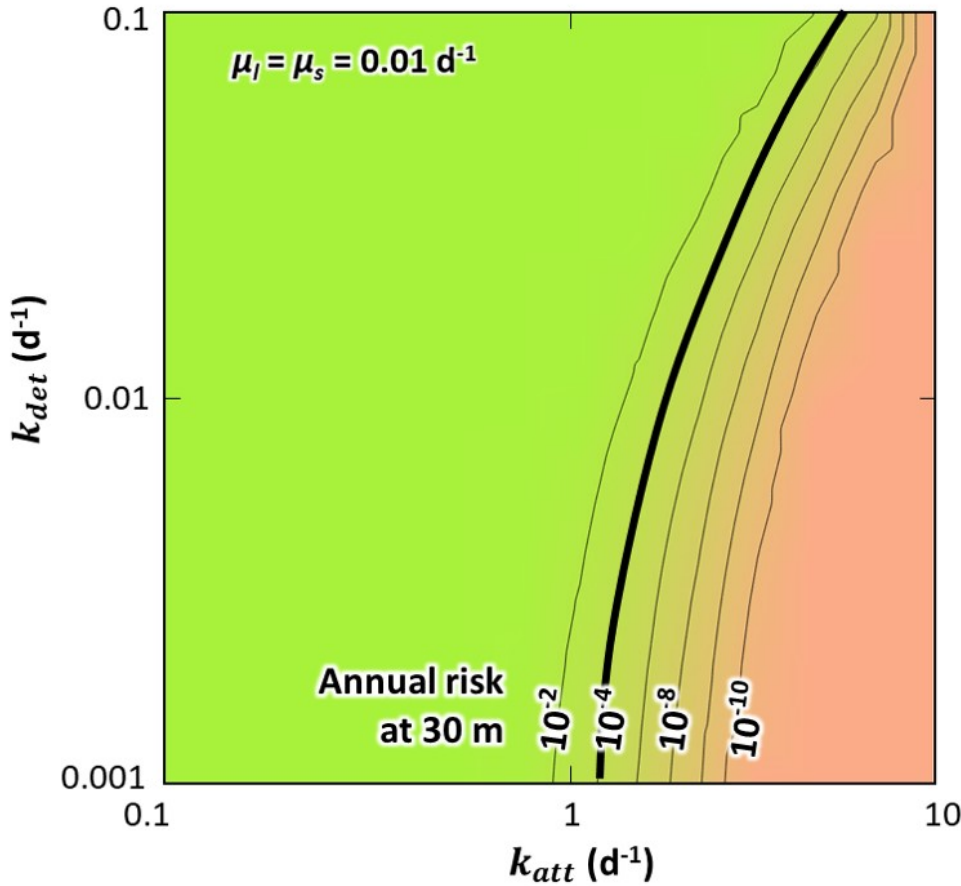
Figure 12. Sensitivity of annual health risk at a 30 m setback distance to attachment and detachment coefficient input parameters. The simulation parameters are v_D = 0.1 m/d , \alpha = 2 m , and \theta = 0.3 .
