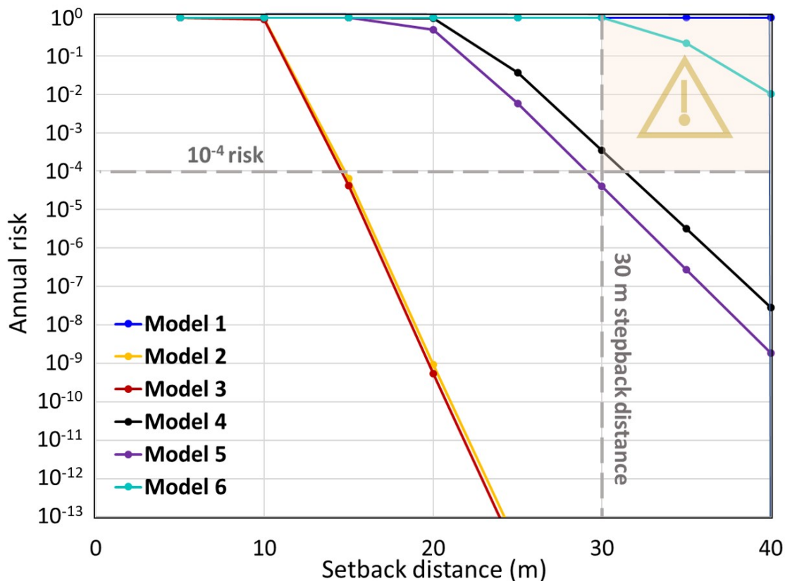
625 Figure 11. Simulation results for annual health risk predictions as a function of setback distances 626 for selected values of kinetic reaction coefficients (see Table 1). The simulation parameters are 627 v_D = 0.1 \text{ m/j} , \alpha = 2 \text{ m} , and \theta = 0.3 . The shaded zone with a warning symbol corresponds to a health 628 risk exceeding the 10^{-4} threshold of the regulatory setback distances, i.e., the danger zone.
