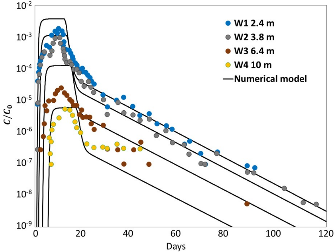
Figure 5. Comparison of modeled and measured MS2 breakthrough curves of field test experiment (Schijven et al., 1999). The simulation parameters are v_D = 0.5 m/d, \alpha = 0.01 m, \theta = 0.35 , K_{att} = 1.26 /d, K_{det} = 0.0008 /d, \mu_l = 0.03 /d, and \mu_s = 0.09 /d.
