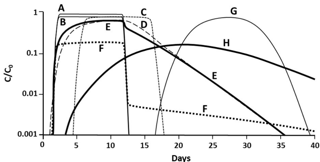
328 Figure 2. Theoretical breakthrough curves predicted for transport models involving various mass 329 transfer mechanisms: A) tracer (nonreactive, purely advective – dispersive transport); B) same 330 model but with first-order degradation; C) equilibrium sorption reactive transport (valid for solutes); 331 D) and G), model C with a high dispersion or a high retarding factor, respectively; E), F), and H), 332 two-site kinetic reactive transport models, valid for organic compounds (e.g., pesticides and 333 pharmaceutical products), with low detachment, high detachment, and high attachment, 334 respectively. Pulses are injected over ten days, 3 m upstream, at 1.5 m/d pore velocity. Modified 335 from Schijven et al. (1999).
