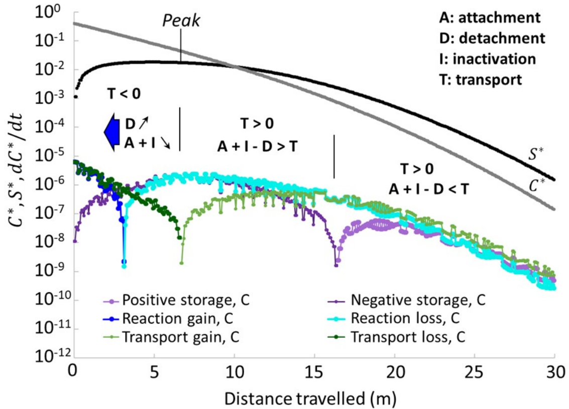
565 Figure 10. Mass transfer budget decomposition along the longitudinal profile after 25 days (same 566 model as shown in Fig. 9). Transport mass changes (T) are by advection and dispersion. Only the 567 inactivation of mobile viruses (I) is considered. The storage gain or loss corresponds to the balance 568 of transport and reactions ( T - [A + I - D] ). C^* (gray line) and S^* (black line) are respectively mobile 569 and immobile virus concentrations normalized to the source concentration ( C_0 ). Mass transfers are 570 in d^{-1} .
