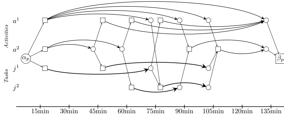
FIGURE 8.1 – Example of a cleaned network
