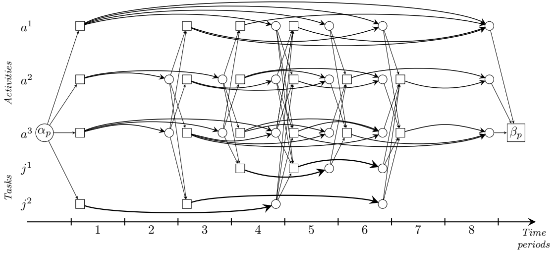
FIGURE 7.3 – Example of a network for activity assignment with time flexibility
