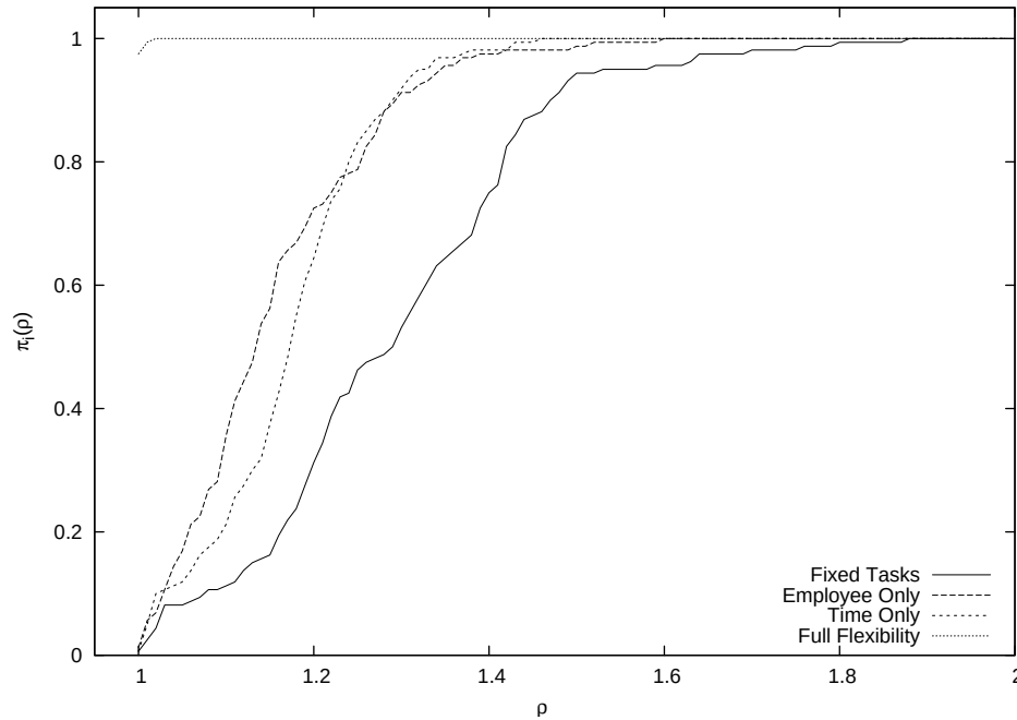
FIGURE 7.5 – Profile curves comparing the solution values obtained for the various strategies
