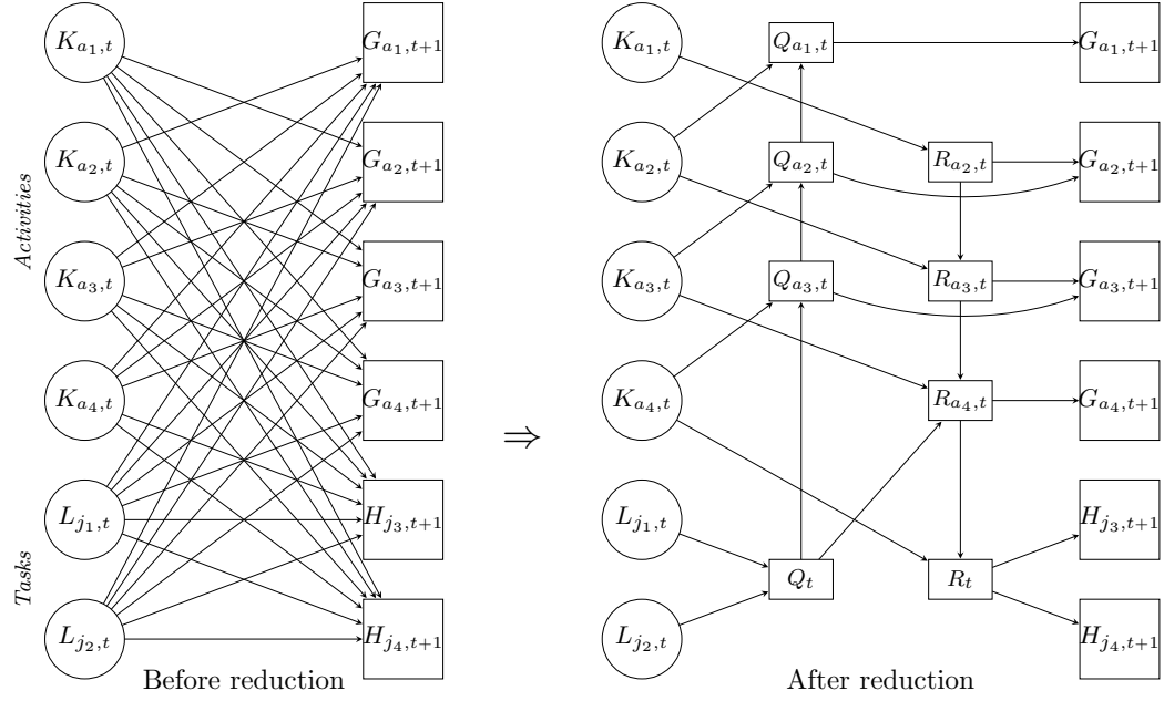
FIGURE 7.4 – Arc reduction in a piece subnetwork with four activities and four tasks
