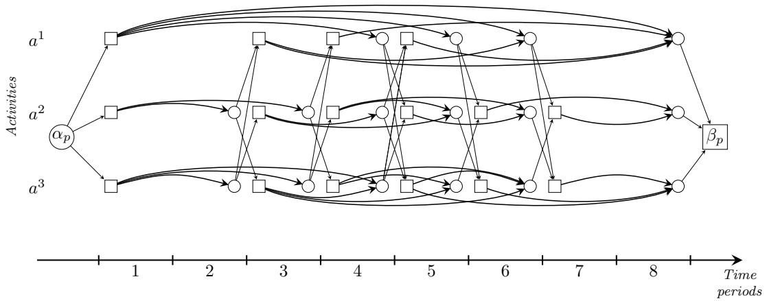
FIGURE 7.1 – Example of a network for activity assignment without tasks
