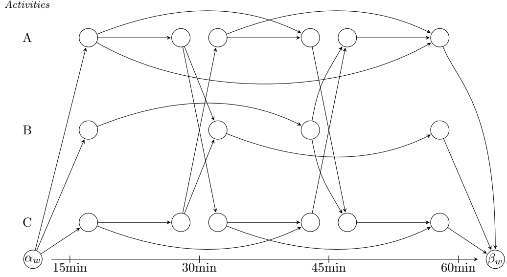
FIGURE 6.1 – Example of a network for a piece of work w \in W
