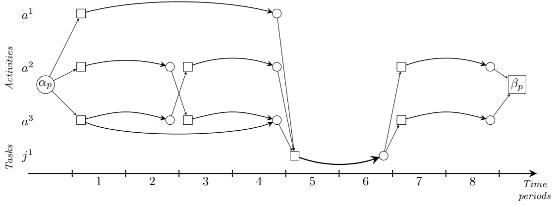
FIGURE 7.2 – Example of a network for activity assignment with fixed tasks
