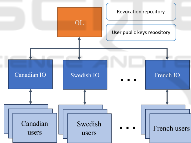
Figure 2: Overall architecture of the solution.
